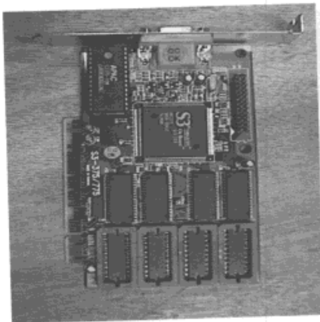
Photo 9 - Video Card - Component side
