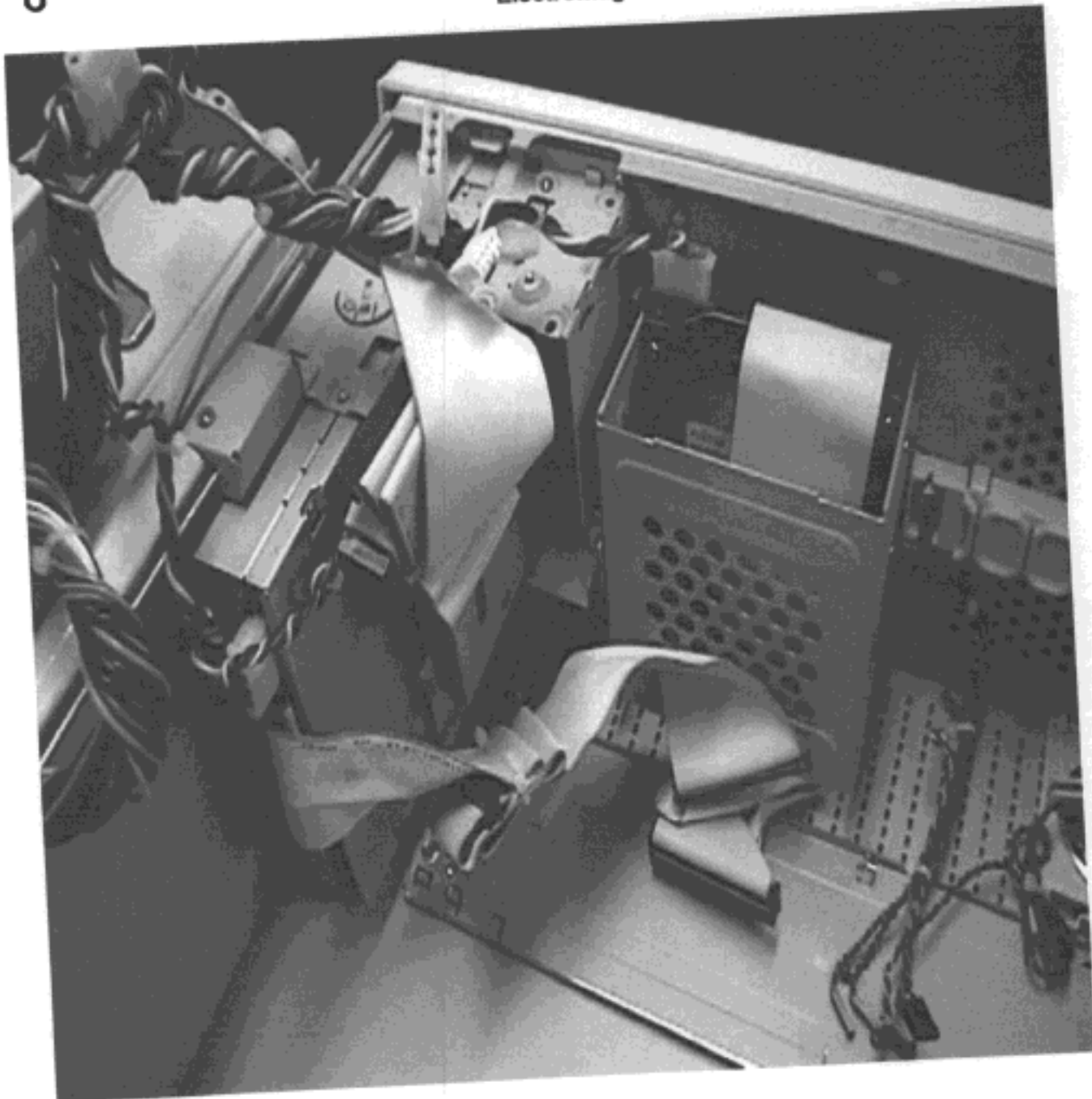
Photo 8 - Detail of Power Supply and power supply cables routing
