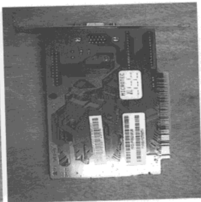
Photo 10 - Video Card - Solder side
