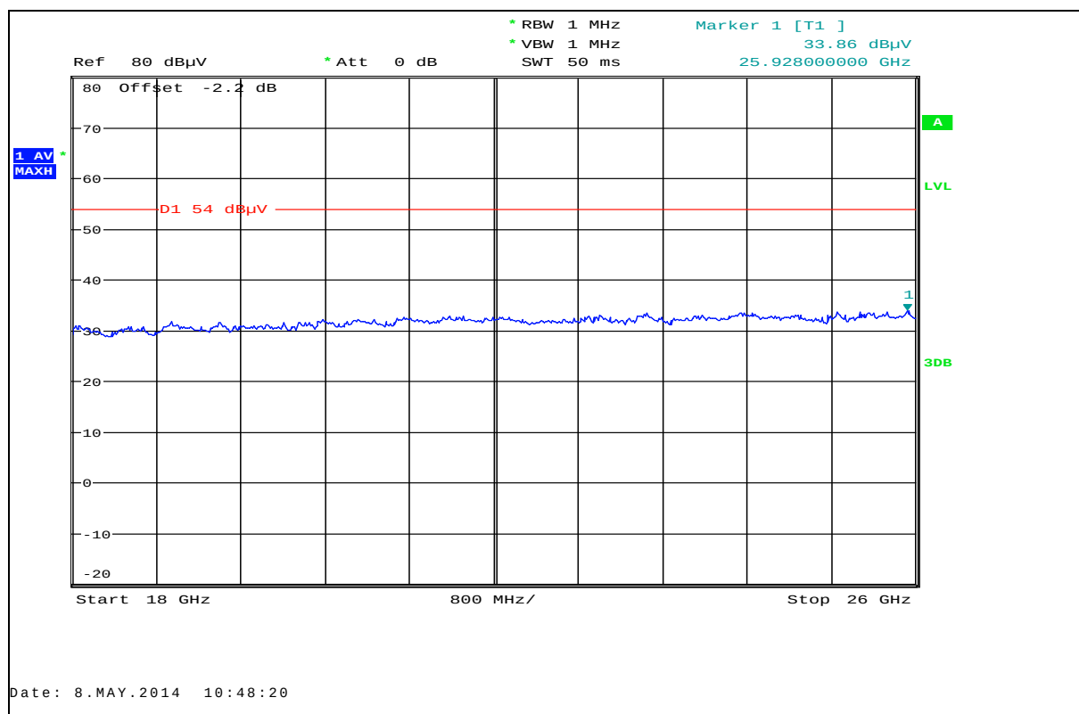
Plot 36: 18 GHz – 26 GHz, antenna horizontal / vertical, low / mid / high frequency
