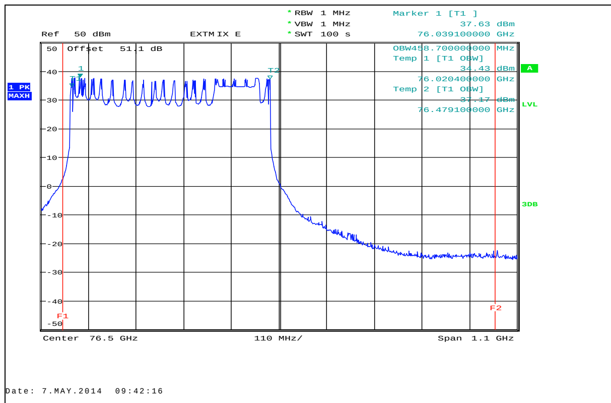
Plot 25: Occupied bandwidth (99%), T_{nom} / V_{nom} , high frequency
