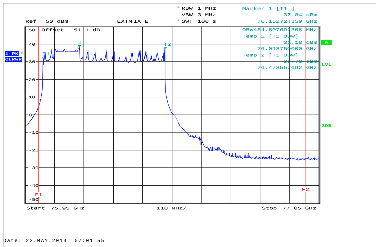
Plot 20: Occupied bandwidth (99%), T_{min} / V_{min} - V_{max} , low frequency
