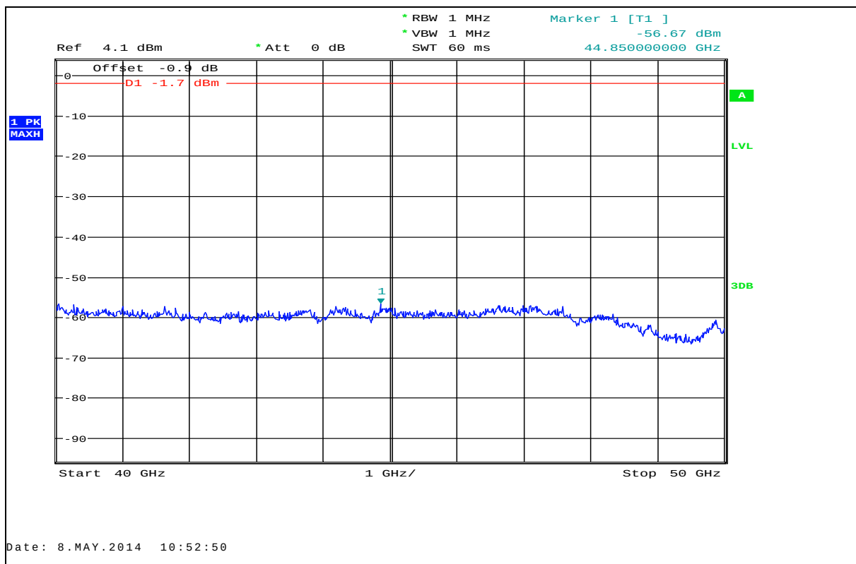
Plot 38: 40 GHz – 50 GHz, antenna horizontal / vertical, low / mid / high frequency
