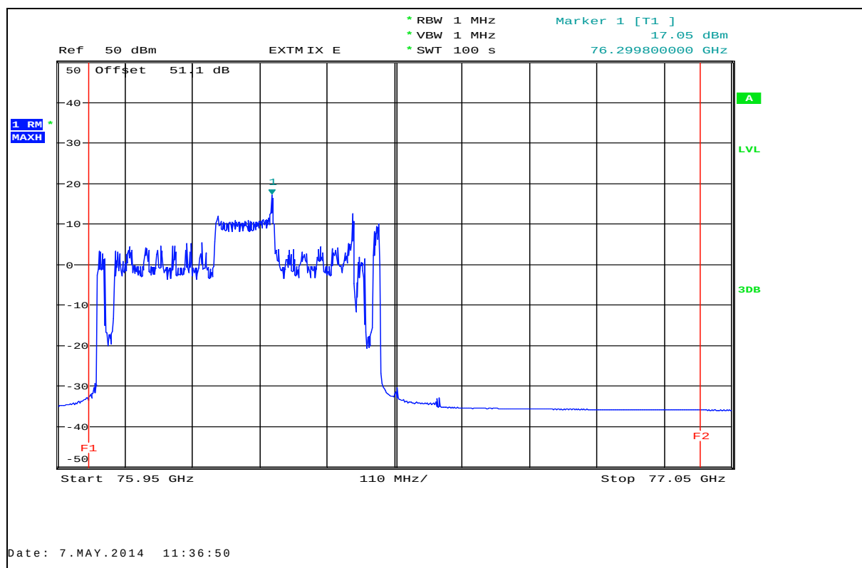
Plot 10: EIRP (RMS detector), T_{\min} / V_{\min} - V_{\max} , mid frequency
