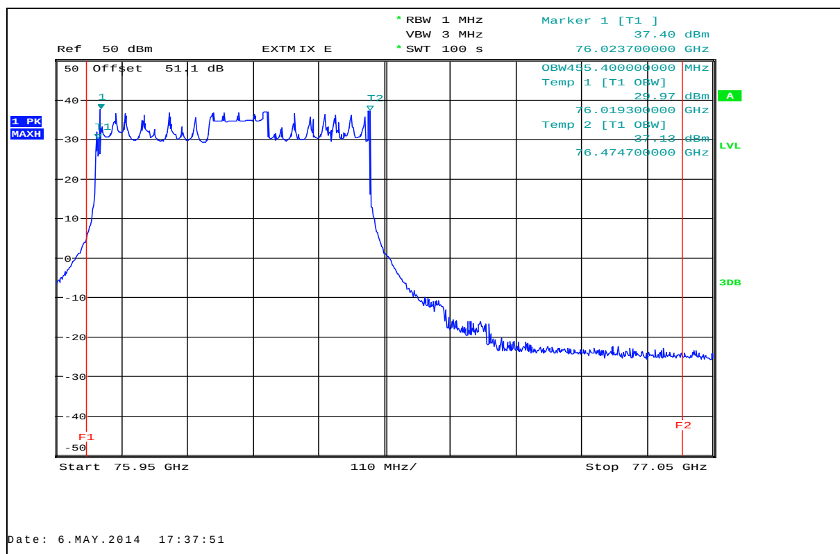
Plot 22: Occupied bandwidth (99%), T_{\text{nom}} / V_{\text{nom}} , mid frequency
