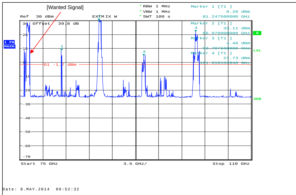
Plot 40: 75 GHz – 110 GHz, antenna horizontal / vertical, low / mid / high frequency
