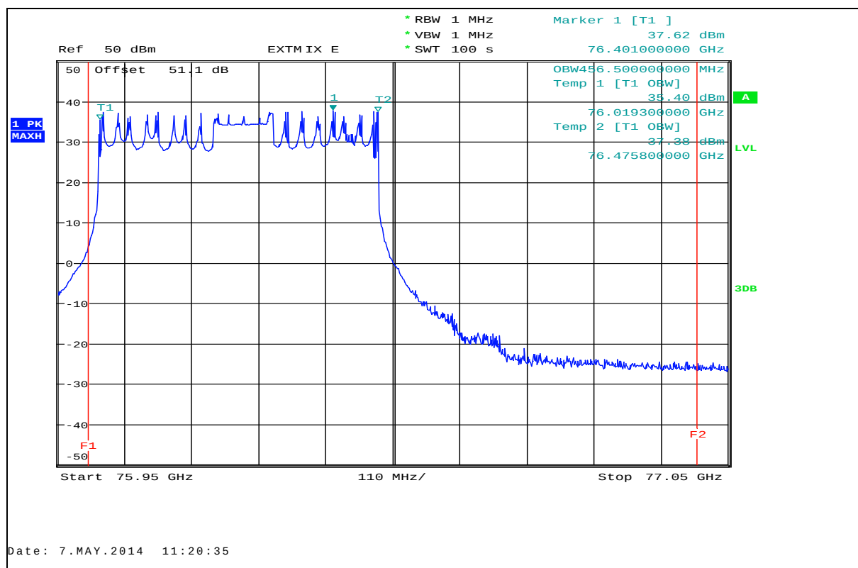
Plot 23: Occupied bandwidth (99%), T_{\min} / V_{\min} - V_{\max} , mid frequency
