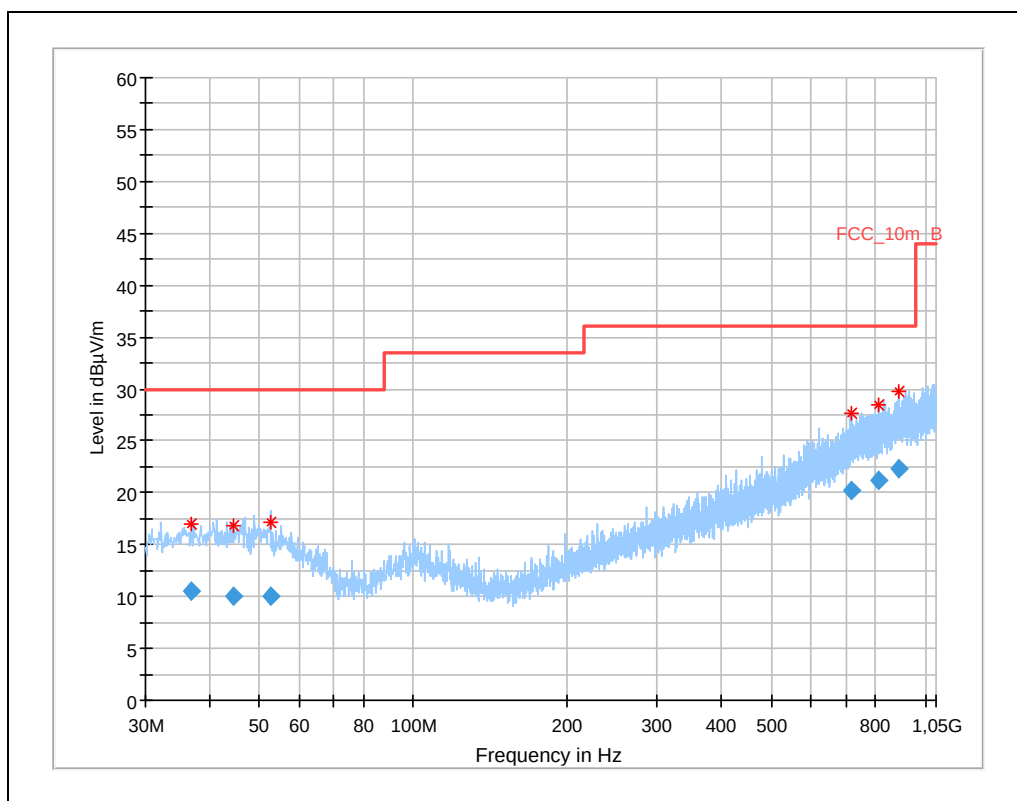
Plot 30: 30 MHz – 1 GHz, antenna horizontal / vertical, mid frequency
