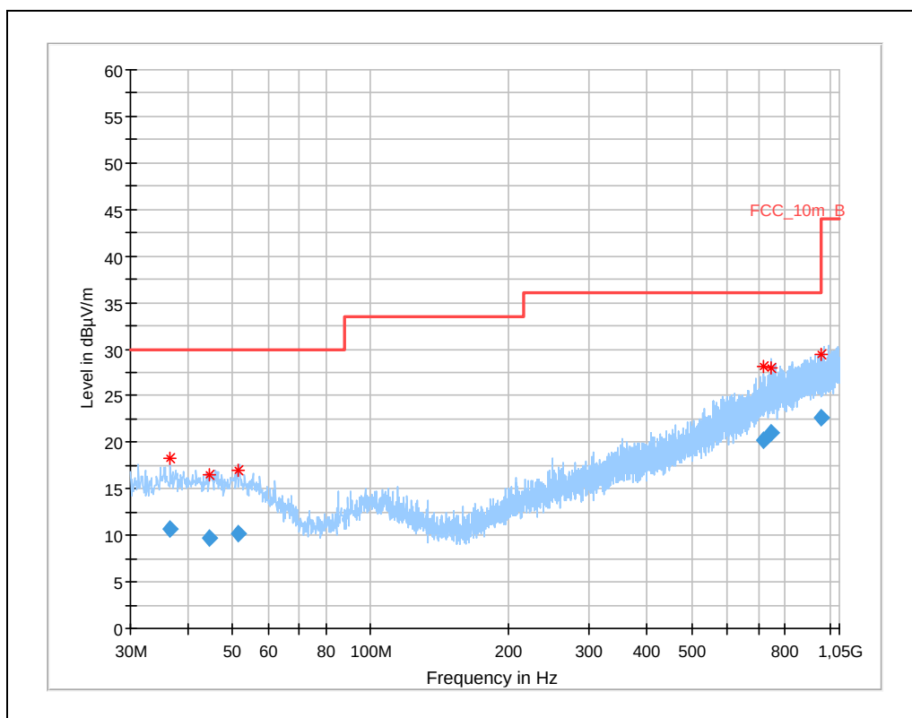
Plot 29: 30 MHz – 1 GHz, antenna horizontal / vertical, low frequency
