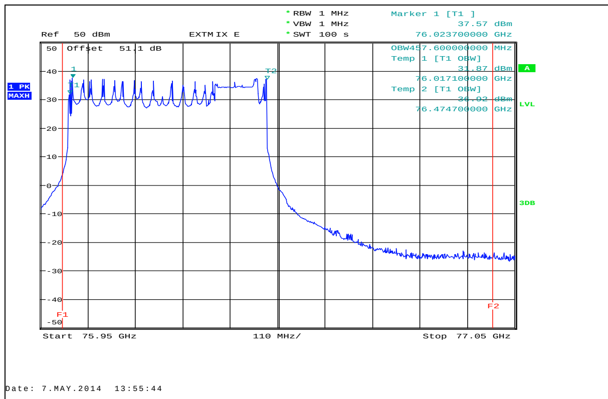
Plot 26: Occupied bandwidth (99%), T_{min} / V_{min} - V_{max} , high frequency
