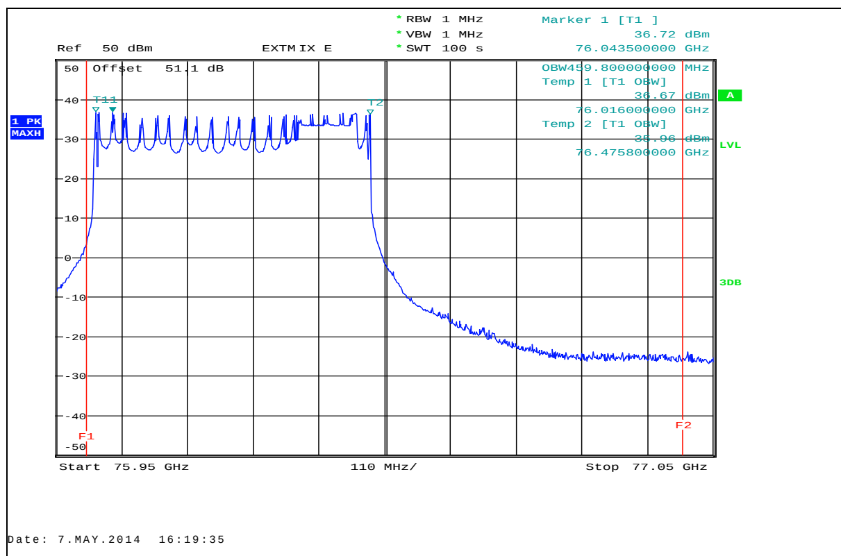
Plot 27: Occupied bandwidth (99%), T_{\max} / V_{\min} - V_{\max} , high frequency
