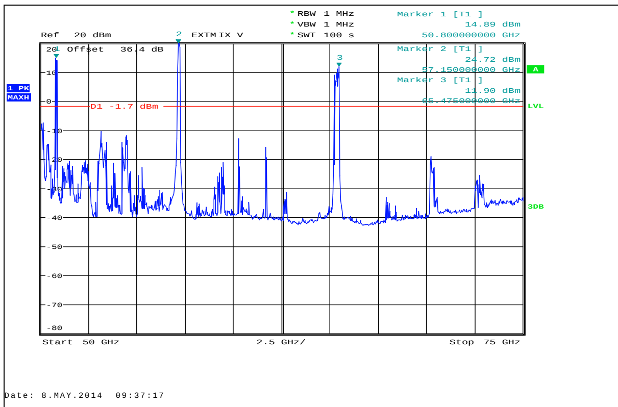
Plot 39: 50 GHz – 75 GHz, antenna horizontal / vertical, low / mid / high frequency
