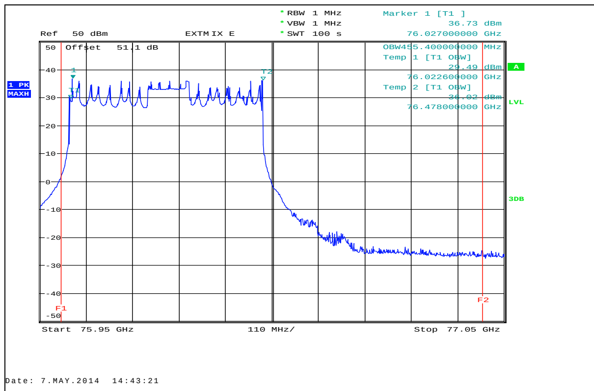
Plot 24: Occupied bandwidth (99%), T_{\max} / V_{\min} - V_{\max} , mid frequency
