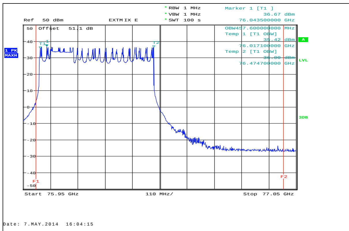
Plot 21: Occupied bandwidth (99%), T_{\max} / V_{\min} - V_{\max} , low frequency
