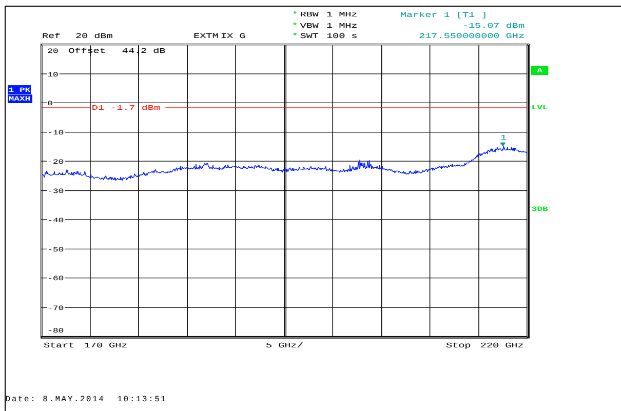
Plot 42: 170 GHz – 220 GHz, antenna horizontal / vertical, low / mid / high frequency
