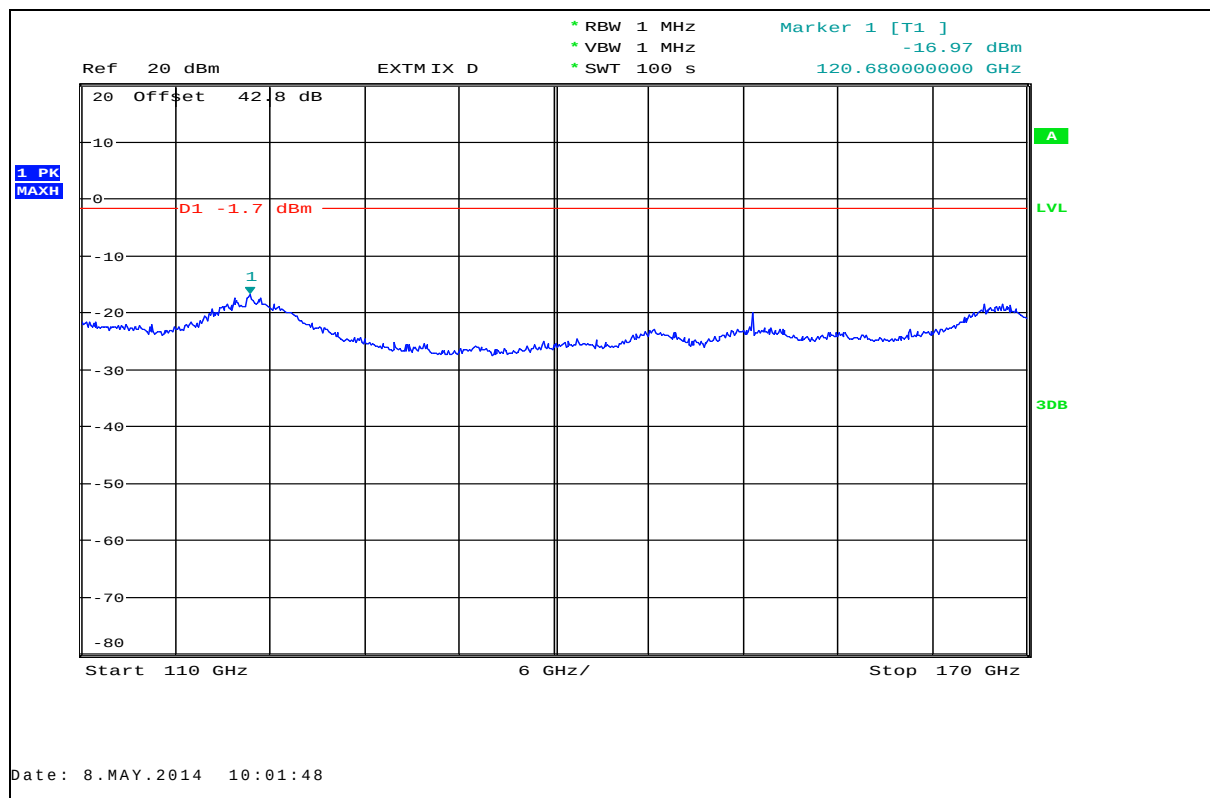
Plot 41: 110 GHz – 170 GHz, antenna horizontal / vertical, low / mid / high frequency
