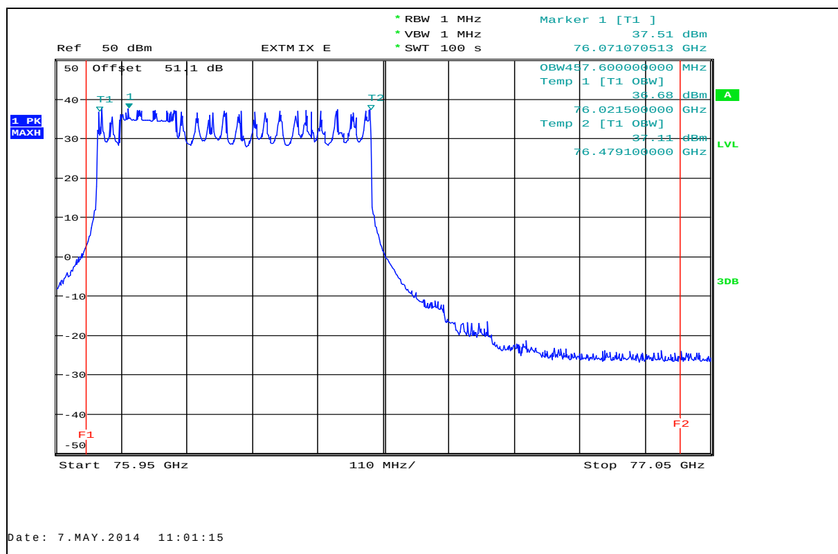
Plot 19: Occupied bandwidth (99%), T_{nom} / V_{nom} , low frequency
