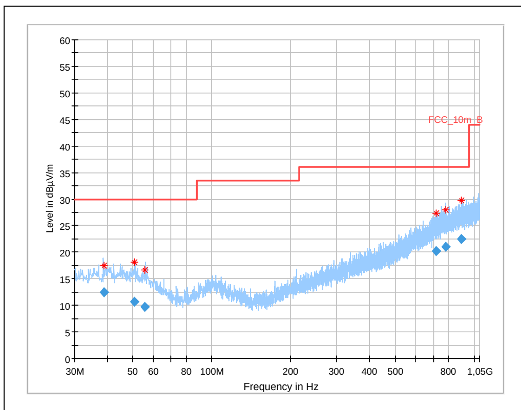
Plot 31: 30 MHz – 1 GHz, antenna horizontal / vertical, high frequency
