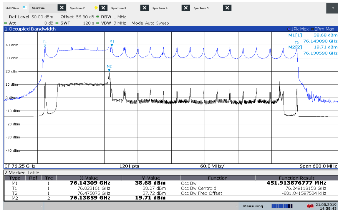
Plot 83: Mode 1, OBW, 20 °C / V_{nom}
