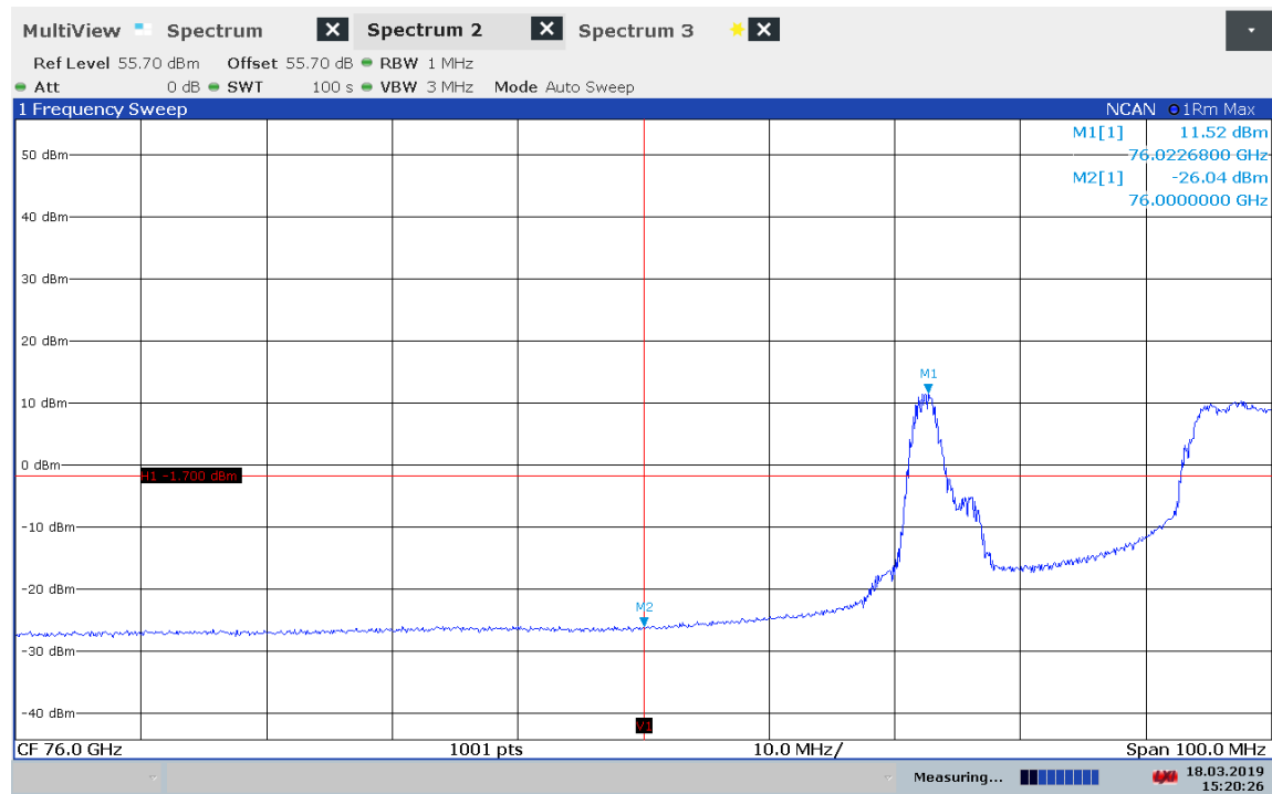
Plot 34: Lower BEC Mode 1
