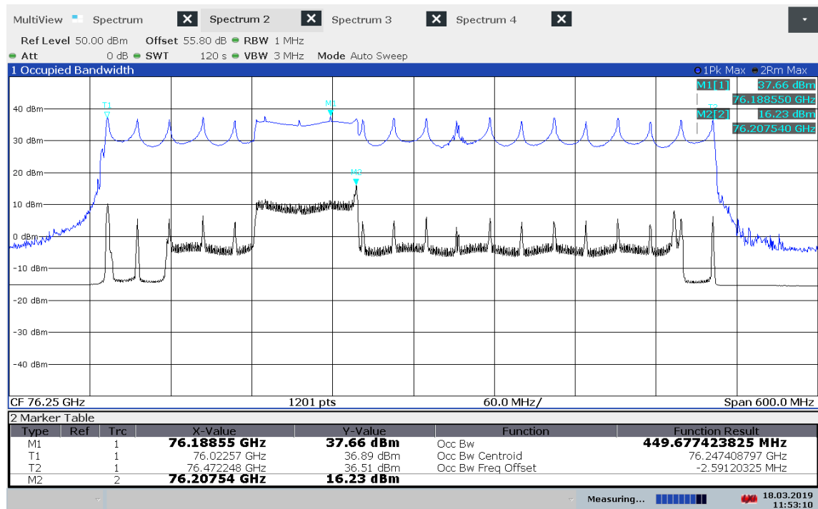
Plot 18: Mode 7, Peak power / Power spectral density, T_{\text{nom}} / V_{\text{nom}}
