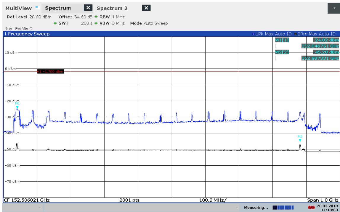
Plot 76: Final measurement 2 nd harmonic (valid for specified modes)
