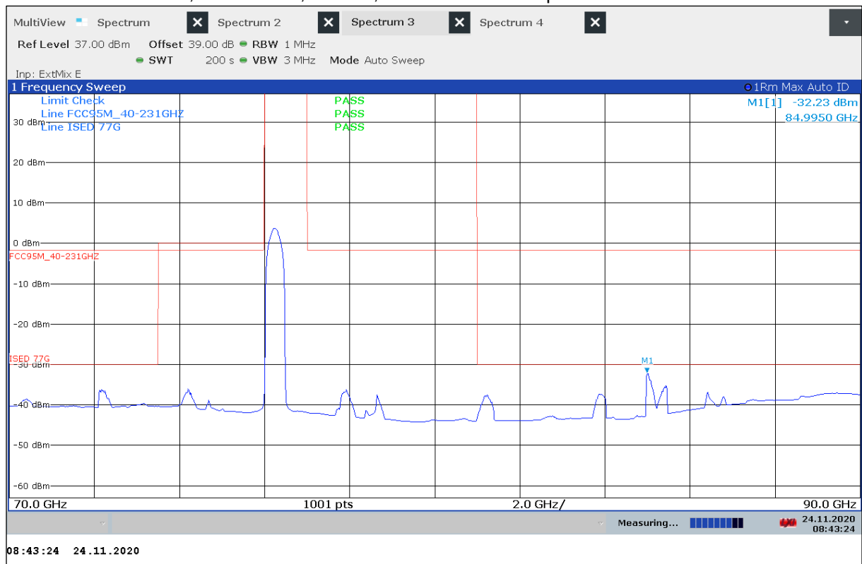
Plot 30: 70 GHz to 90 GHz, Out of Band, Mode 9, horizontal / vertical polarization
