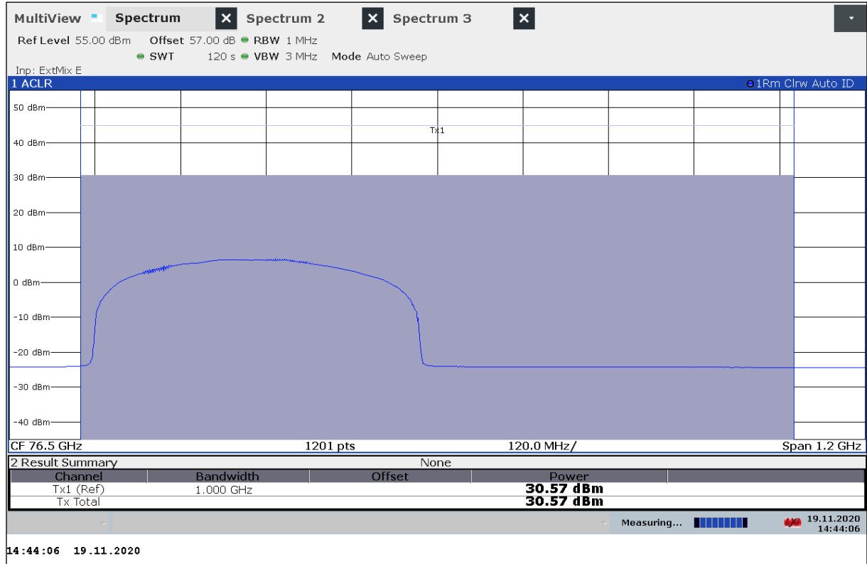
Plot 3: Channel power, Mode 9, T_{\text{nom}} / V_{\text{min}}-V_{\text{max}}
