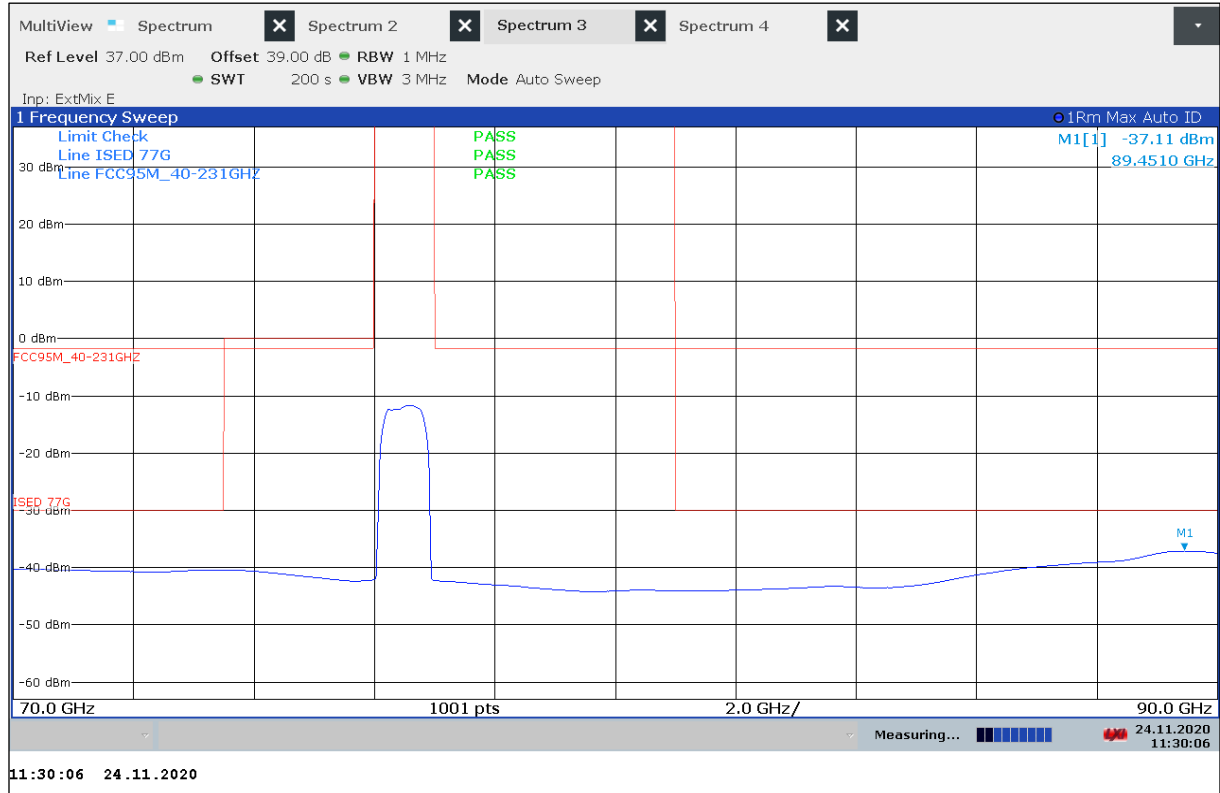
Plot 33: 70 GHz to 90 GHz, Out of Band, Mode 107, horizontal / vertical polarization
