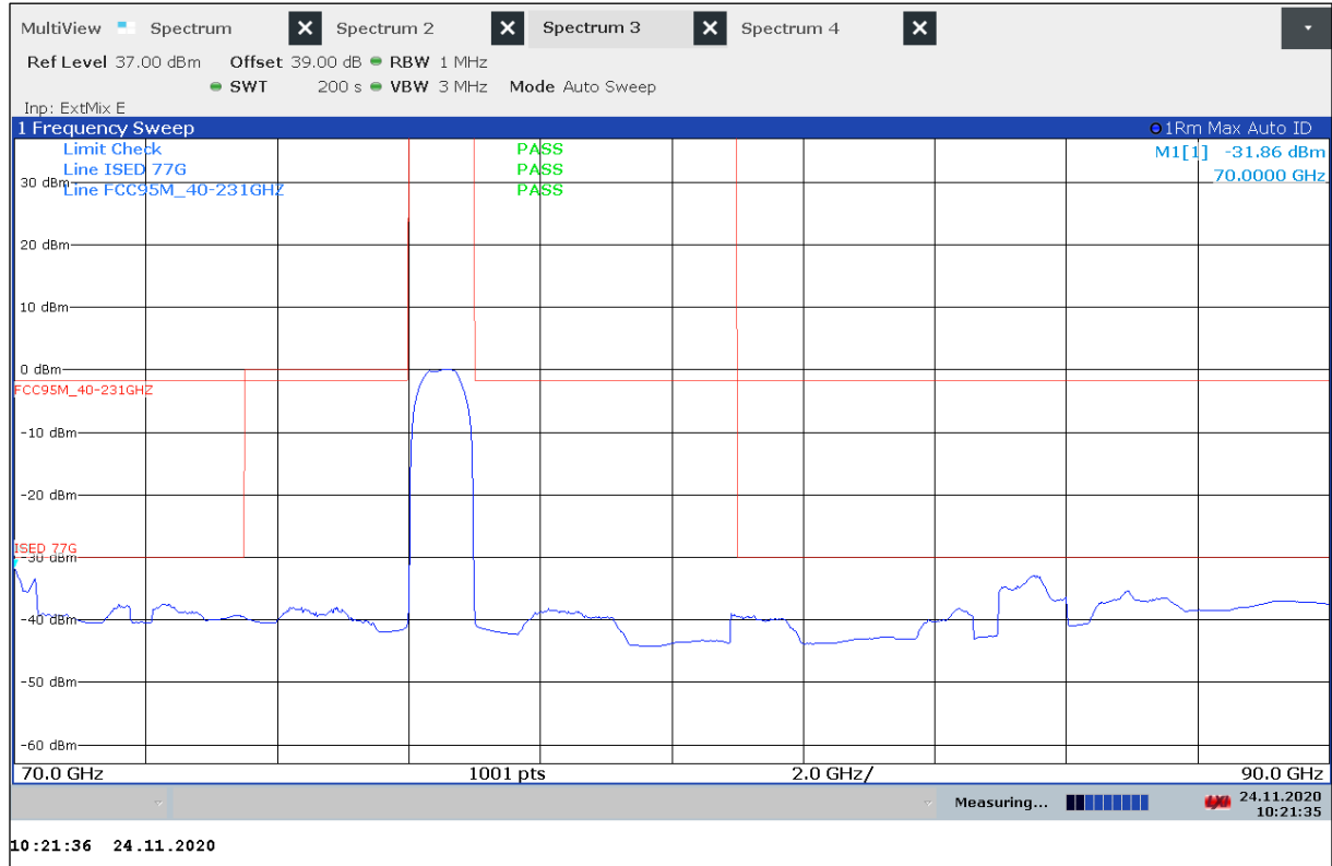
Plot 29: 70 GHz to 90 GHz, Out of Band, Mode 3, horizontal / vertical polarization
