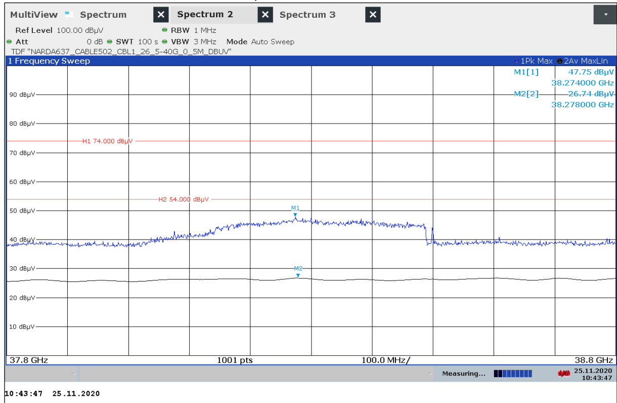
Plot 24: 38 GHz, Mode 21, horizontal / vertical polarization
