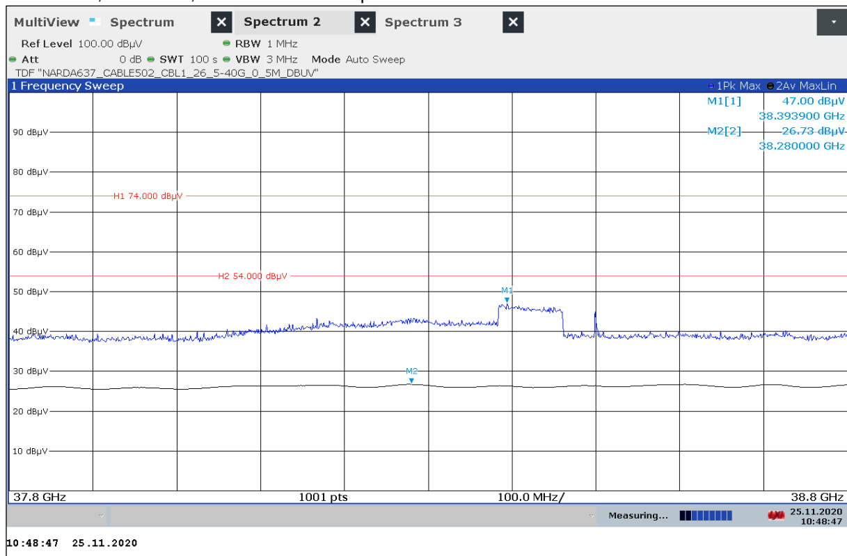
Plot 26: 38 GHz, Mode 107, horizontal / vertical polarization
