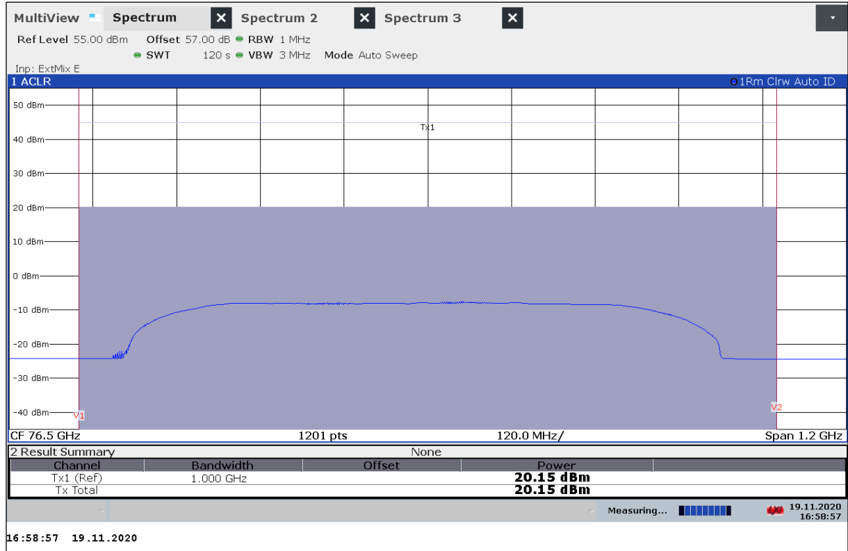
Plot 9: Channel power, Mode 107, T_{\text{nom}} / V_{\text{min}}-V_{\text{max}}
