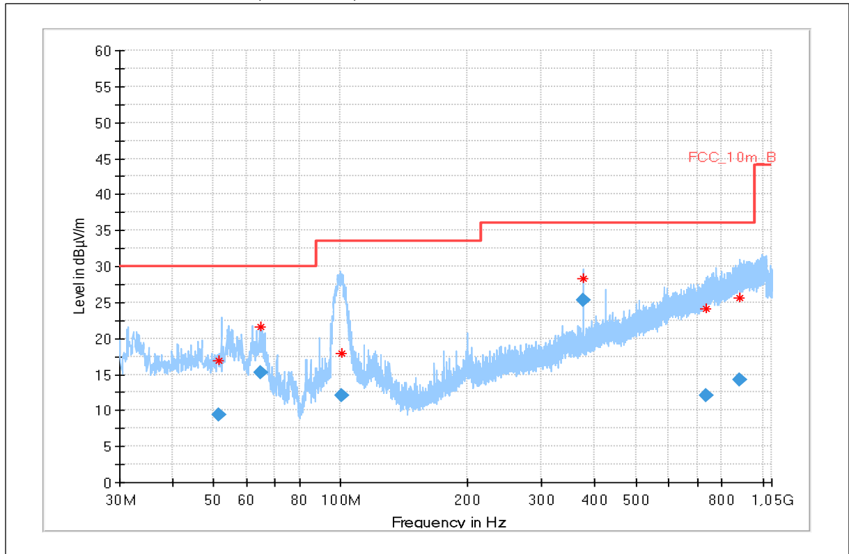
Plot 20: 30 MHz – 1 GHz, Mode 63 (Worst case), antenna vertical / horizontal
