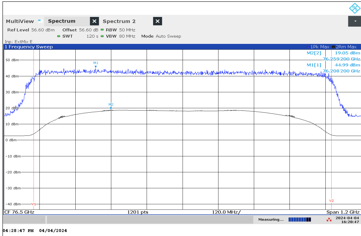
Plot 1: EIRP Peak Power, Mode 03, Peak detector, T_{\text{nom}} / V_{\text{nom}}
