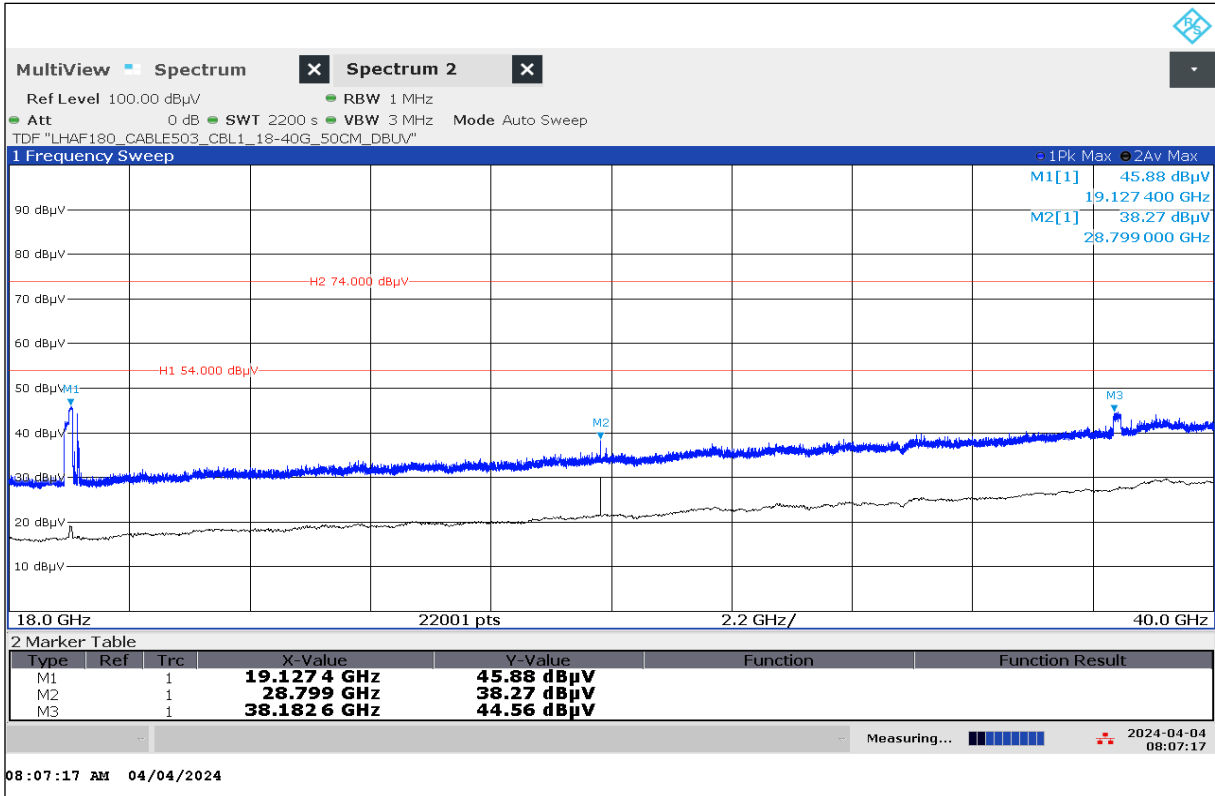
Plot 22: 18 GHz – 40 GHz, Mode 63 (Worst Case), antenna vertical / horizontal
