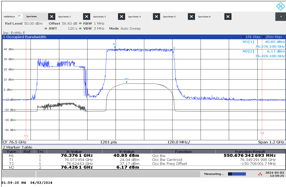
Plot 18: OBW, Mode 63, T_{nom} / V_{nom}
