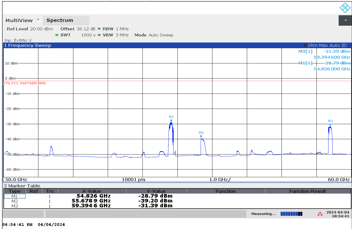
Plot 27: 50 GHz – 60 GHz, Mode 63 (Worst Case), antenna vertical / horizontal
