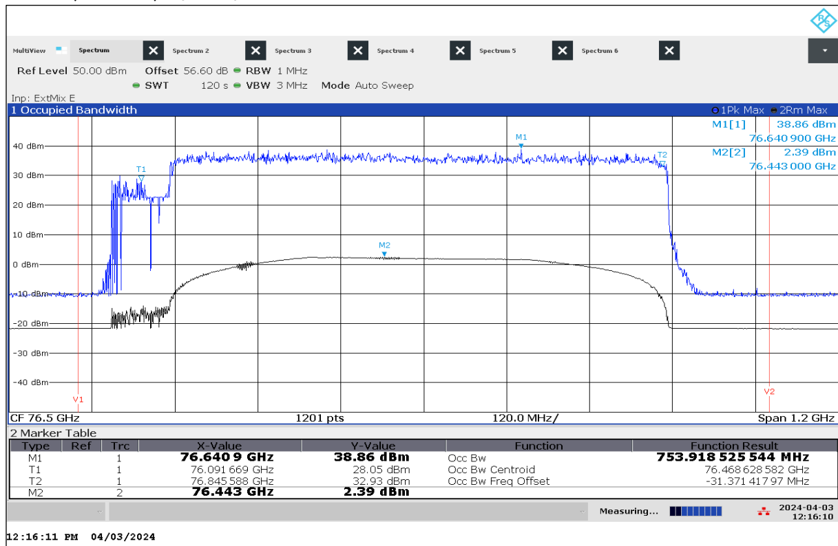
Plot 14: OBW, Mode 15, T_{nom} / V_{nom}
