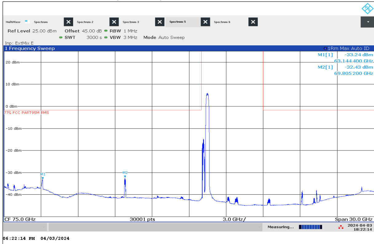
Plot 28: 60 GHz – 90 GHz, Mode 63 (Worst Case), antenna vertical / horizontal
