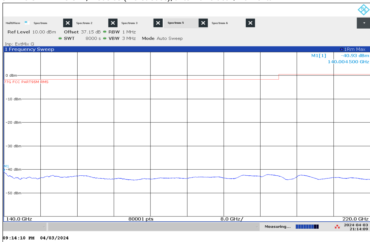
Plot 31: 140 GHz – 220 GHz, Mode 63 (Worst Case), antenna vertical / horizontal
