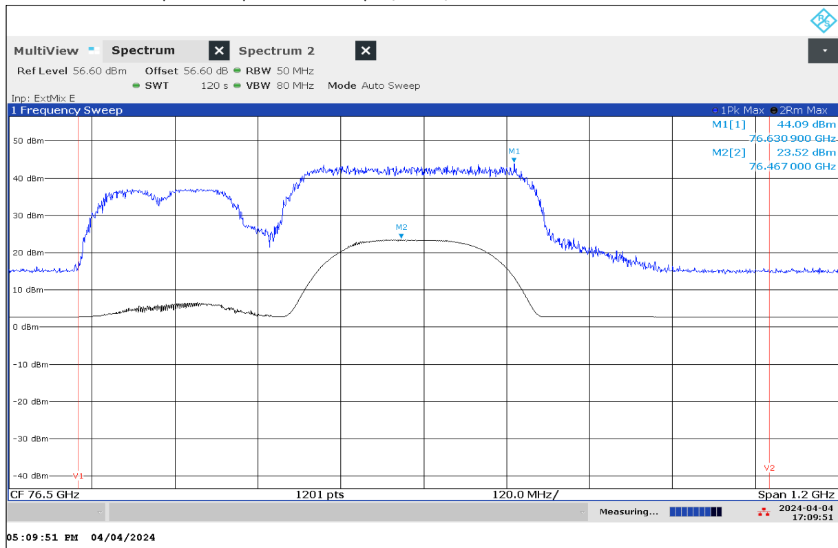
Plot 6: EIRP Peak Power, Mode 63, Peak detector, T_{nom} / V_{nom}
