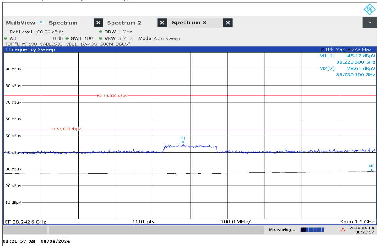
Plot 25: 38 GHz, Mode 63 (Worst case), antenna vertical / horizontal
