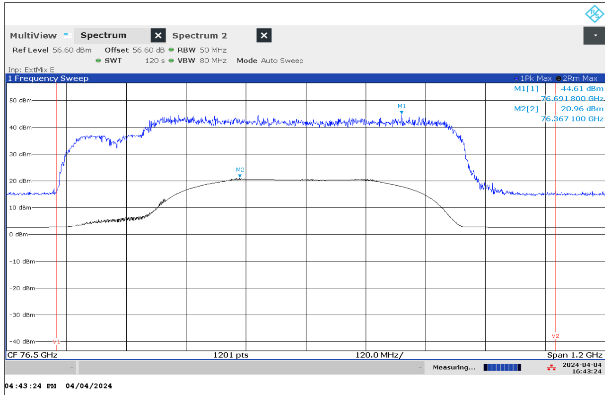
Plot 3: EIRP Peak Power, Mode 27, Peak detector, T_{\text{nom}} / V_{\text{nom}}
