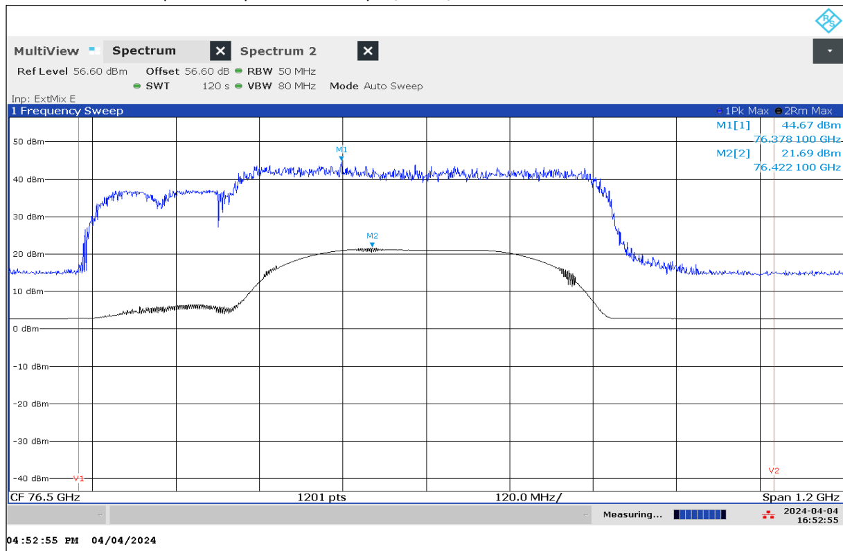
Plot 4: EIRP Peak Power, Mode 39, Peak detector, T_{\text{nom}} / V_{\text{nom}}
