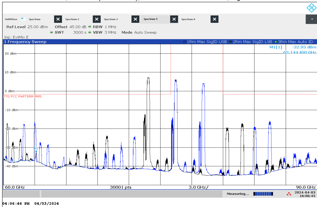
Plot 29: 60 GHz – 90 GHz, Mode 63 (Worst Case), antenna vertical / horizontal, Signal-ID function
