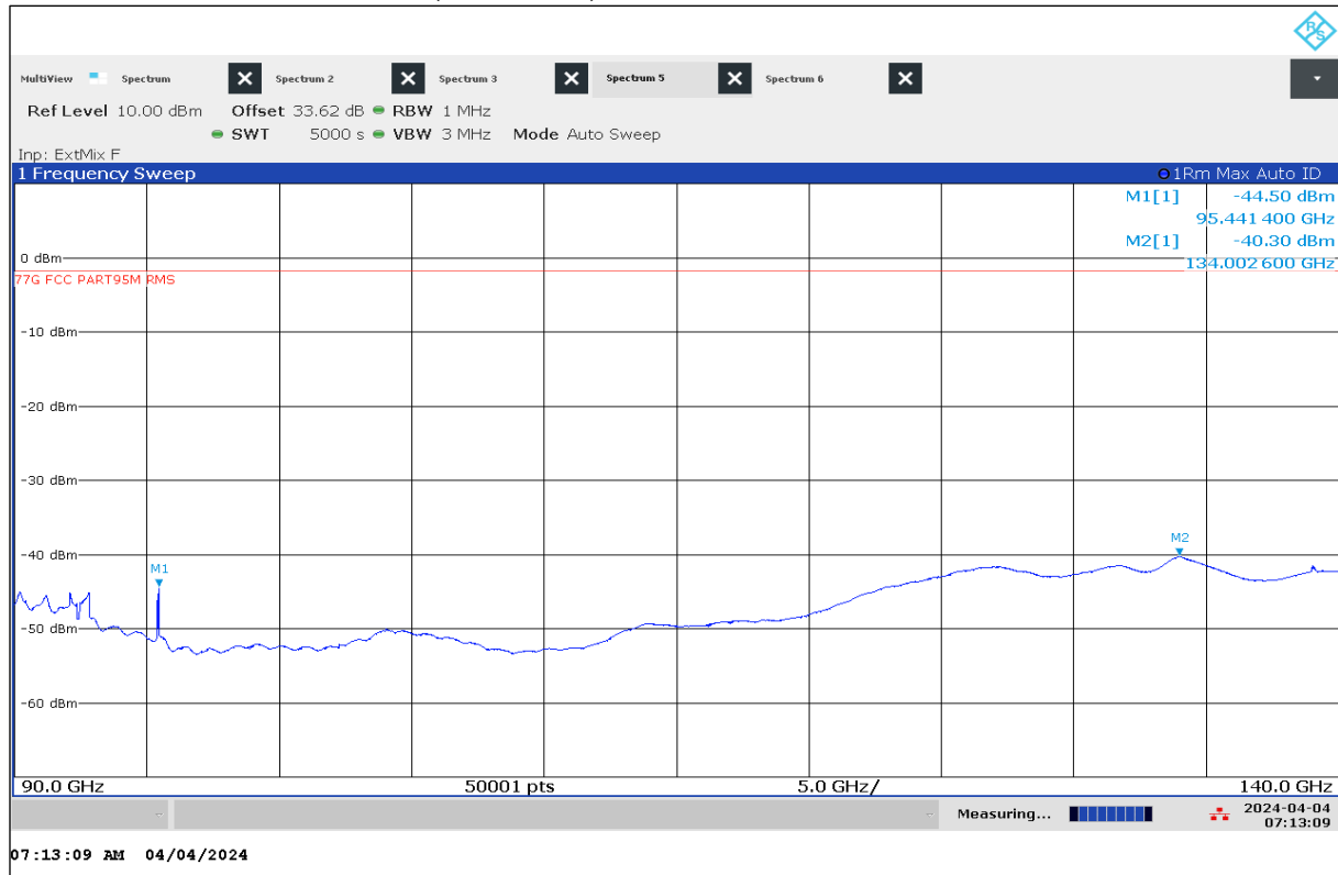
Plot 30: 90 GHz – 140 GHz, Mode 63 (Worst Case), antenna vertical / horizontal
