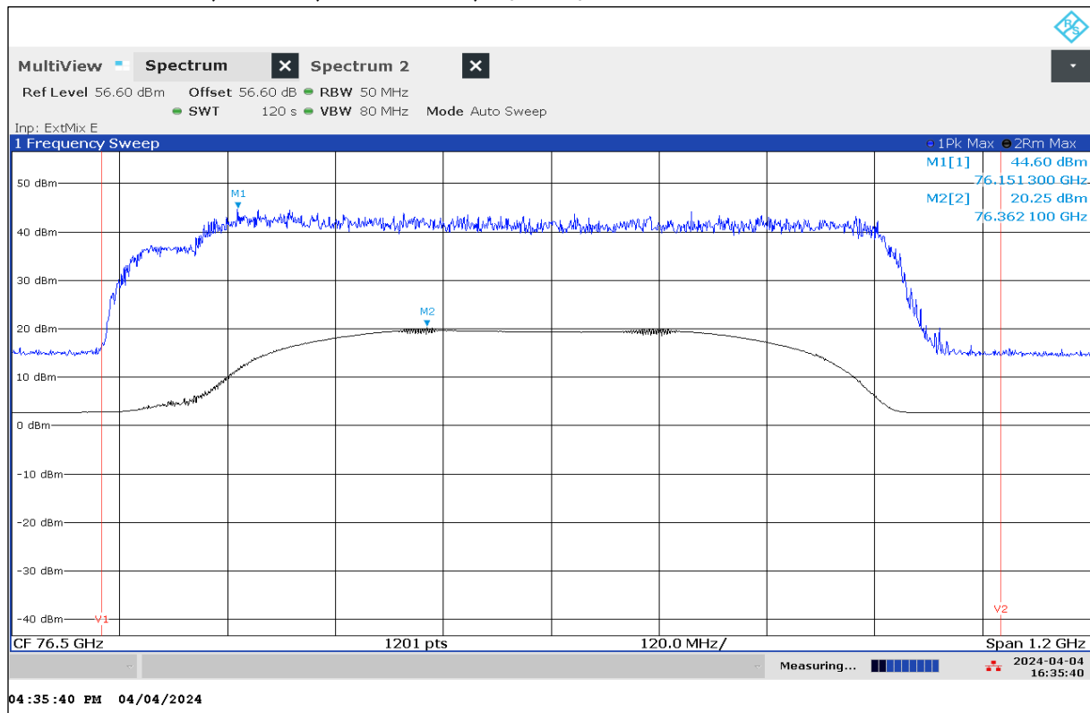
Plot 2: EIRP Peak Power, Mode 15, Peak detector, T_{\text{nom}} / V_{\text{nom}}
