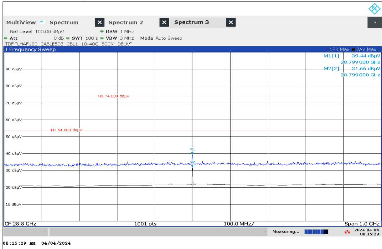
Plot 24: 29 GHz, Mode 63 (Worst case), antenna vertical / horizontal
