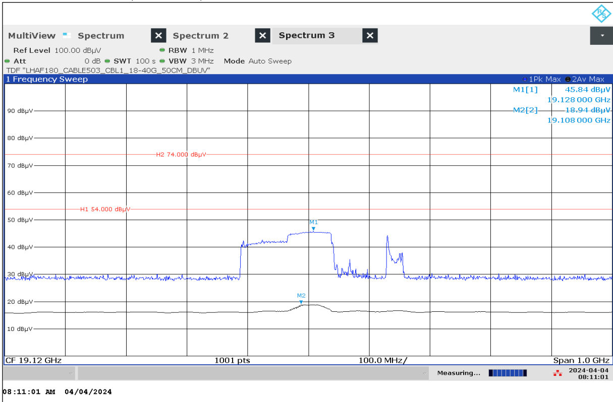
Plot 23: 19 GHz, Mode 63 (Worst case), antenna vertical / horizontal
