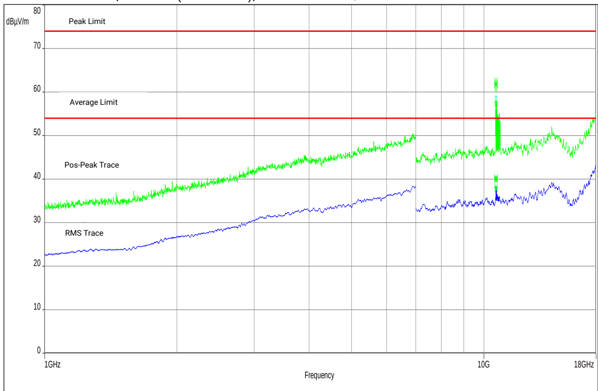
Plot 21: 1 GHz – 18 GHz, Mode 63 (Worst Case), antenna vertical / horizontal
