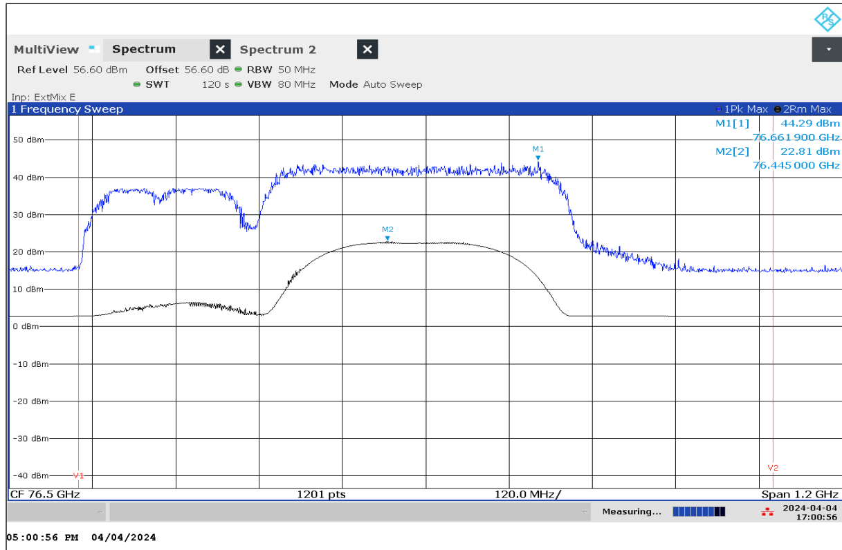
Plot 5: EIRP Peak Power, Mode 51, Peak detector, T_{nom} / V_{nom}
