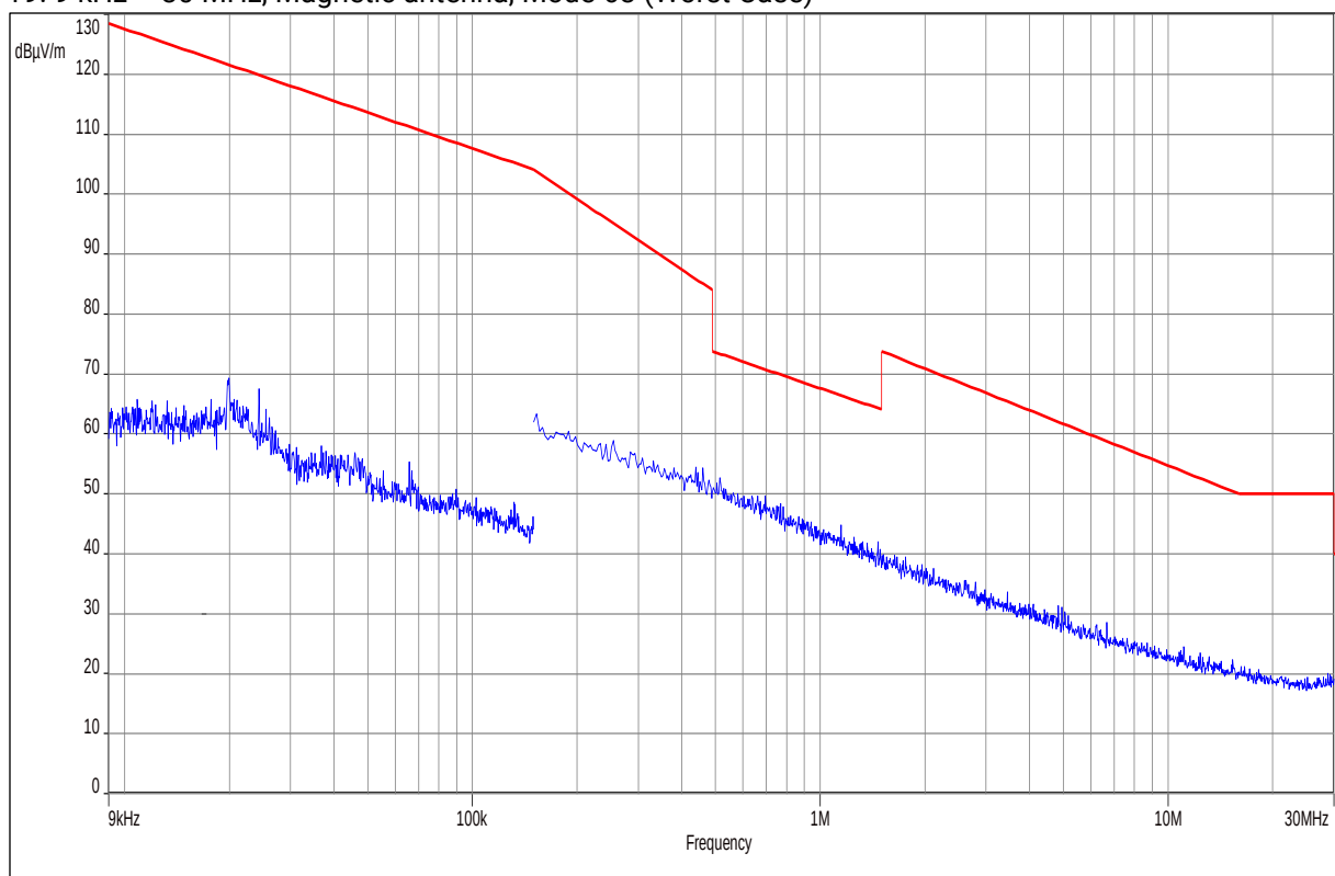
Plot 19: 9 kHz – 30 MHz, Magnetic antenna, Mode 63 (Worst Case)
