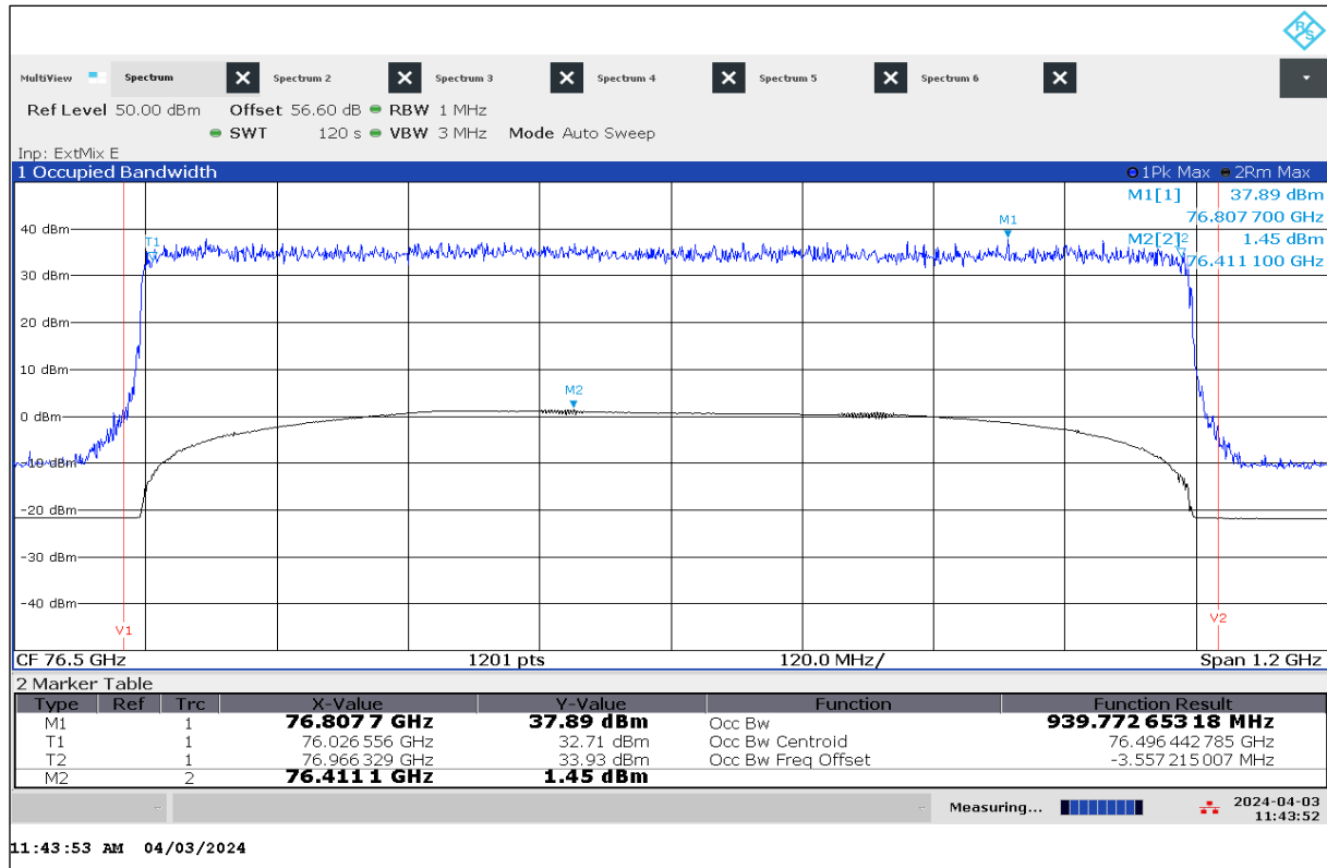
Plot 13: OBW, Mode 03, T_{nom} / V_{nom}
