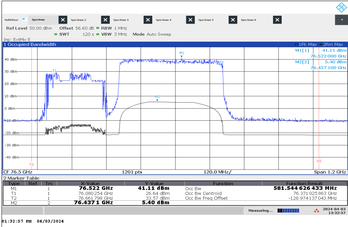
Plot 17: OBW, Mode 51, T_{nom} / V_{nom}
