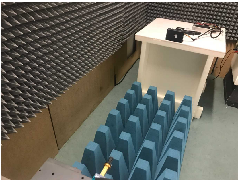
Photo 4: >18 GHz test setup
