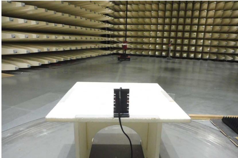
Photo 5: 30 MHz-1 GHz test setup
