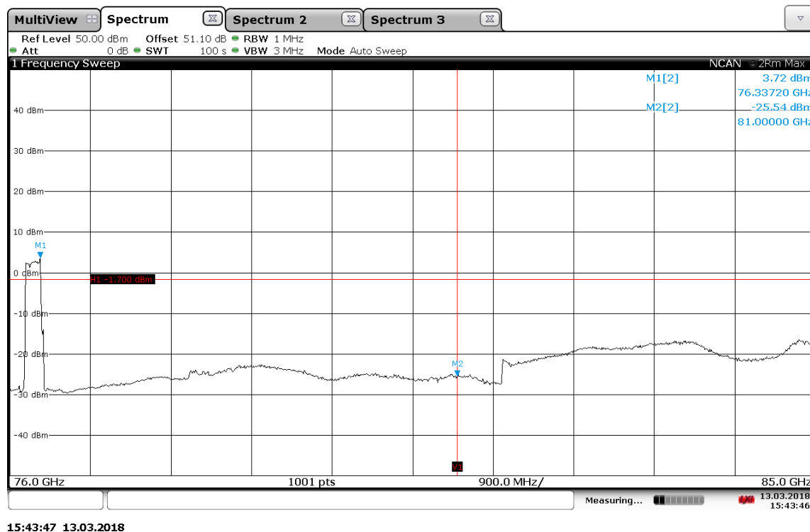
Plot 38: Mode 1, upper BEC
