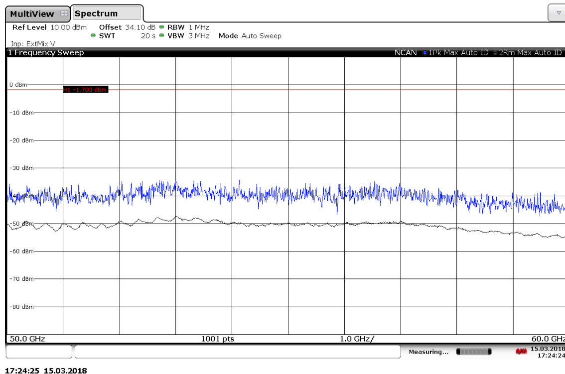
Plot 57: 50 GHz to 60 GHz, Stop-Mode, middle
