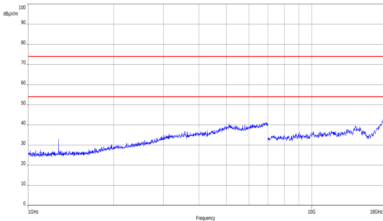
Plot 49: 1 GHz to 18 GHz, Stop-Mode, middle
