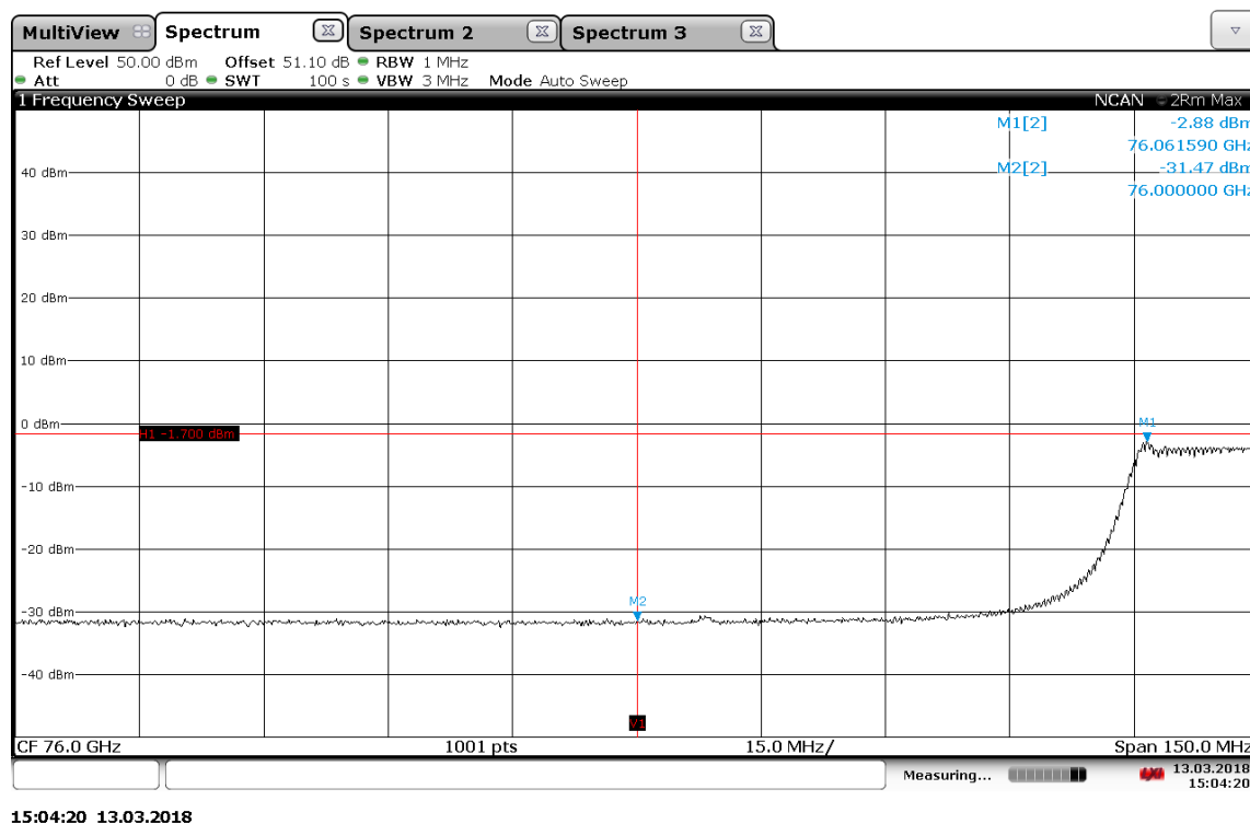
Plot 36: Mode 160, lower BEC
