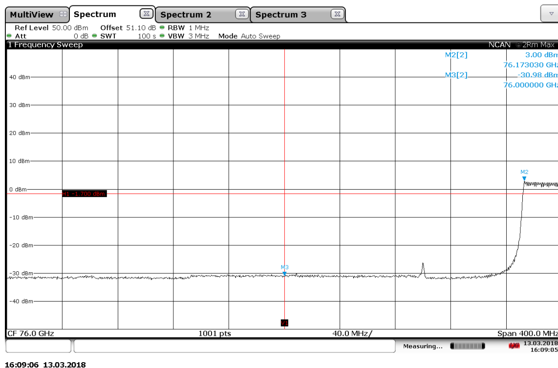
Plot 35: Mode 1, lower BEC
