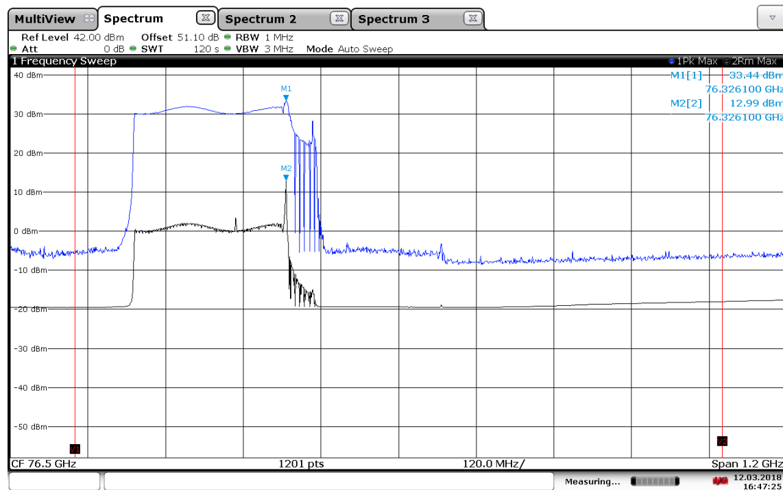
Plot 9: Mode 6, Radiated peak power, T_{nom} / V_{nom}
