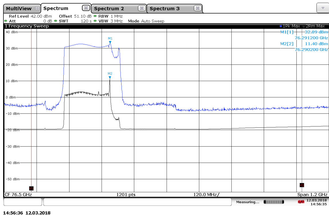
Plot 3: Mode 2, Radiated peak power, T_{\text{nom}} / V_{\text{nom}}
