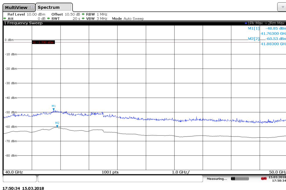
Plot 55: 40 GHz to 50 GHz, Stop-Mode, top
