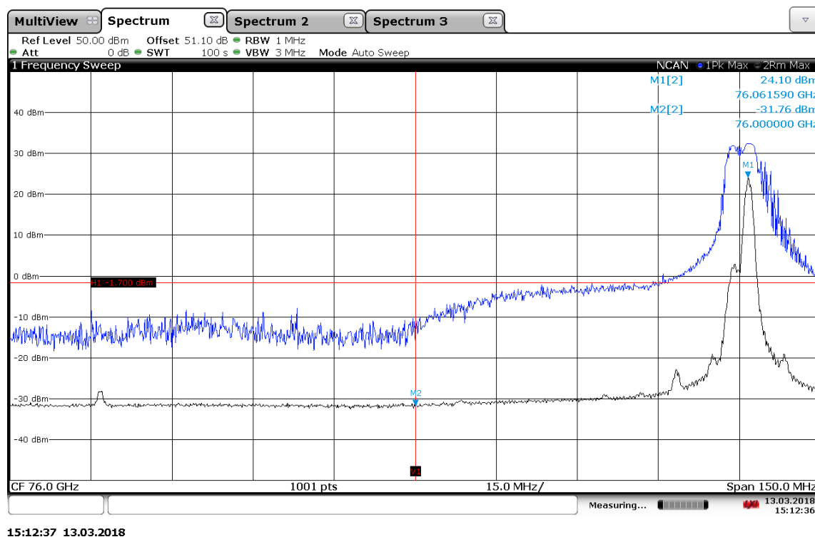
Plot 37: Stop-Mode, Bottom, lower BEC
