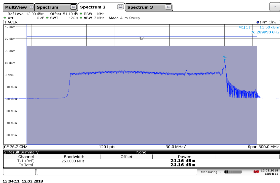
Plot 4: Mode 2, Radiated mean power, T_{\text{nom}} / V_{\text{nom}}
