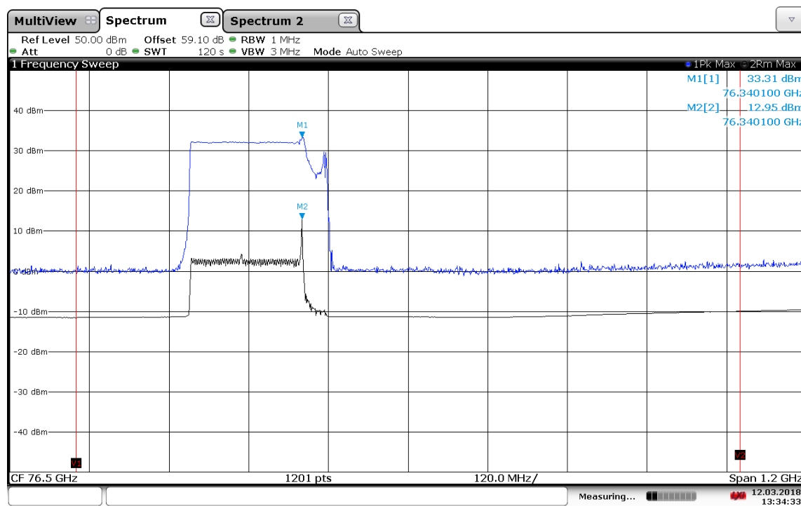
Plot 1: Mode 1, Radiated peak power, T_{\text{nom}} / V_{\text{nom}}
