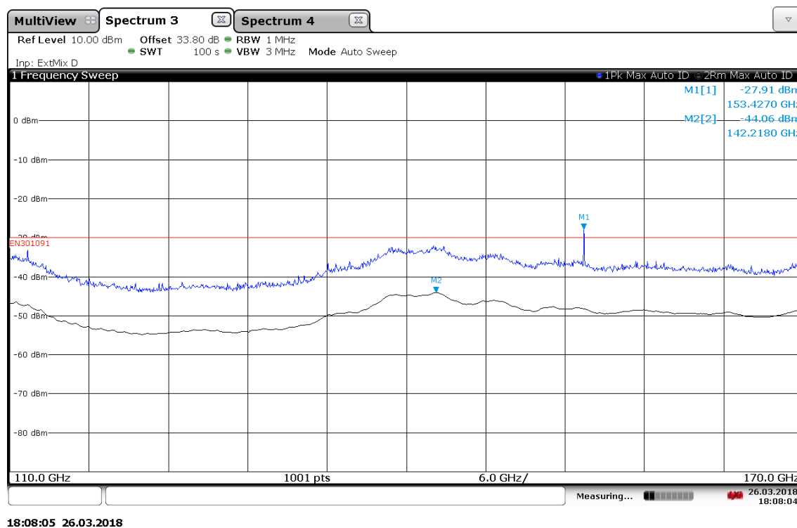
Plot 64: 110 GHz to 170 GHz, Stop-Mode, top
