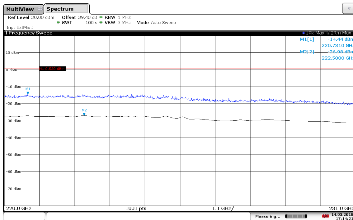
Plot 66: 220 GHz to 231 GHz, Stop-Mode, bottom, middle, top
