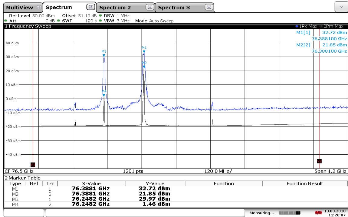
Plot 16: Stop-Mode, middle, Radiated peak power, T_{\text{nom}} / V_{\text{nom}}
