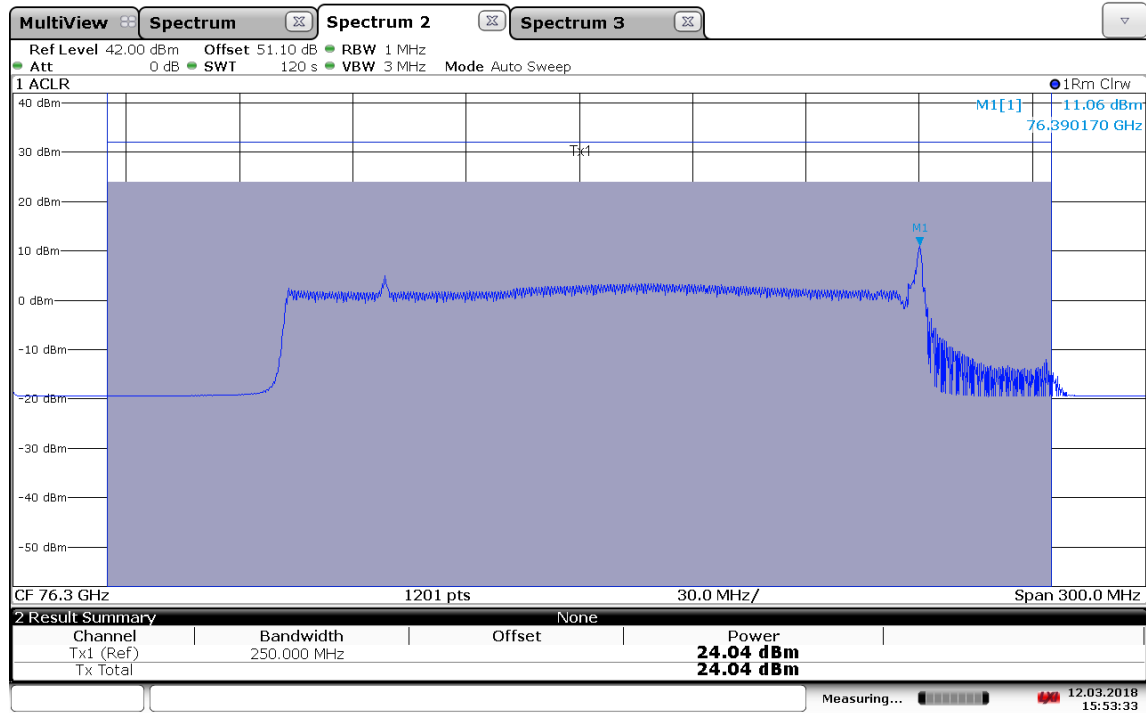
Plot 6: Mode 3, Radiated mean power, T_{\text{nom}} / V_{\text{nom}}
