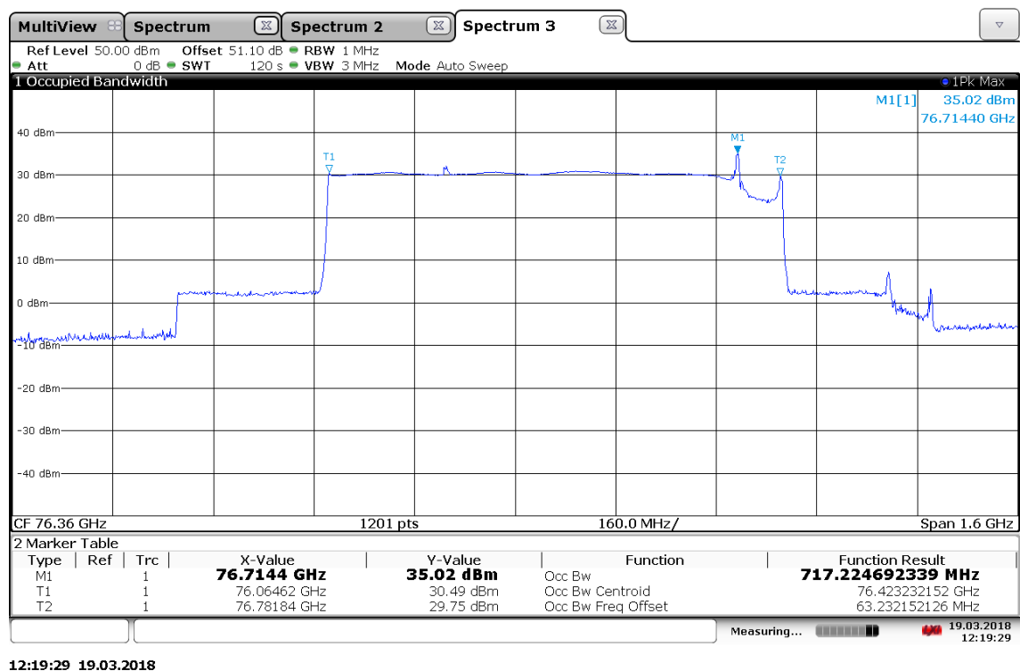
Plot 72: OBW, -40 °C
