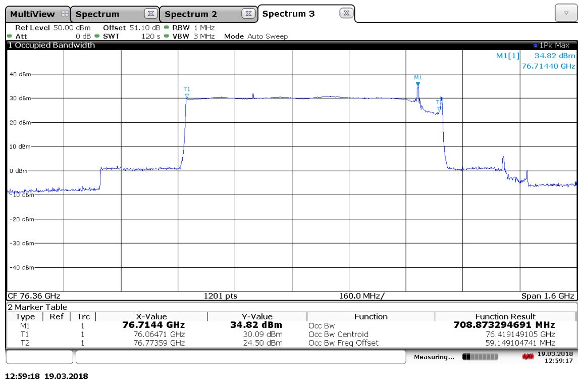
Plot 73: OBW, -30 °C
