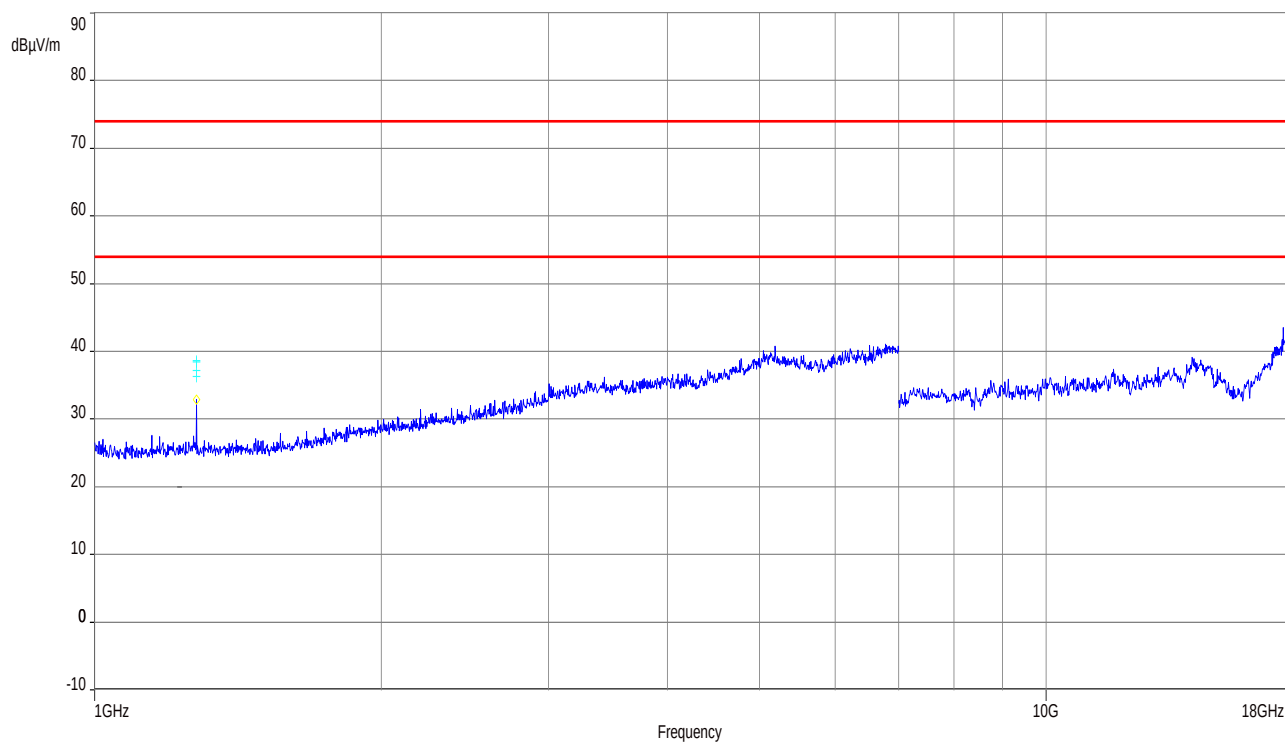
Plot 48: 1 GHz to 18 GHz, Stop-Mode, bottom
