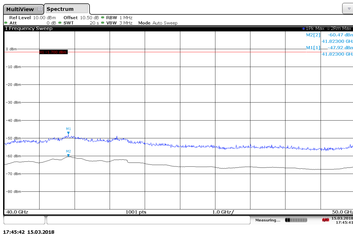
Plot 53: 40 GHz to 50 GHz, Stop-Mode, bottom
