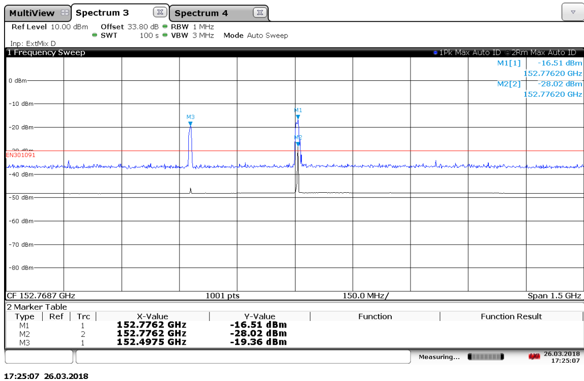
Plot 70: Final measurement, 2 nd harmonic, Stop-Mode, middle
