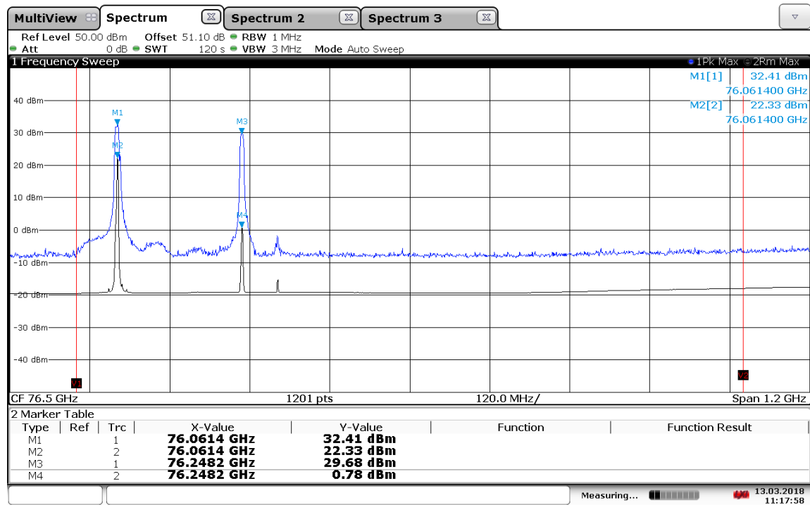
Plot 15: Stop-Mode, bottom, Radiated peak power, T_{\text{nom}} / V_{\text{nom}}
