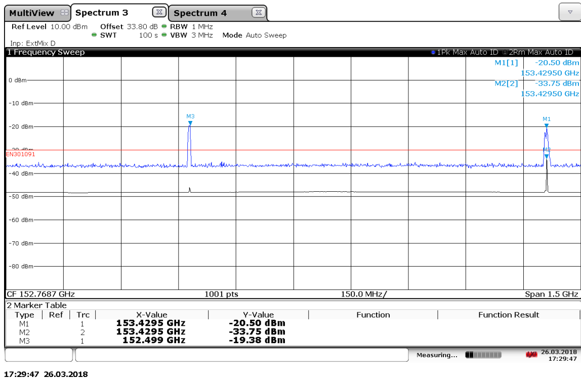
Plot 71: Final measurement, 2 nd harmonic, Stop-Mode, top
