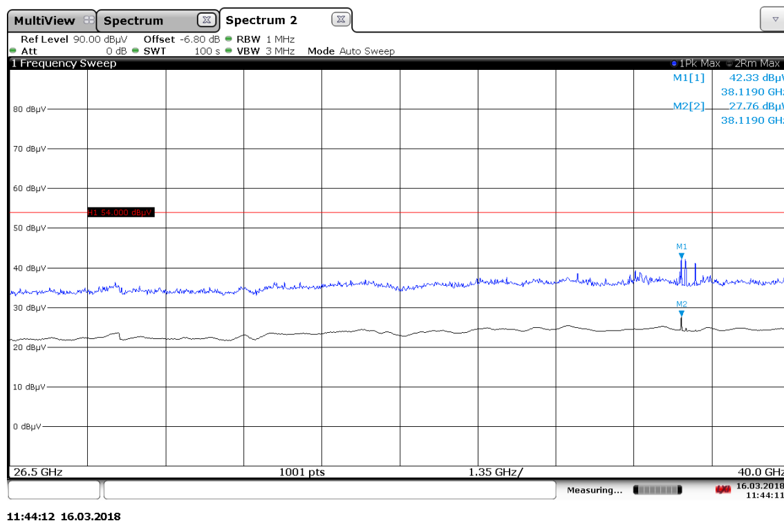
Plot 52: 26.5 GHz to 40 GHz, Stop-Mode, bottom, middle, top
