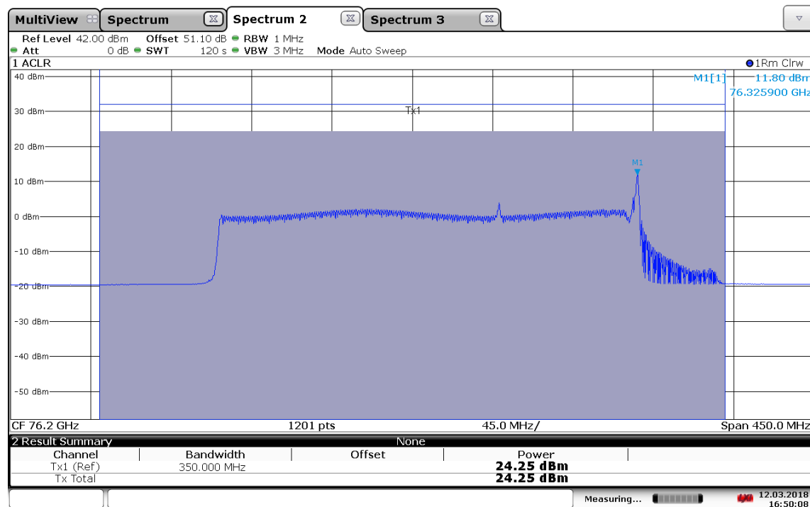
Plot 10: Mode 6, Radiated mean power, T_{nom} / V_{nom}
