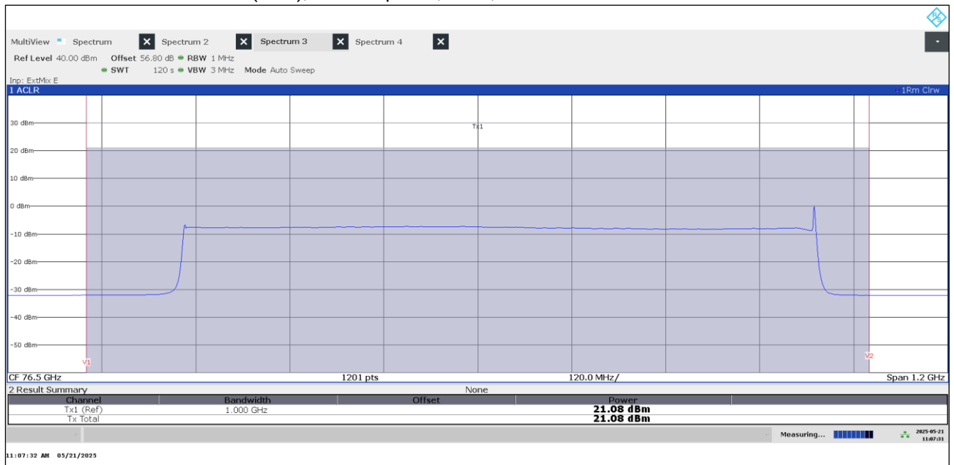
Plot 9: Radiated Mean Power (EIRP), Channel power, EUT1, Mode 78
