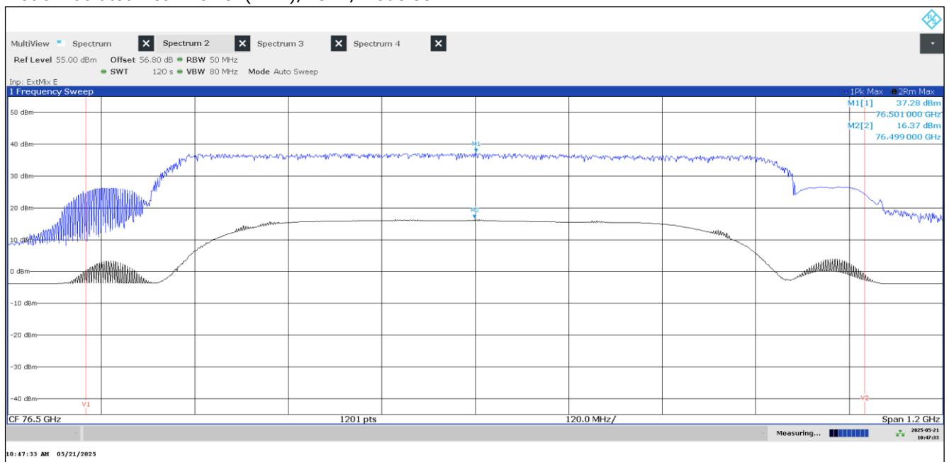
Plot 6: Radiated Peak Power (EIRP), EUT1, Mode 03
