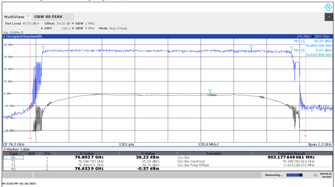
Plot 12: Occupied Bandwidth (99%), EUT 1, Mode 02
