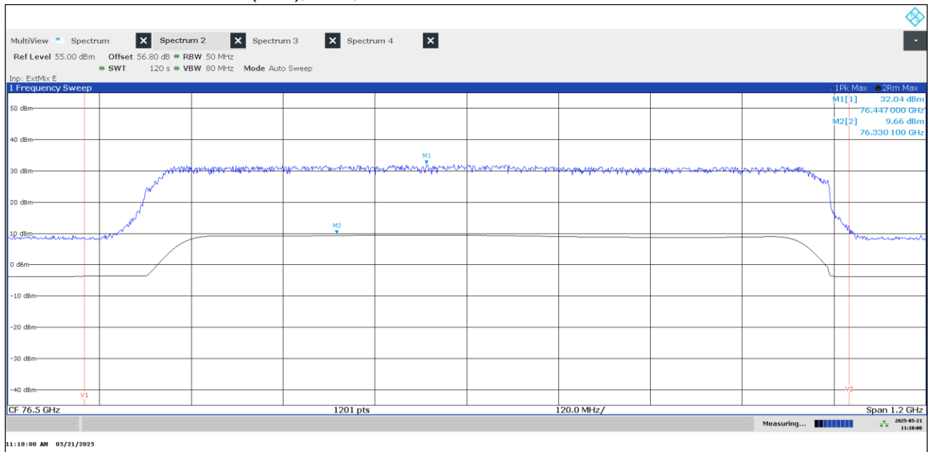
Plot 10: Radiated Peak Power (EIRP), EUT1, Mode 78
