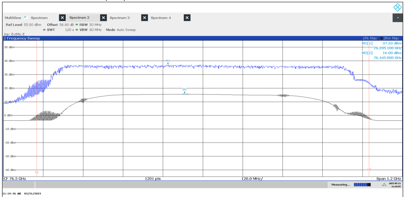
Plot 8: Radiated Peak Power (EIRP), EUT1, Mode 04
