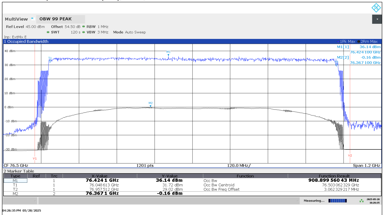
Plot 11: Occupied Bandwidth (99%), EUT 1, Mode 01
