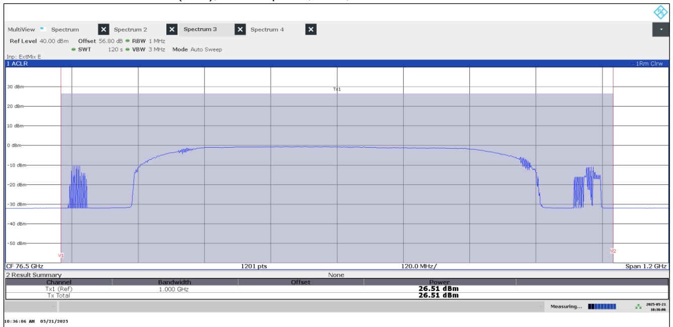
Plot 5: Radiated Mean Power (EIRP), Channel power, EUT1, Mode 03
