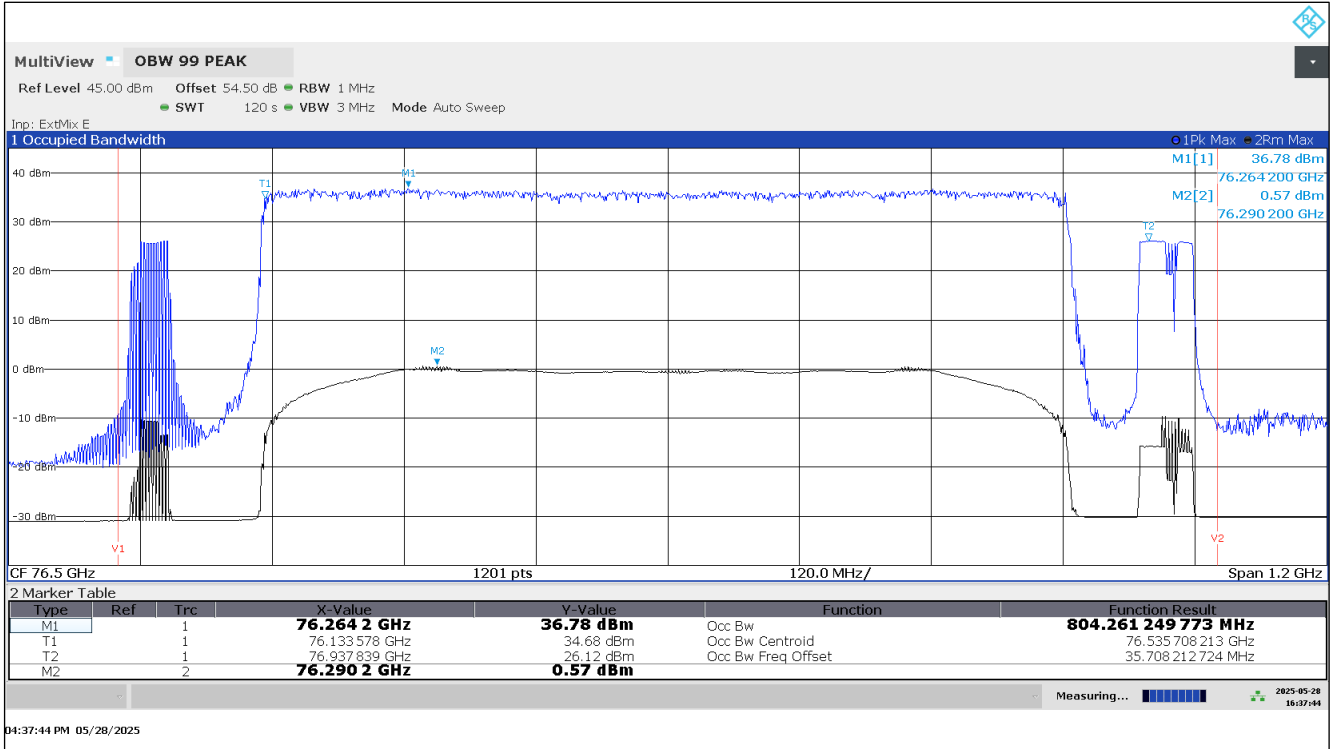
Plot 13: Occupied Bandwidth (99%), EUT 1, Mode 03
