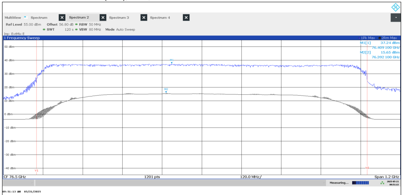
Plot 4: Radiated Peak Power (EIRP), EUT1, Mode 02
