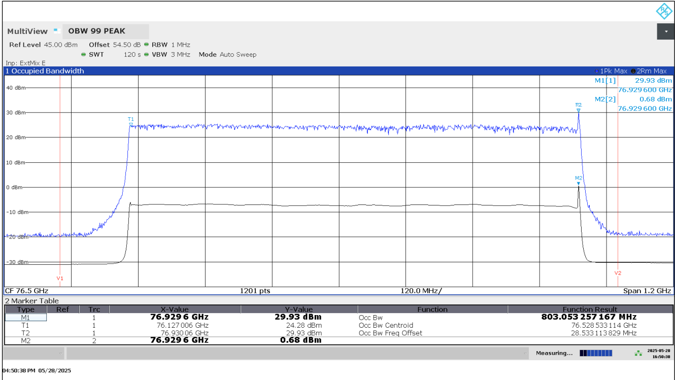
Plot 15: Occupied Bandwidth (99%), EUT 1, Mode 78
