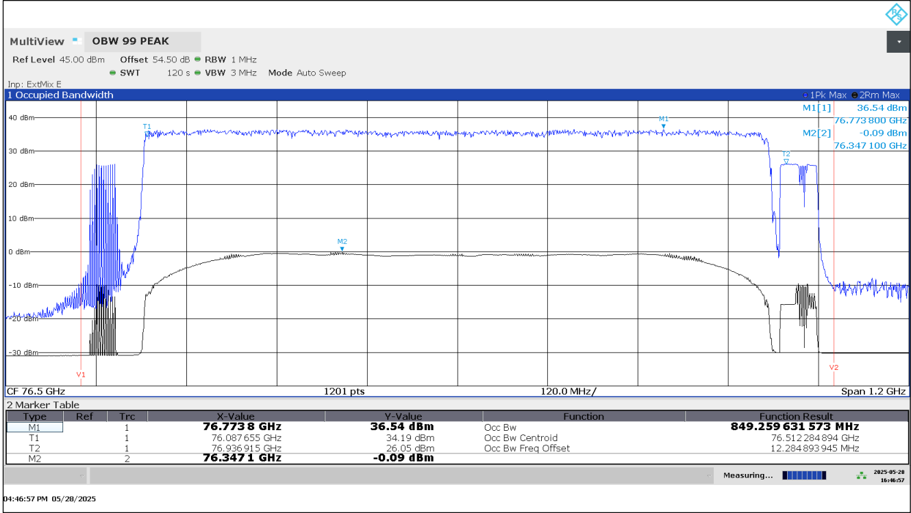
Plot 14: Occupied Bandwidth (99%), EUT 1, Mode 04
