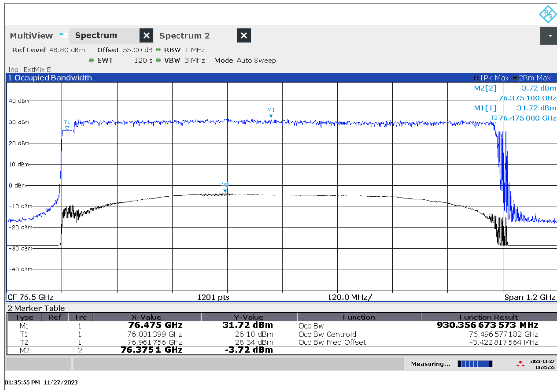
Plot 14: OBW, Mode 27, T_{\text{min}} / V_{\text{min-max}}
