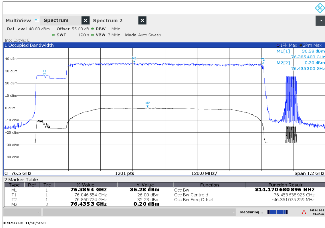
Plot 10: OBW, Mode 21, T_{\text{nom}} / V_{\min-\max}
