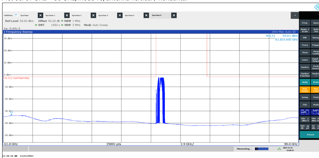
Plot 66: 61 GHz – 90 GHz, Mode 15, antenna vertical / horizontal
