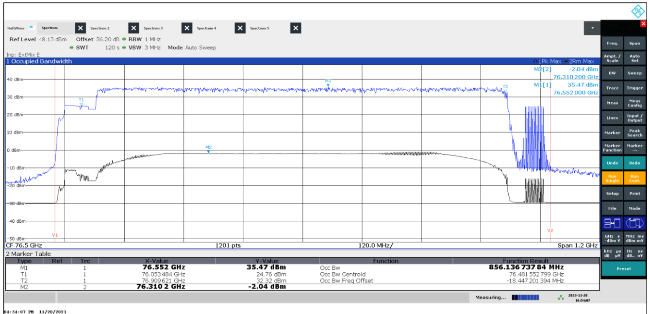
Plot 10: OBW, Mode 21, T_{\text{nom}} / V_{\min-\max}
