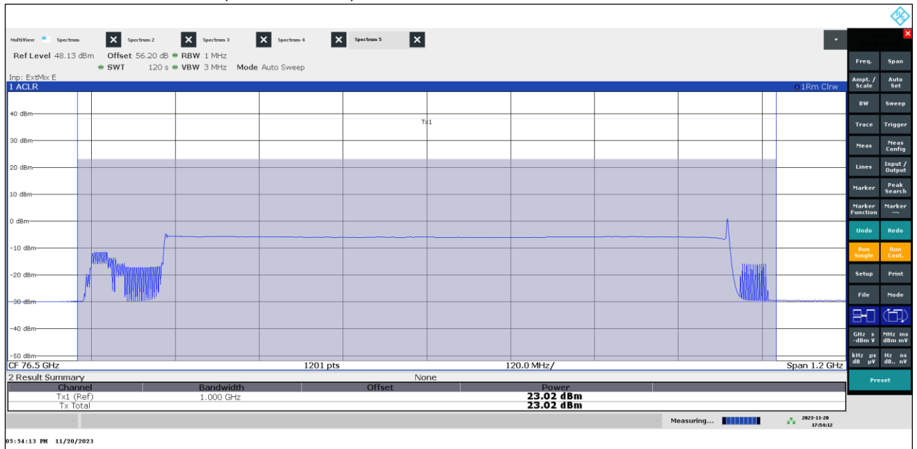
Plot 52: EIRP Mean Power (Channel Power), Mode 80, RMS detector, T_{\text{nom}} / V_{\text{min-max}}
