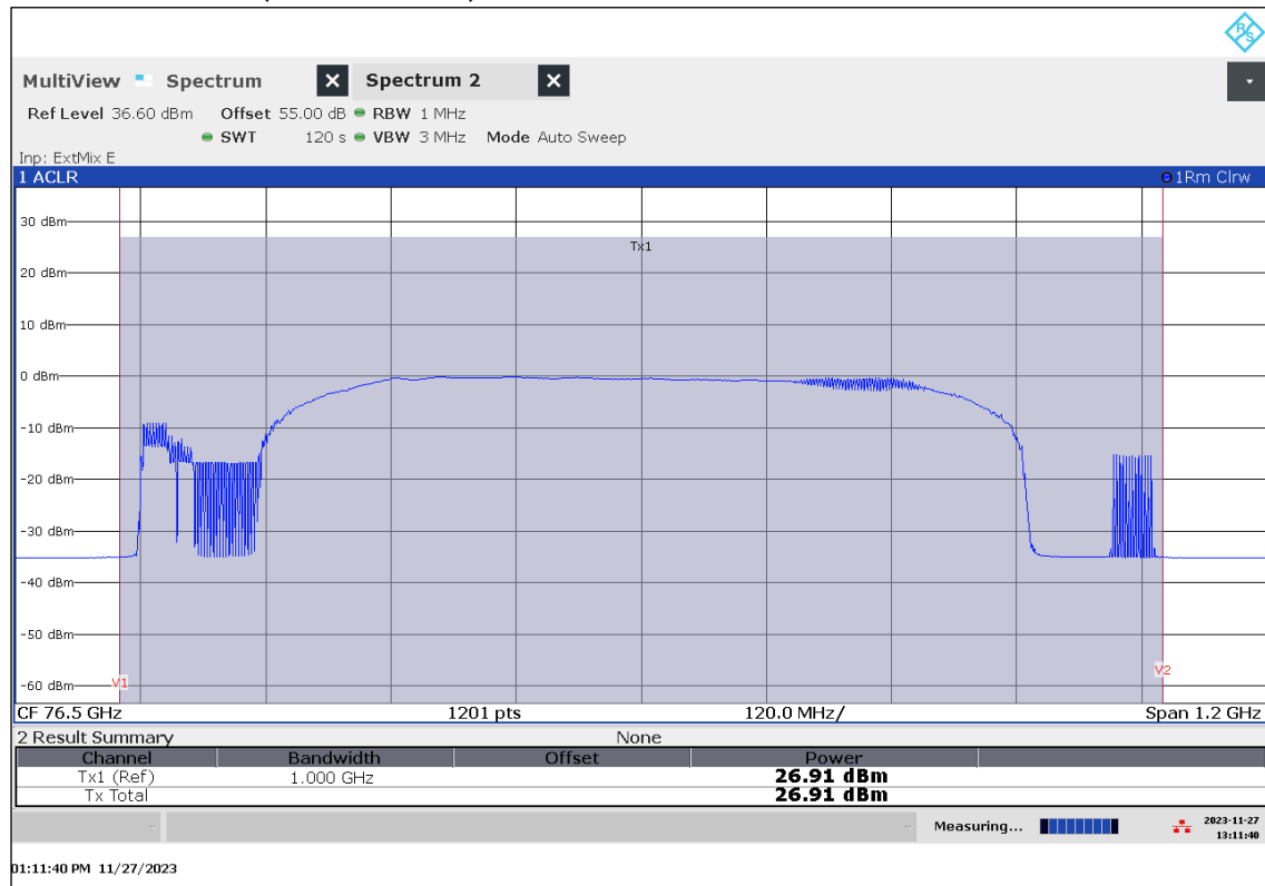
Plot 35: EIRP Mean Power (Channel Power), Mode 15, RMS detector, T_{\text{min}} / V_{\text{min-max}}
