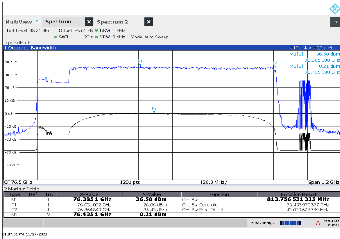
Plot 8: OBW, Mode 15, T_{\text{min}} / V_{\text{min-max}}
