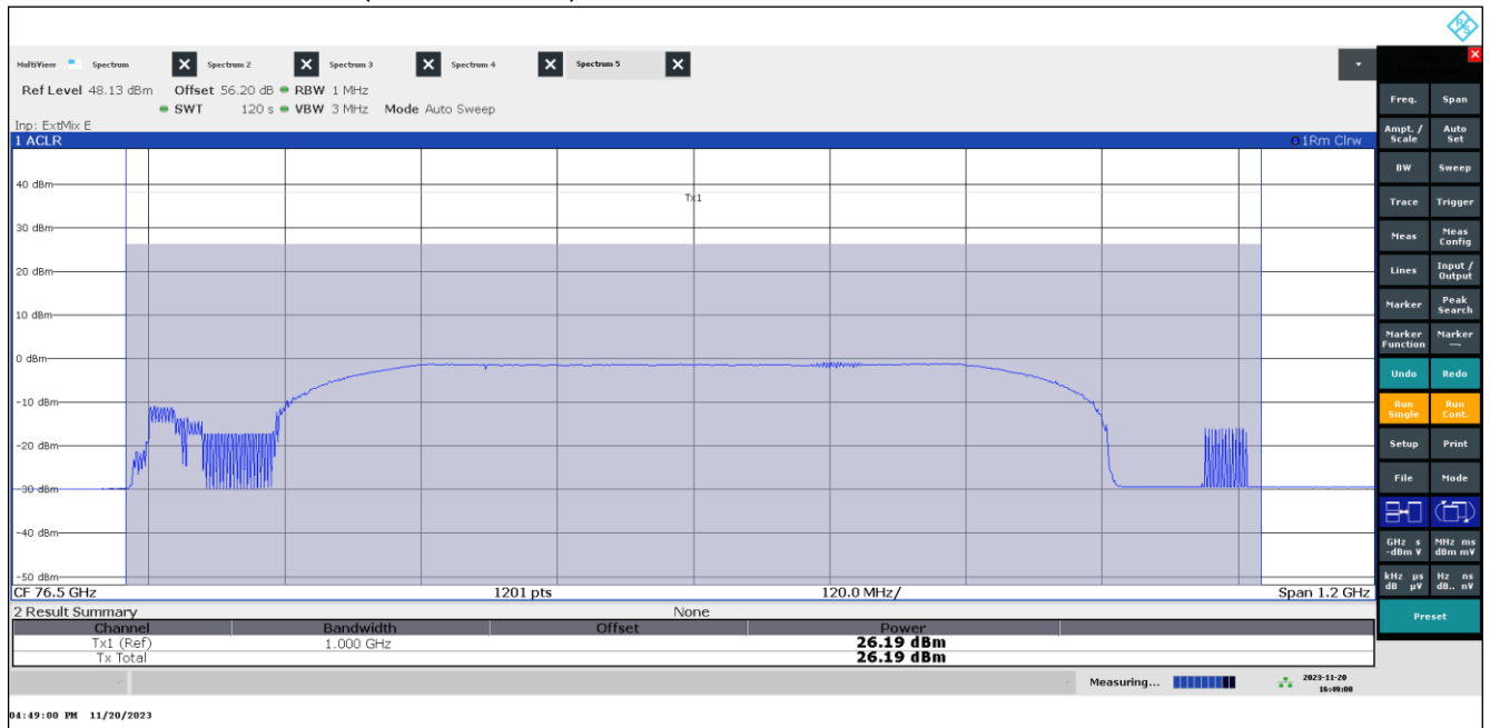
Plot 34: EIRP Mean Power (Channel Power), Mode 15, RMS detector, T_{\text{nom}} / V_{\text{min-max}}
