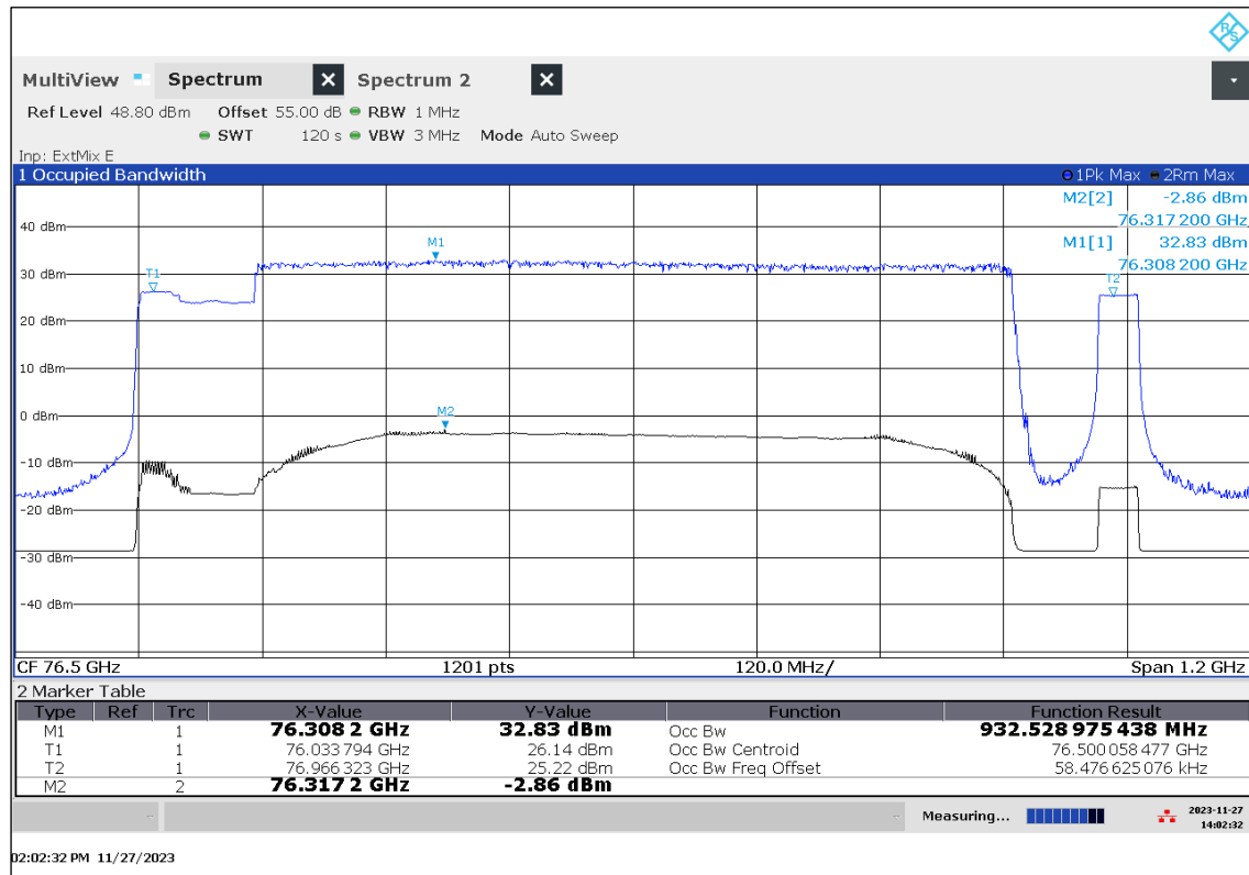
Plot 20: OBW, Mode 51, T_{\text{min}} / V_{\text{min-max}}
