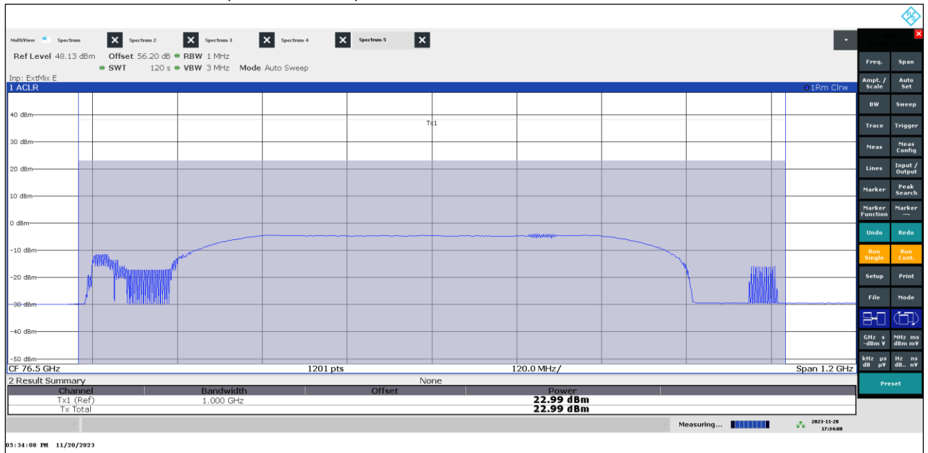
Plot 46: EIRP Mean Power (Channel Power), Mode 51, RMS detector, T_{\text{nom}} / V_{\text{min-max}}
