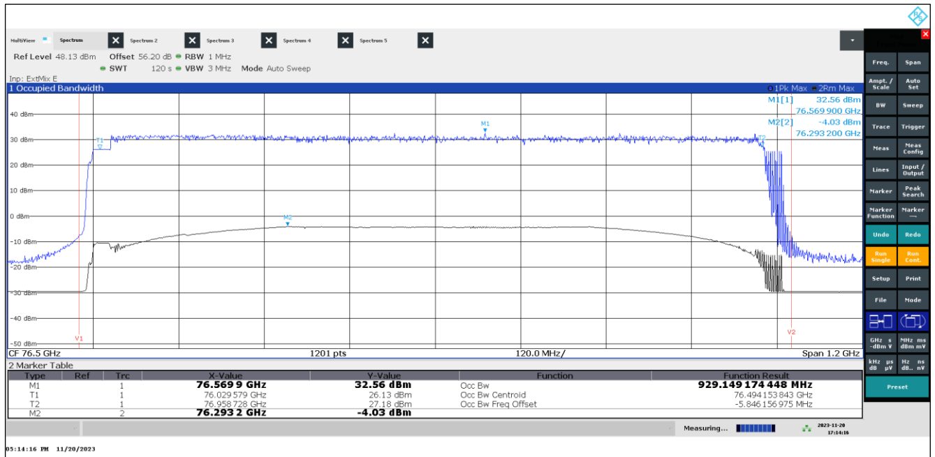
Plot 13: OBW, Mode 27, T_{\text{nom}} / V_{\text{min-max}}
