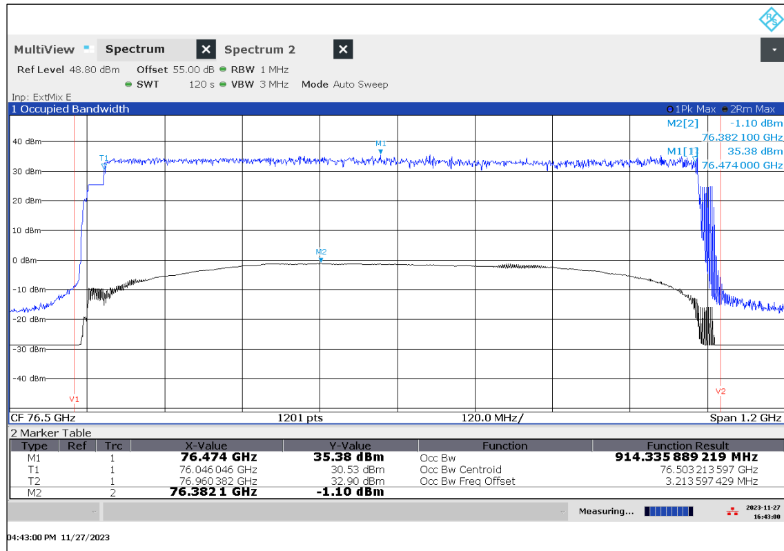
Plot 78: Mode 09, OBW, -10 °C / V_{\min-max}
