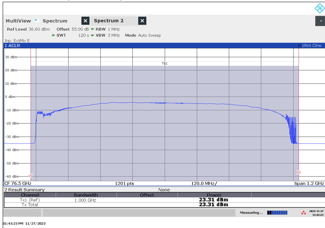
Plot 41: EIRP Mean Power (Channel Power), Mode 27, RMS detector, T_{\text{min}} / V_{\text{min-max}}
