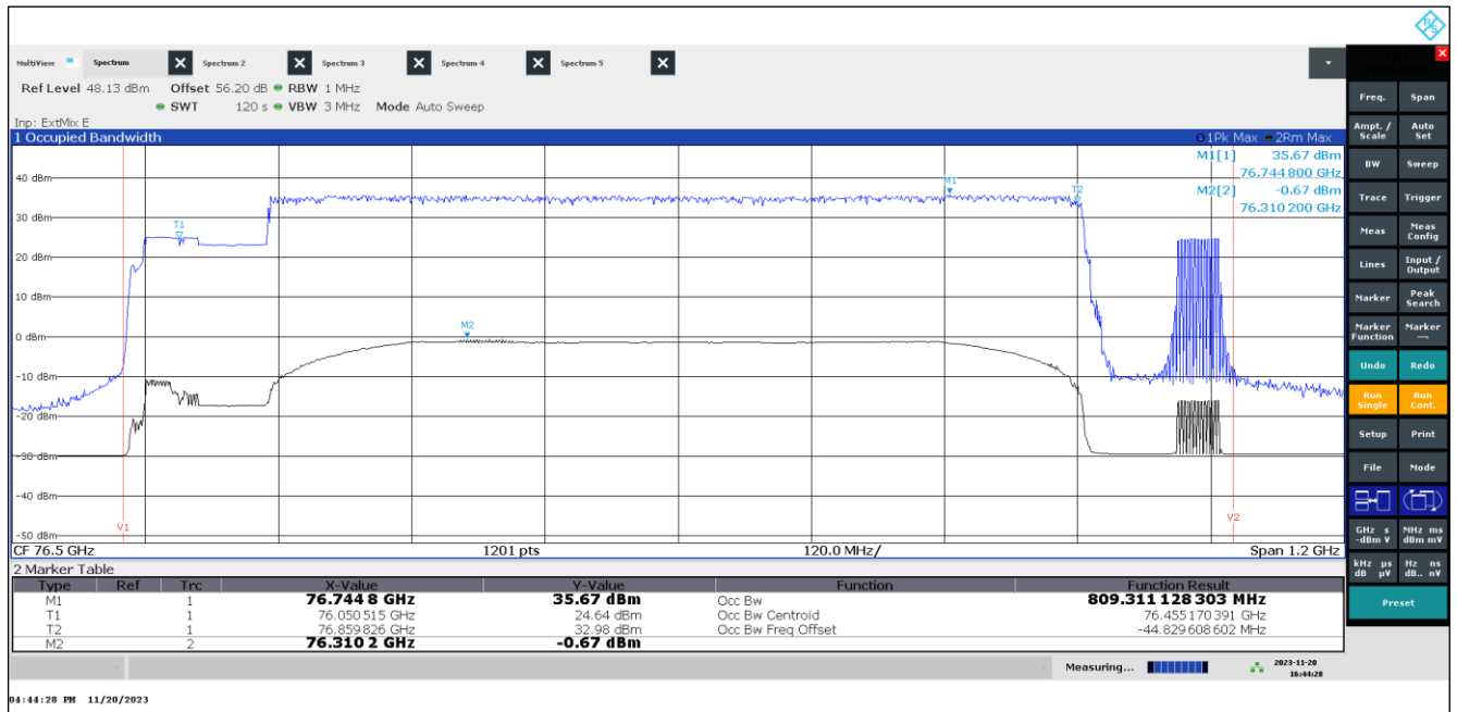
Plot 7: OBW, Mode 15, T_{\text{nom}} / V_{\text{min-max}}
