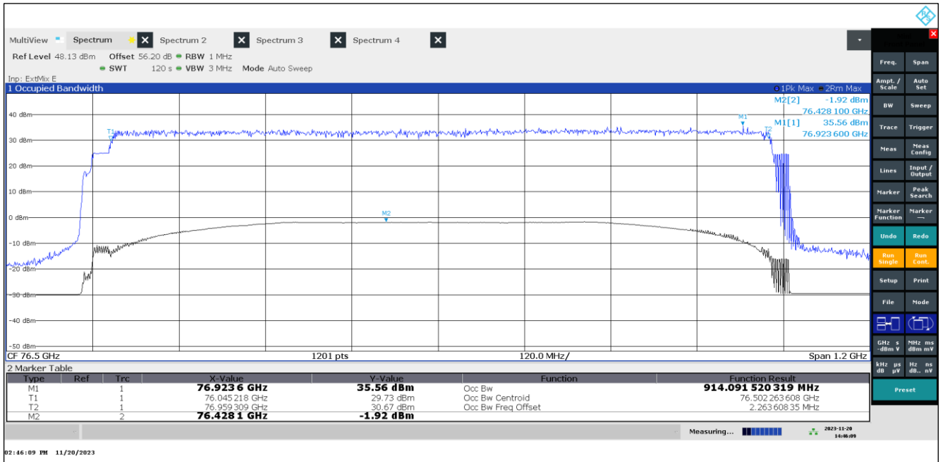
Plot 1: OBW, Mode 03, T_{\text{nom}} / V_{\text{min-max}}
