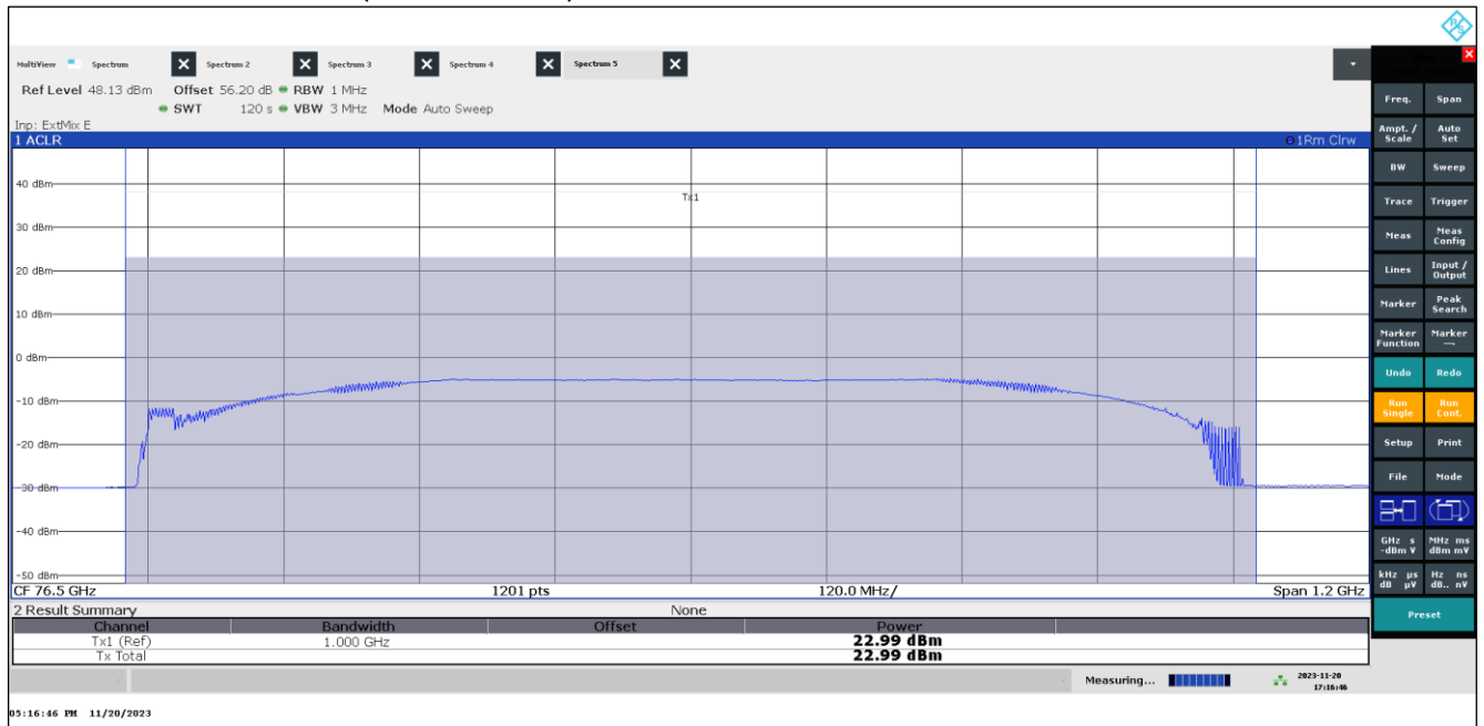
Plot 40: EIRP Mean Power (Channel Power), Mode 27, RMS detector, T_{\text{nom}} / V_{\text{min-max}}
