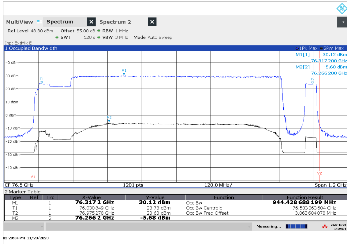
Plot 21: OBW, Mode 51, T_{\max} / V_{\min-\max}
