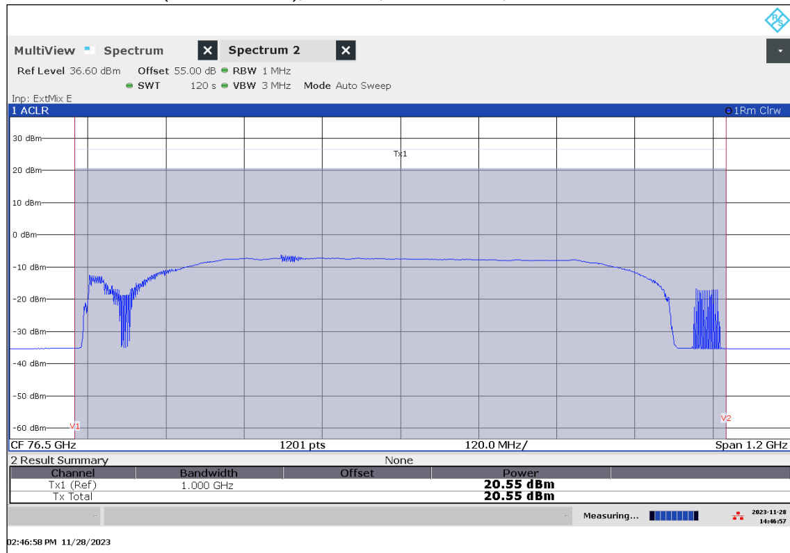
Plot 51: EIRP Mean Power (Channel Power), Mode 63, RMS detector, T_{\max} / V_{\min-\max}
