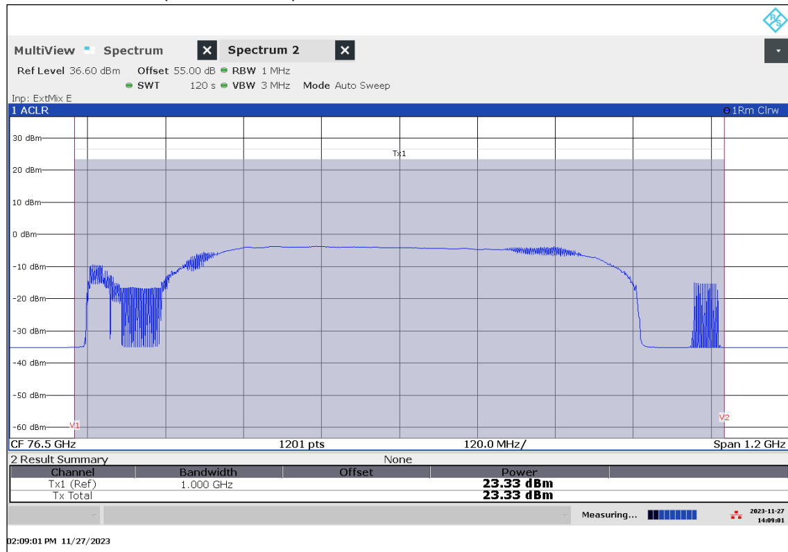
Plot 47: EIRP Mean Power (Channel Power), Mode 51, RMS detector, T_{\text{min}} / V_{\text{min-max}}
