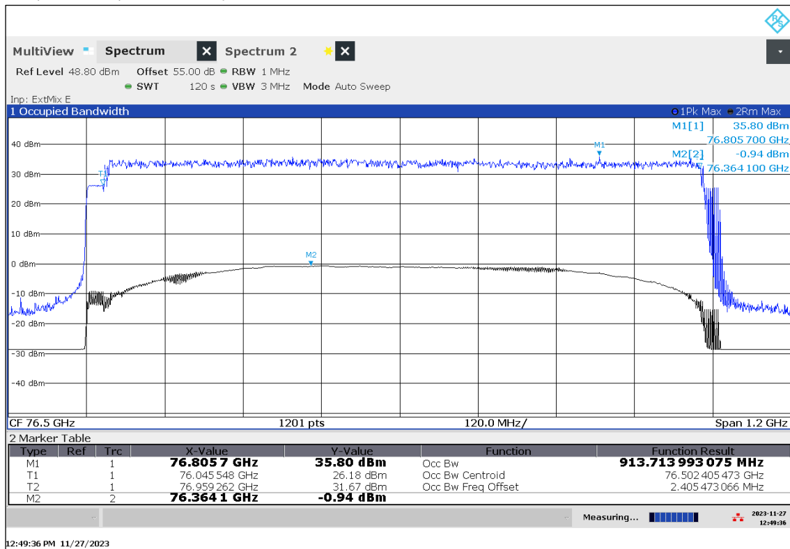
Plot 2: OBW, Mode 03, T_{\text{min}} / V_{\text{min-max}}
