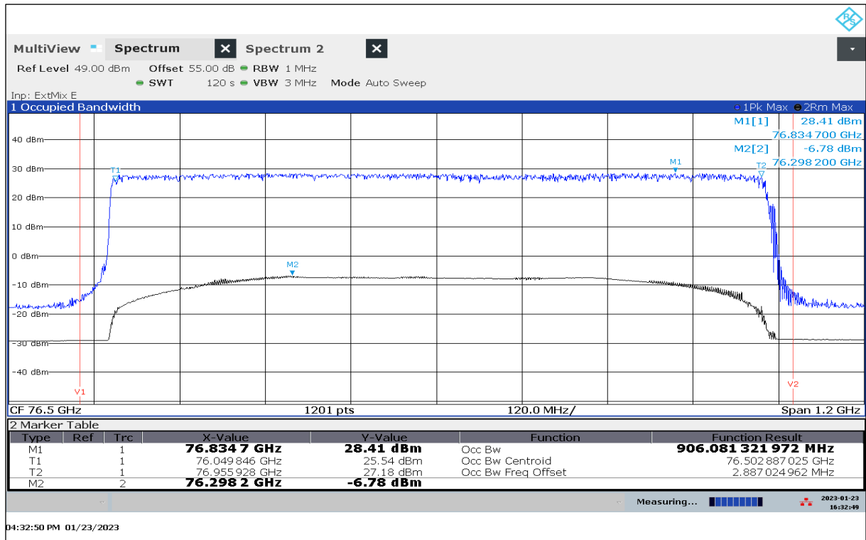
Plot 13: OBW, Mode 27, T_{\text{nom}} / V_{\text{min-max}}
