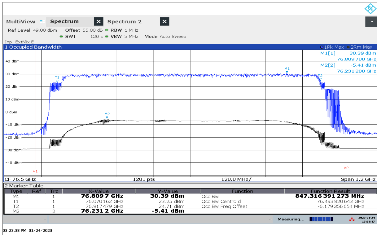
Plot 24: OBW, Mode 63, T_{\max} / V_{\min-\max}
