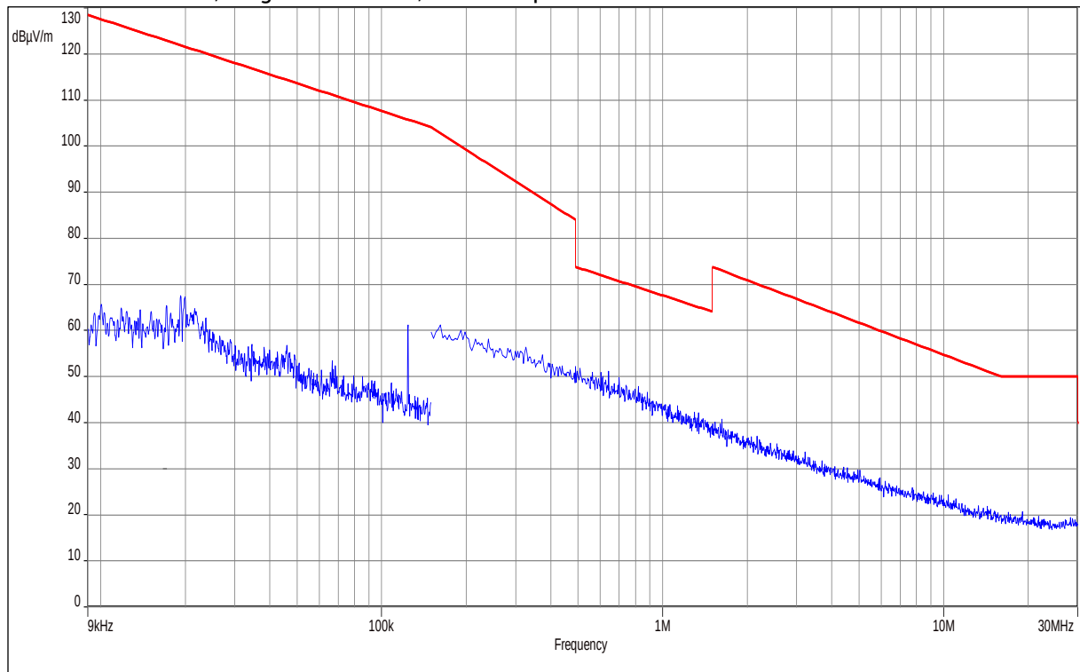
Plot 55: 9 kHz – 30 MHz, Magnetic antenna, valid for specified modes
