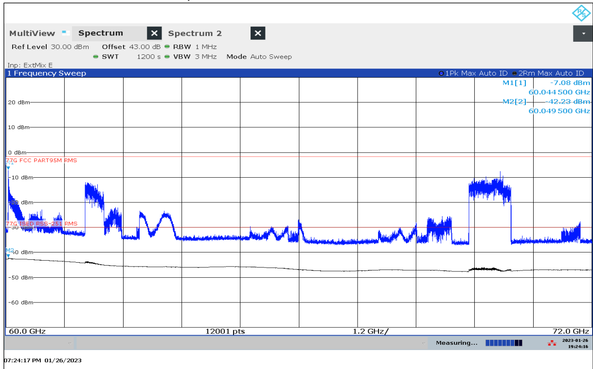
Plot 63: 60 GHz – 72 GHz, valid for specified modes, antenna vertical / horizontal
