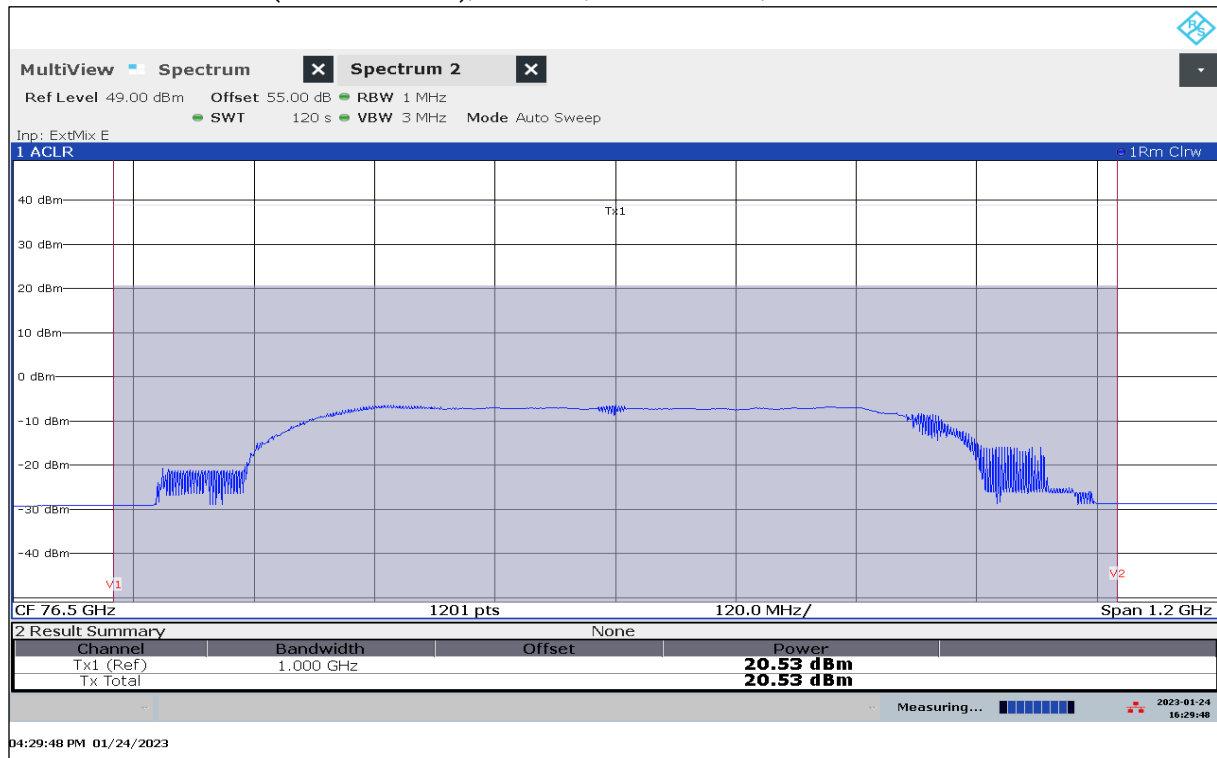
Plot 48: EIRP Mean Power (Channel Power), Mode 51, RMS detector, T_{\max} / V_{\min-\max}
