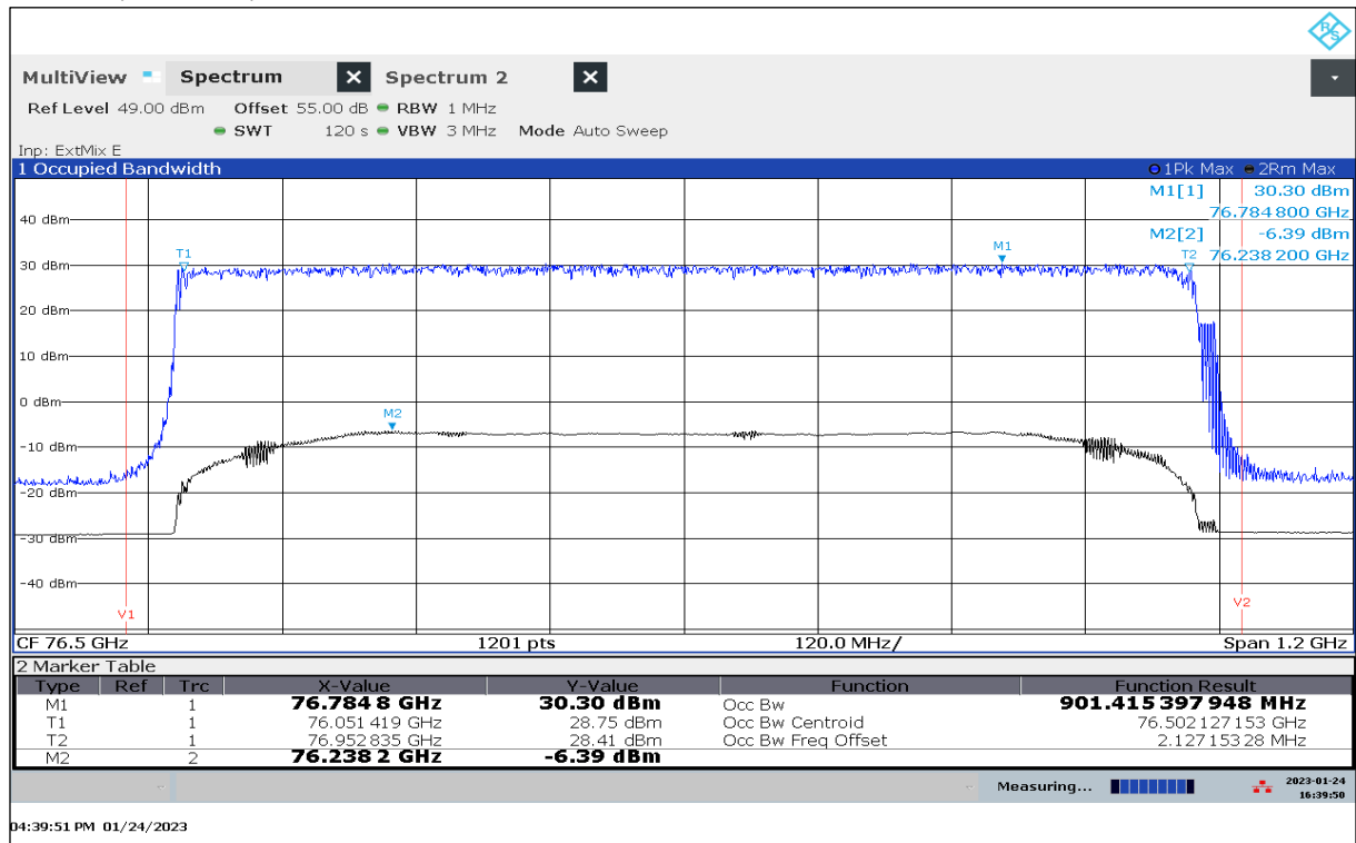
Plot 18: OBW, Mode 39, T_{\max} / V_{\min-\max}
