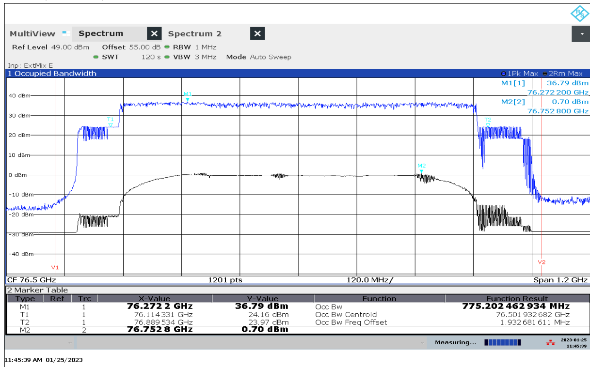
Plot 8: OBW, Mode 15, T_{\text{min}} / V_{\text{min-max}}
