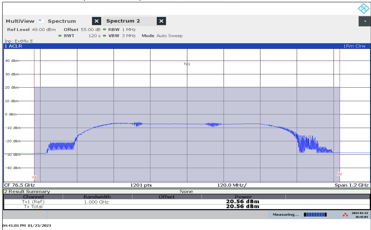
Plot 46: EIRP Mean Power (Channel Power), Mode 51, RMS detector, T_{\text{nom}} / V_{\min-\max}
