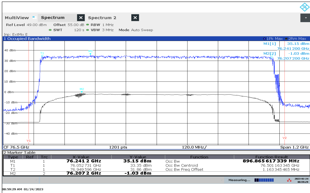
Plot 86: Mode 09, OBW, 85 °C / V min-max
