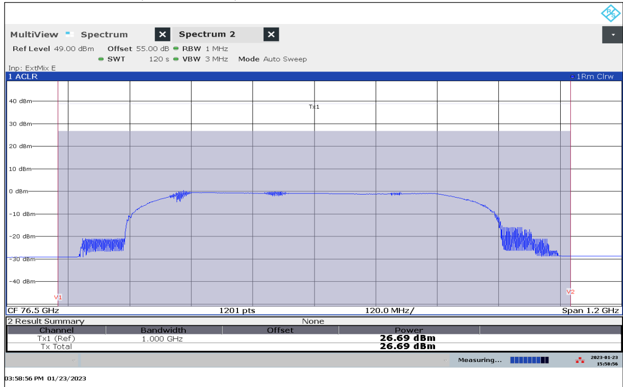
Plot 34: EIRP Mean Power (Channel Power), Mode 15, RMS detector, T_{\text{nom}} / V_{\min-\max}
