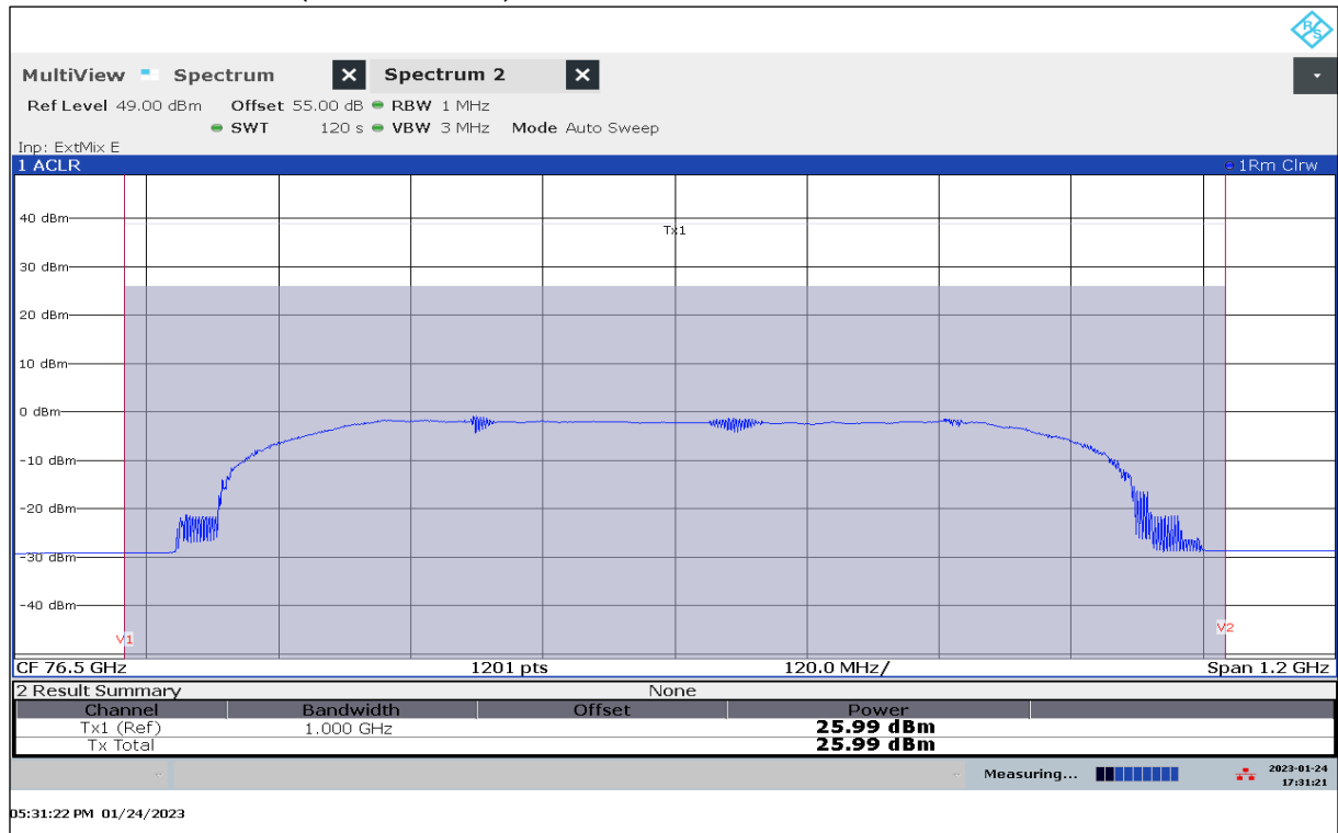
Plot 39: EIRP Mean Power (Channel Power), Mode 21, RMS detector, T_{\max} / V_{\min-\max}
