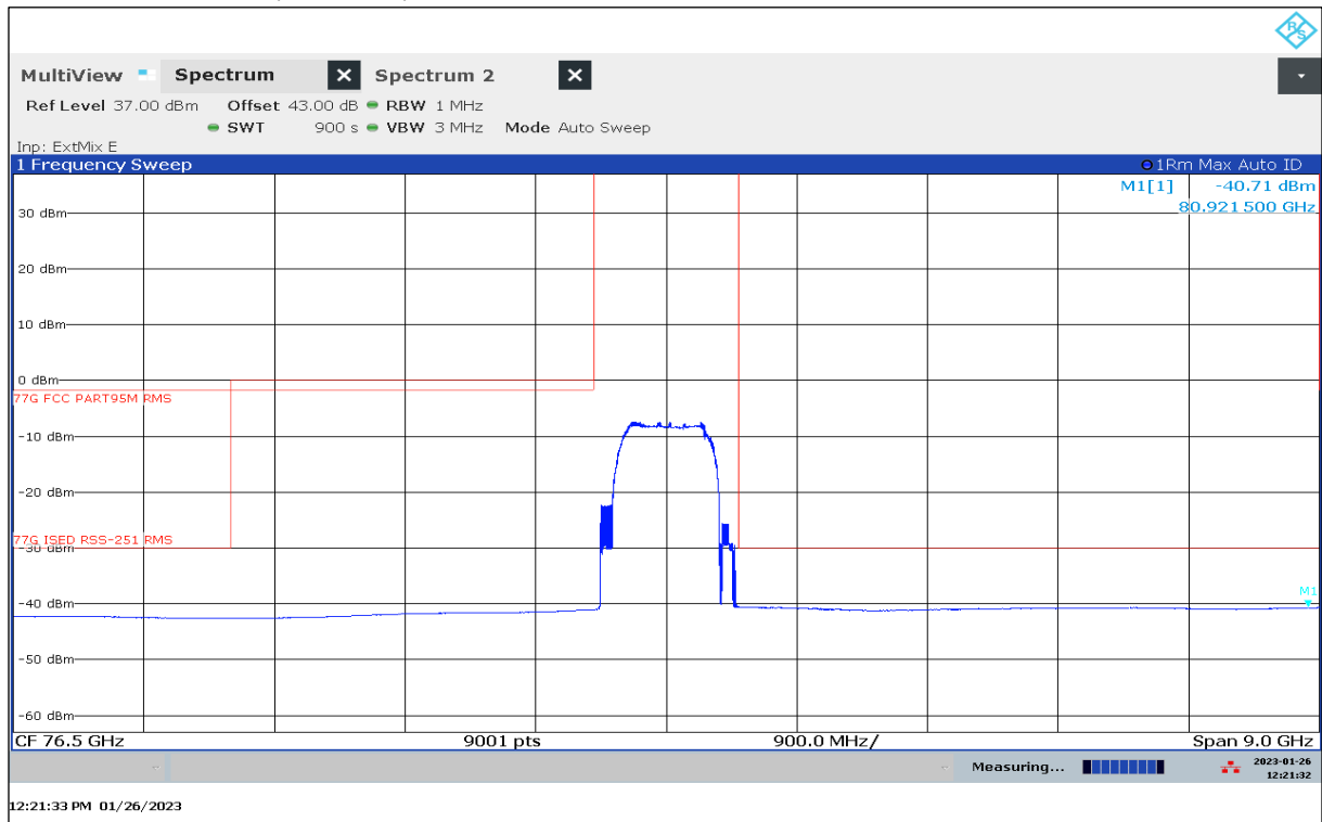
Plot 70: 72 GHz – 81 GHz, Mode 51, antenna vertical / horizontal
