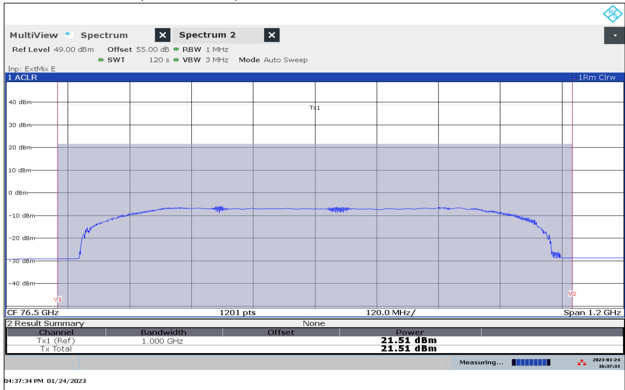
Plot 45: EIRP Mean Power (Channel Power), Mode 39, RMS detector, T_{\max} / V_{\min-\max}
