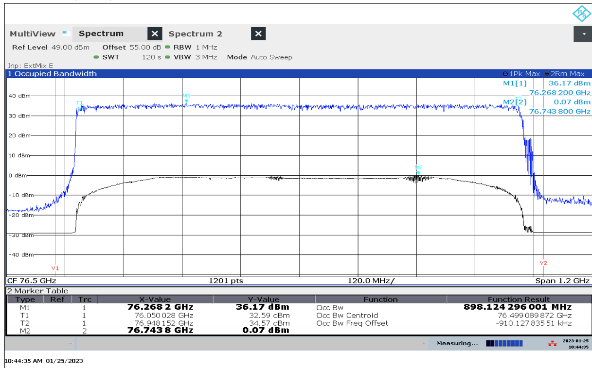
Plot 78: Mode 09, OBW, -20 °C / V min-max
