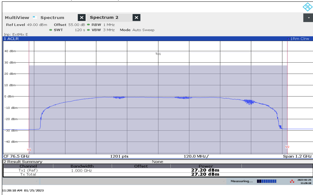
Plot 29: EIRP Mean Power (Channel Power), Mode 03, RMS detector, T_{\min} / V_{\min-max}
