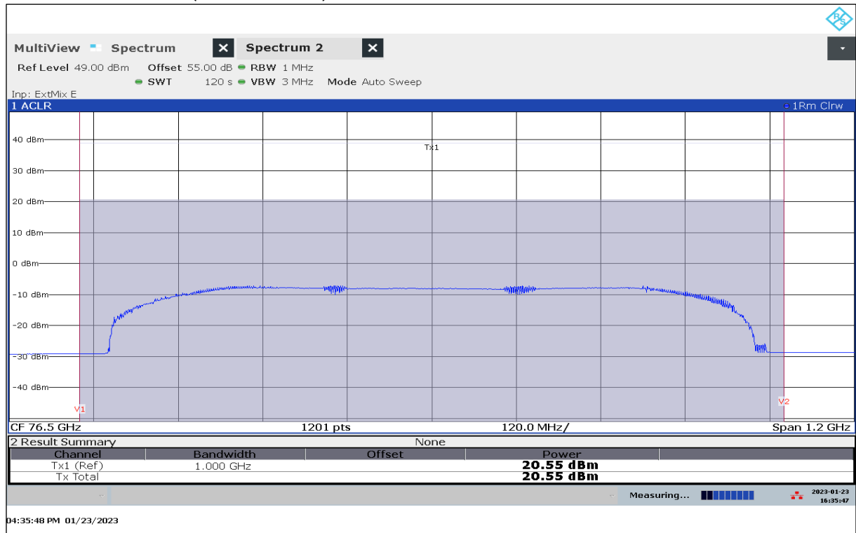
Plot 43: EIRP Mean Power (Channel Power), Mode 39, RMS detector, T_{\text{nom}} / V_{\text{min-max}}
