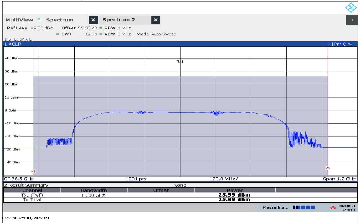
Plot 36: EIRP Mean Power (Channel Power), Mode 15, RMS detector, T_{\max} / V_{\min-\max}
