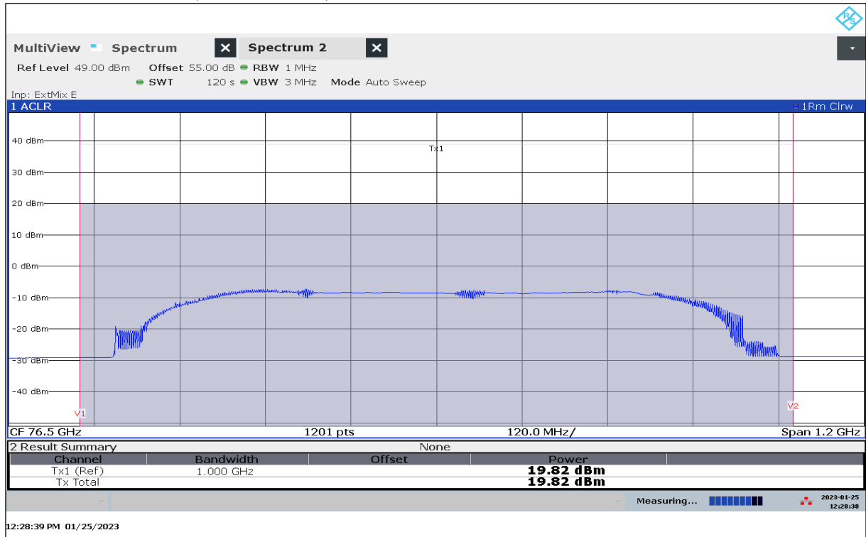
Plot 50: EIRP Mean Power (Channel Power), Mode 63, RMS detector, T_{\text{min}} / V_{\text{min-max}}
