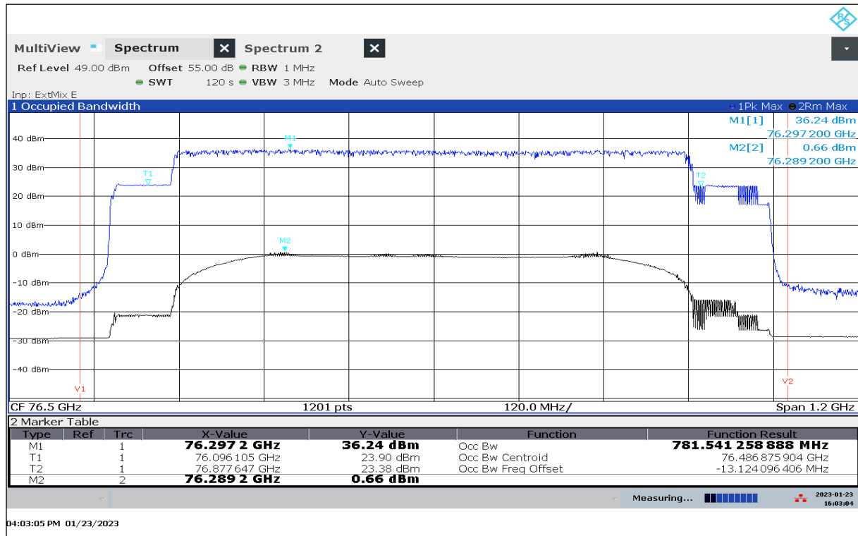
Plot 7: OBW, Mode 15, T_{\text{nom}} / V_{\text{min-max}}
