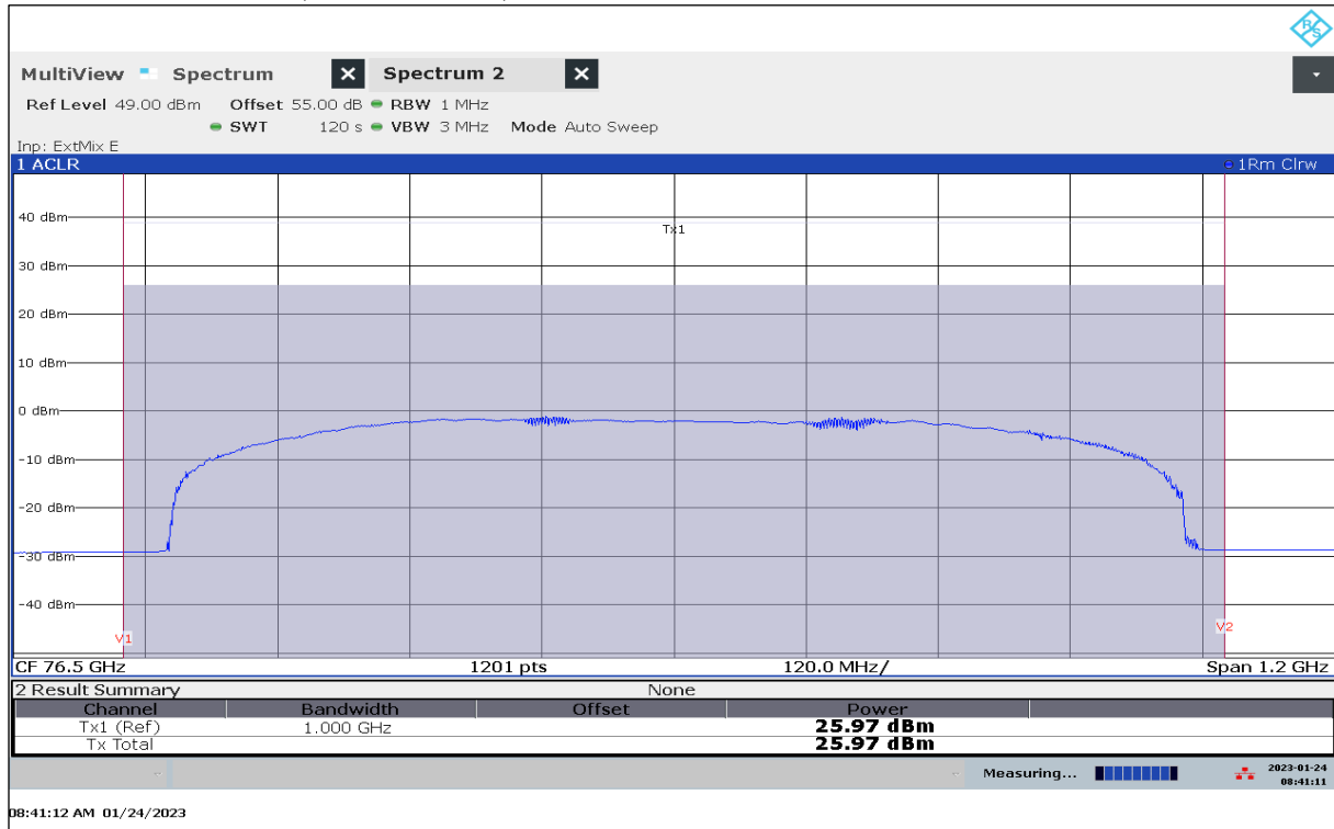
Plot 30: EIRP Mean Power (Channel Power), Mode 03, RMS detector, T_{\max} / V_{\min-max}
