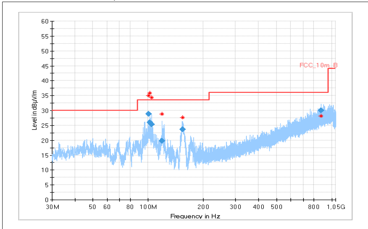
Plot 56: 30 MHz – 1 GHz, valid for specified modes, antenna vertical / horizontal
