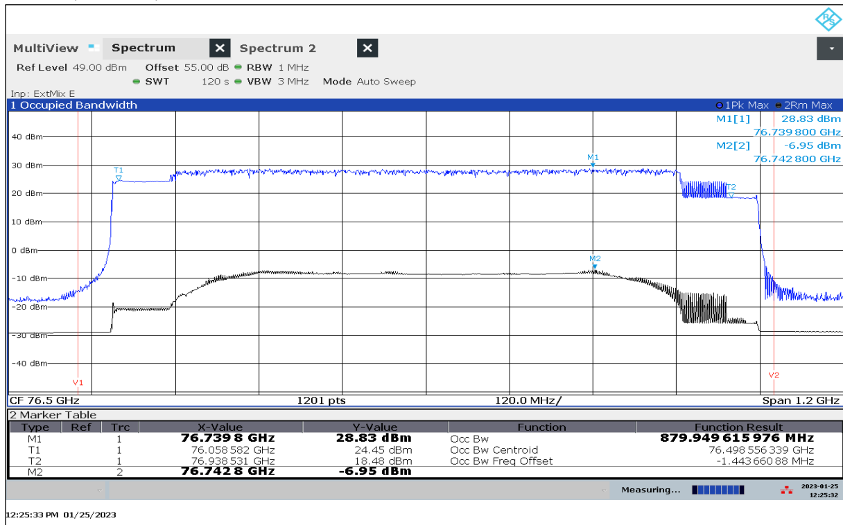
Plot 20: OBW, Mode 51, T_{\text{min}} / V_{\text{min-max}}
