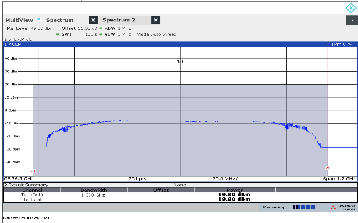
Plot 41: EIRP Mean Power (Channel Power), Mode 27, RMS detector, T_{\min} / V_{\min-\max}
