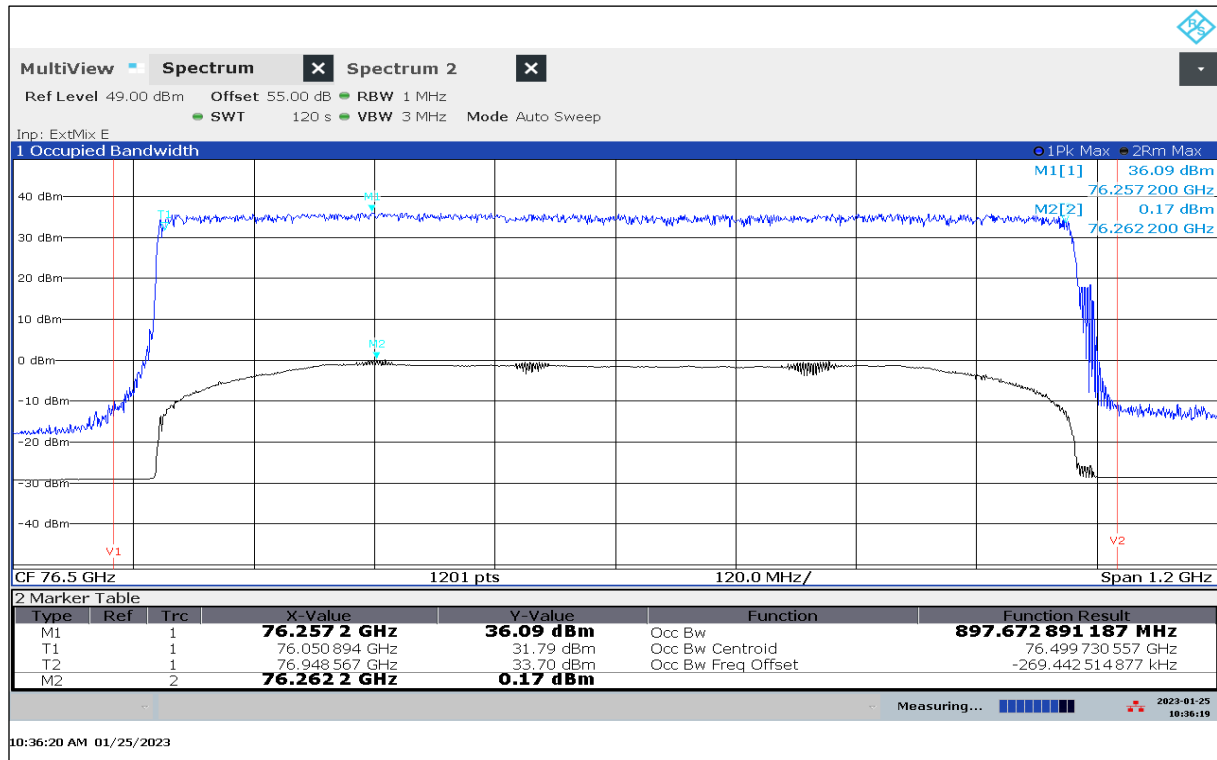
Plot 79: Mode 09, OBW, -10 °C / V min-max
