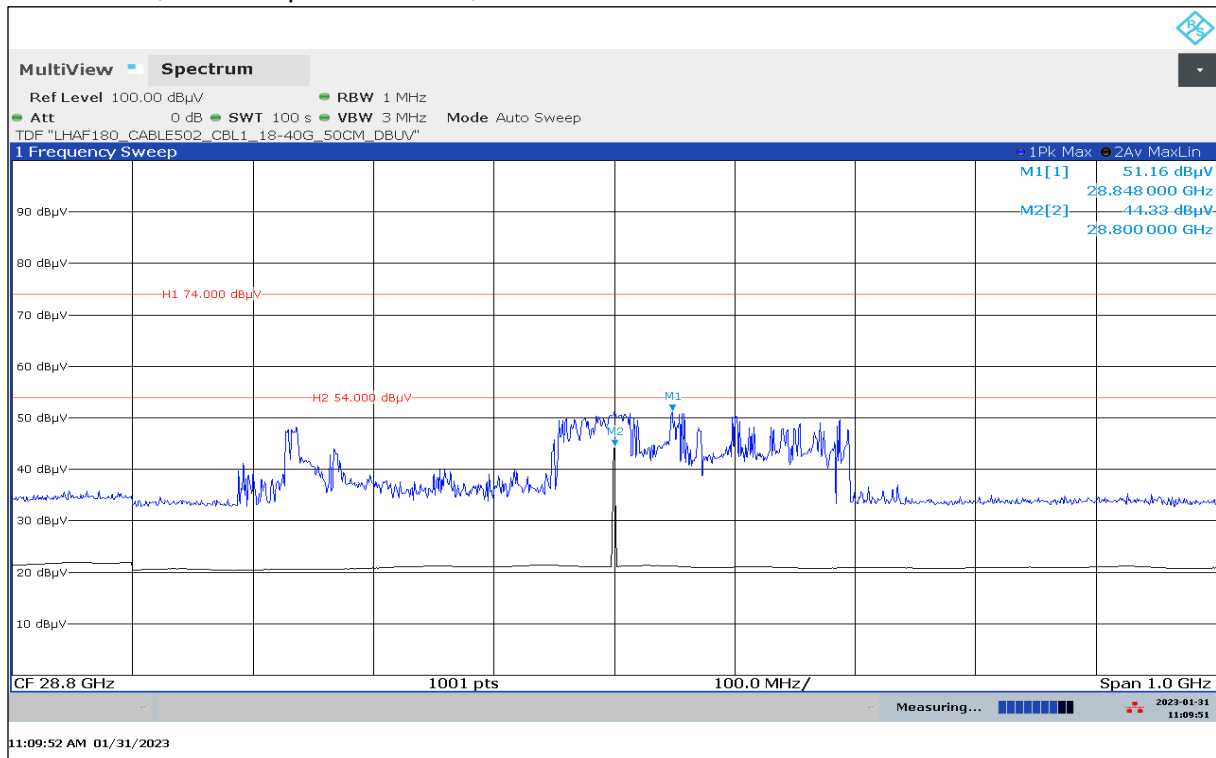
Plot 60: 28.8 GHz, valid for specified modes, antenna vertical / horizontal
