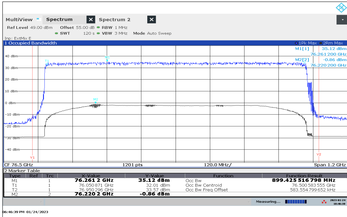
Plot 83: Mode 09, OBW, 30 °C / V min-max
