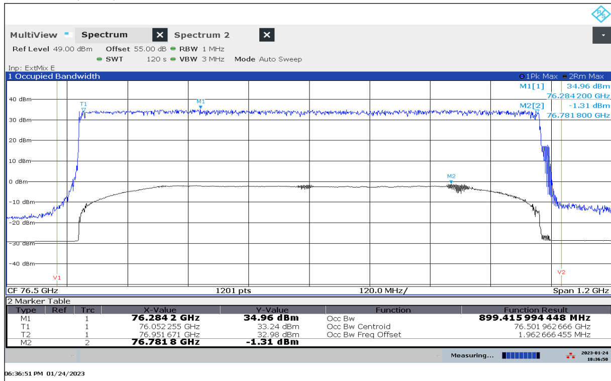
Plot 84: Mode 09, OBW, 40 °C / V min-max
