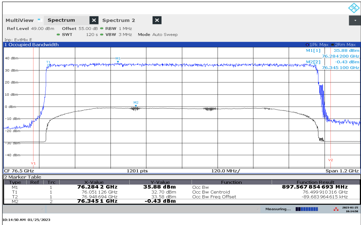
Plot 81: Mode 09, OBW, 10 °C / V min-max
