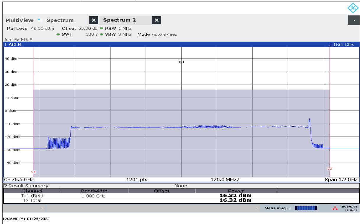
Plot 53: EIRP Mean Power (Channel Power), Mode 80, RMS detector, T_{\min} / V_{\min-max}
