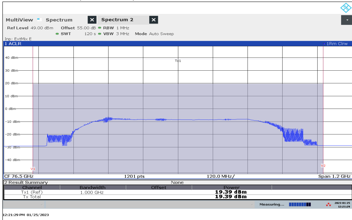
Plot 47: EIRP Mean Power (Channel Power), Mode 51, RMS detector, T_{\min} / V_{\min-\max}
