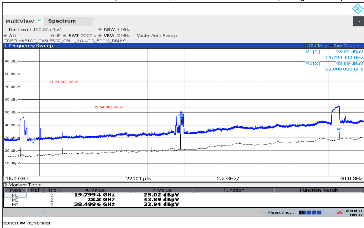
Plot 59: 18 GHz – 40 GHz, valid for specified modes, antenna vertical / horizontal (Average detector)
