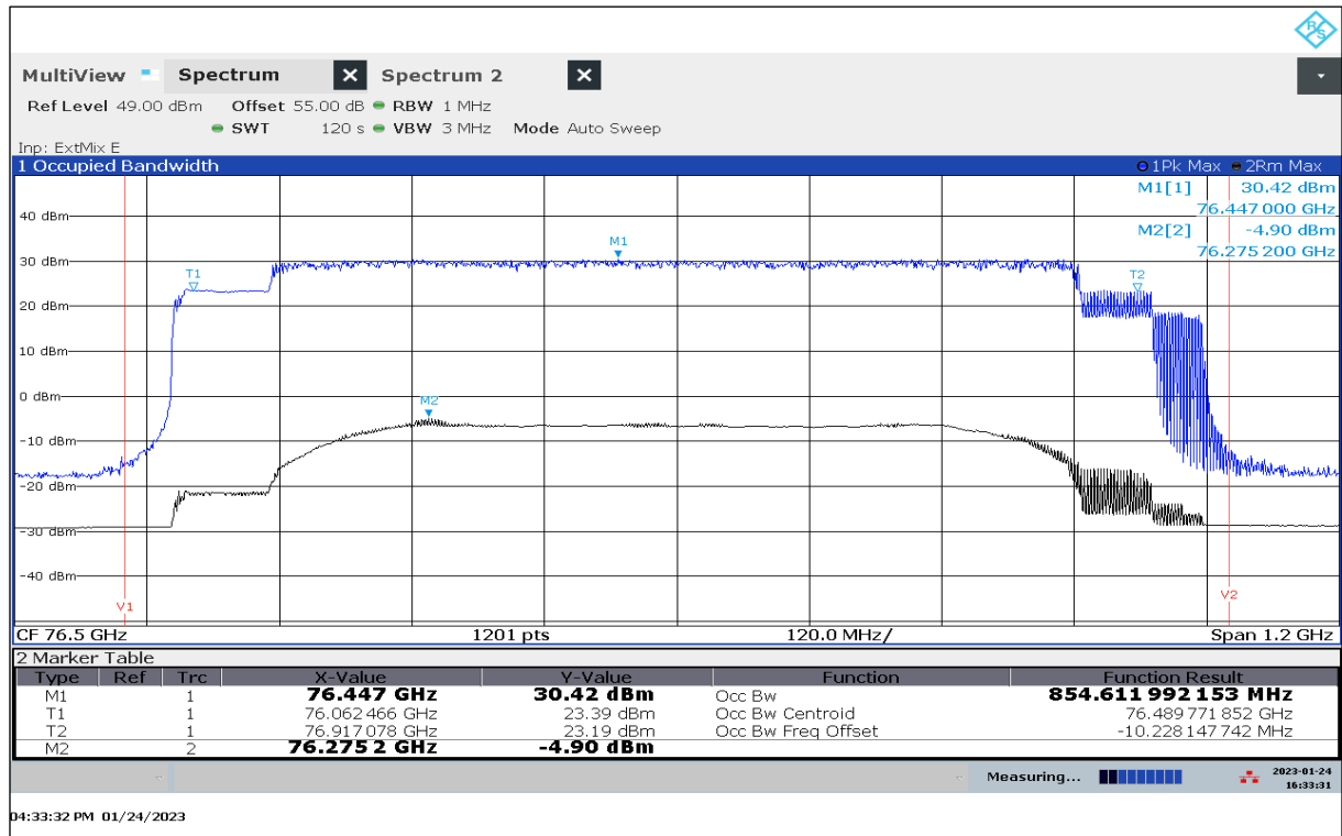
Plot 21: OBW, Mode 51, T_{\max} / V_{\min-\max}
