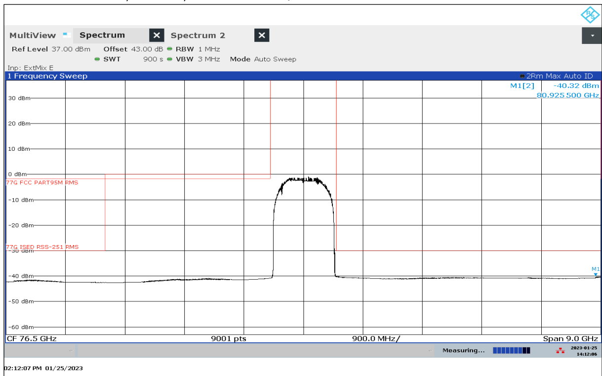
Plot 64: 72 GHz – 81 GHz, Mode 03, antenna vertical / horizontal
