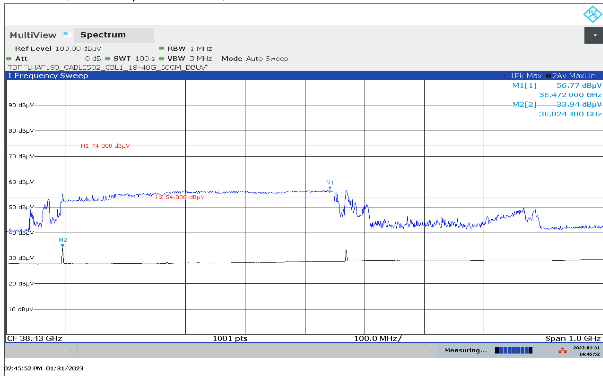
Plot 61: 38 GHz, valid for specified modes, antenna vertical / horizontal
