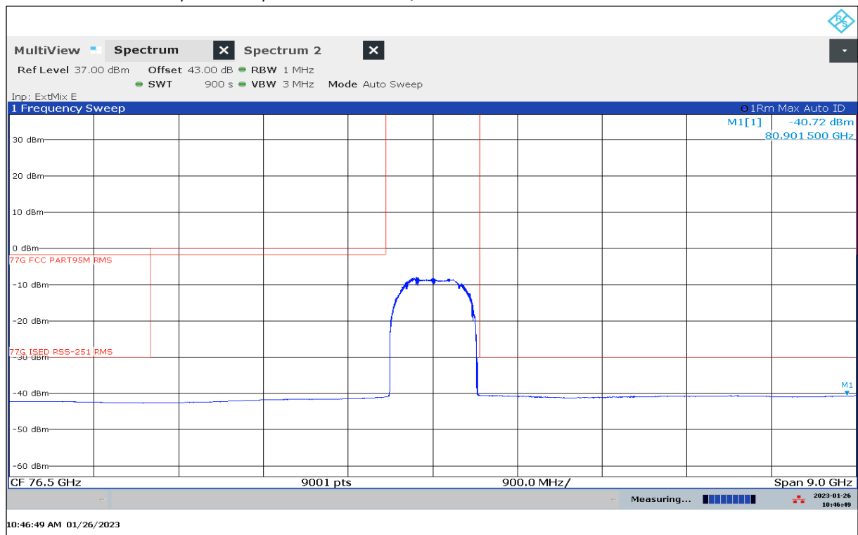
Plot 68: 72 GHz – 81 GHz, Mode 27, antenna vertical / horizontal
