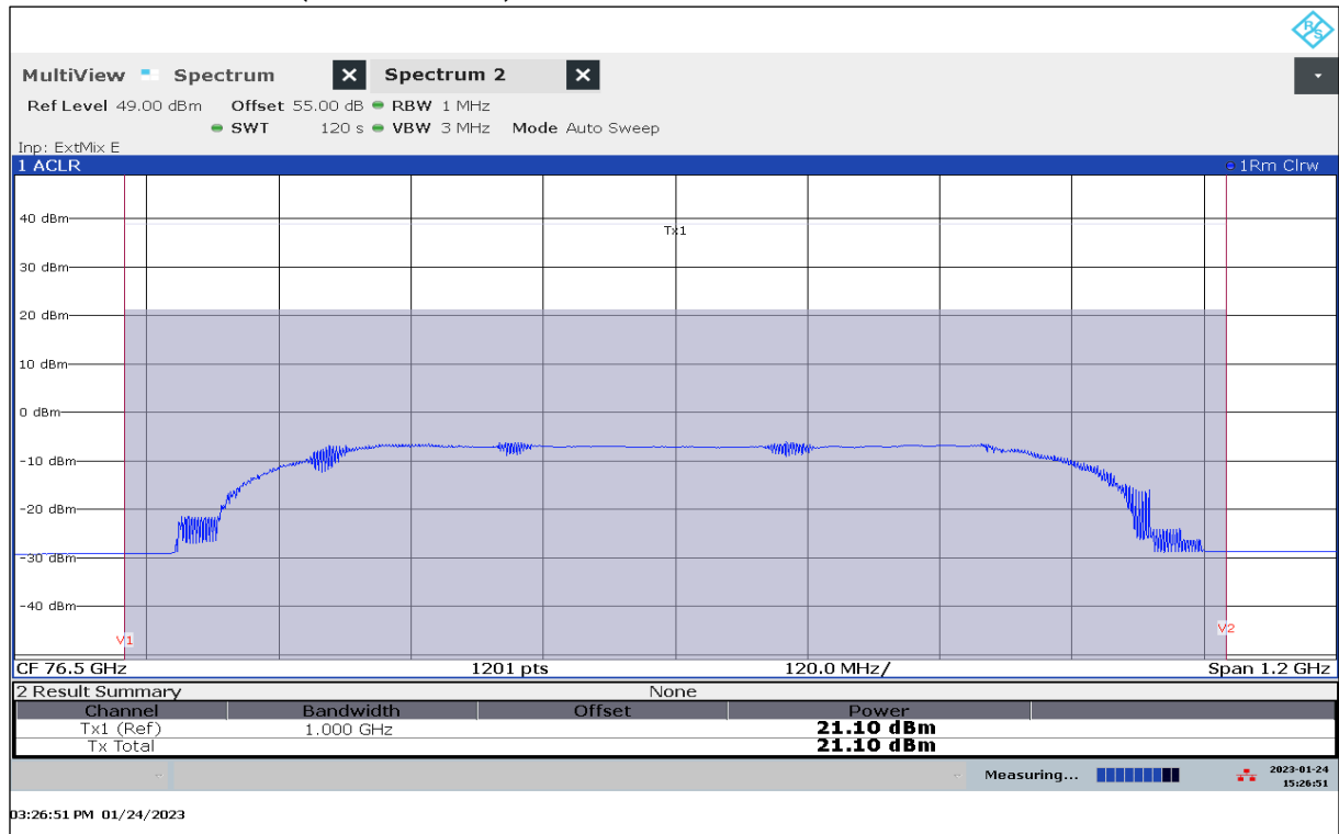
Plot 51: EIRP Mean Power (Channel Power), Mode 63, RMS detector, T_{\max} / V_{\min-\max}
