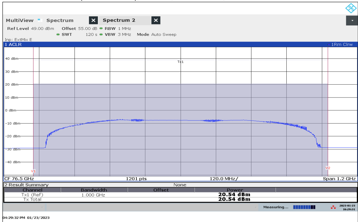
Plot 40: EIRP Mean Power (Channel Power), Mode 27, RMS detector, T_{\text{nom}} / V_{\min-\max}
