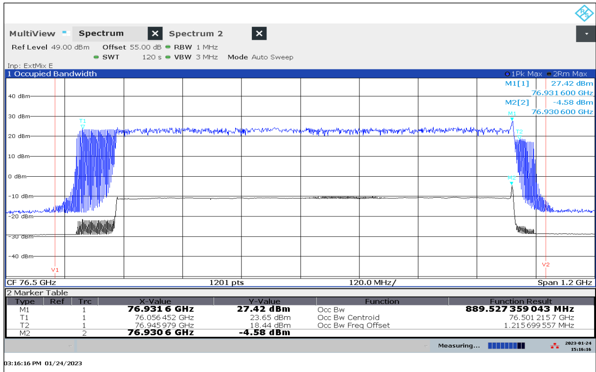
Plot 27: OBW, Mode 80, T_{\max} / V_{\min-\max}
