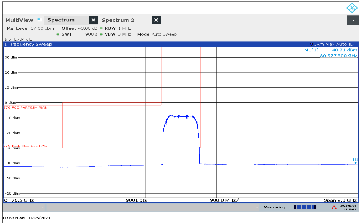
Plot 69: 72 GHz – 81 GHz, Mode 39, antenna vertical / horizontal
