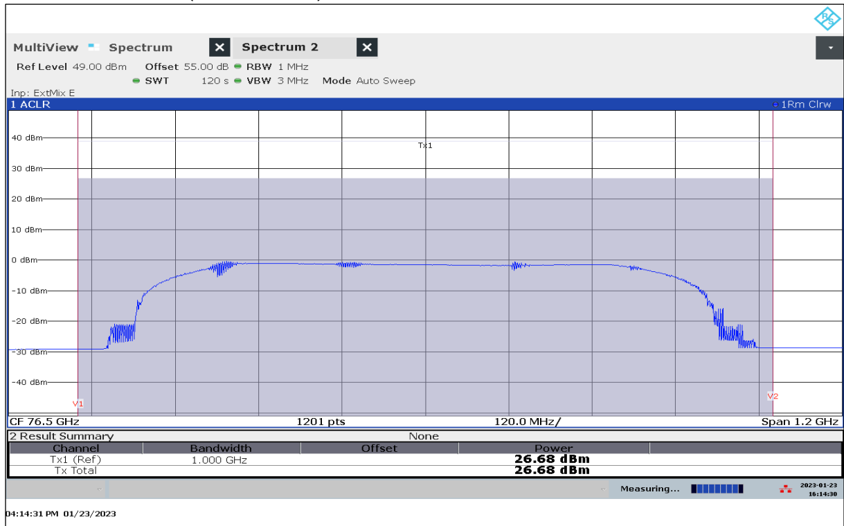
Plot 37: EIRP Mean Power (Channel Power), Mode 21, RMS detector, T_{\text{nom}} / V_{\text{min-max}}
