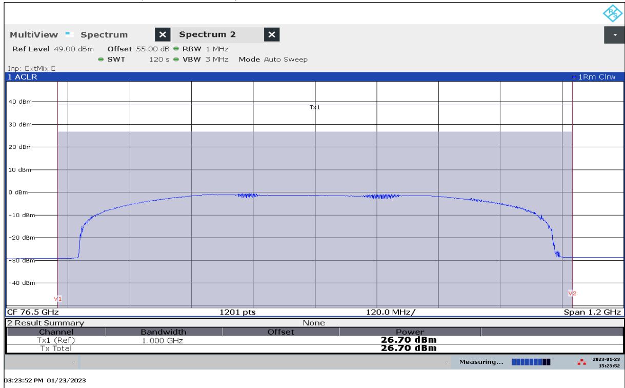
Plot 28: EIRP Mean Power (Channel Power), Mode 03, RMS detector, T_{\text{nom}} / V_{\min-\max}
