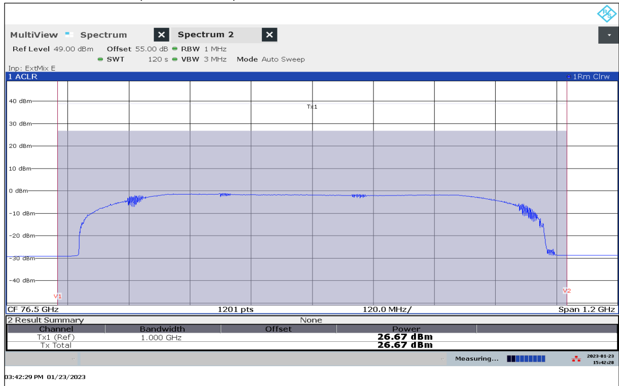
Plot 31: EIRP Mean Power (Channel Power), Mode 09, RMS detector, T_{\text{nom}} / V_{\text{min-max}}
