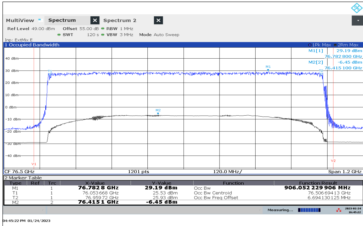
Plot 15: OBW, Mode 27, T_{\max} / V_{\min-\max}
