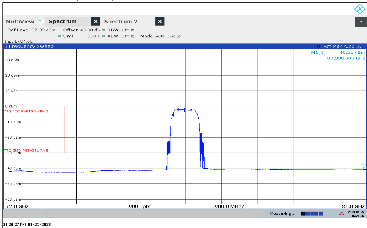
Plot 66: 72 GHz – 81 GHz, Mode 15, antenna vertical / horizontal
