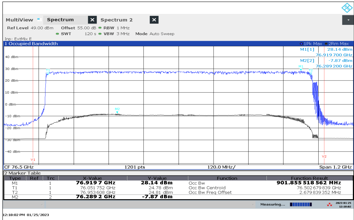
Plot 17: OBW, Mode 39, T_{\min} / V_{\min-\max}
