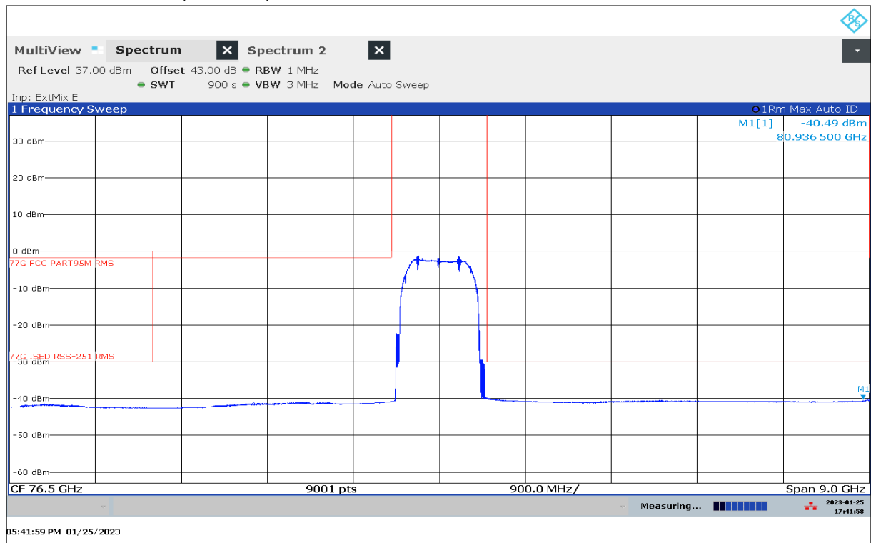
Plot 67: 72 GHz – 81 GHz, Mode 21, antenna vertical / horizontal
