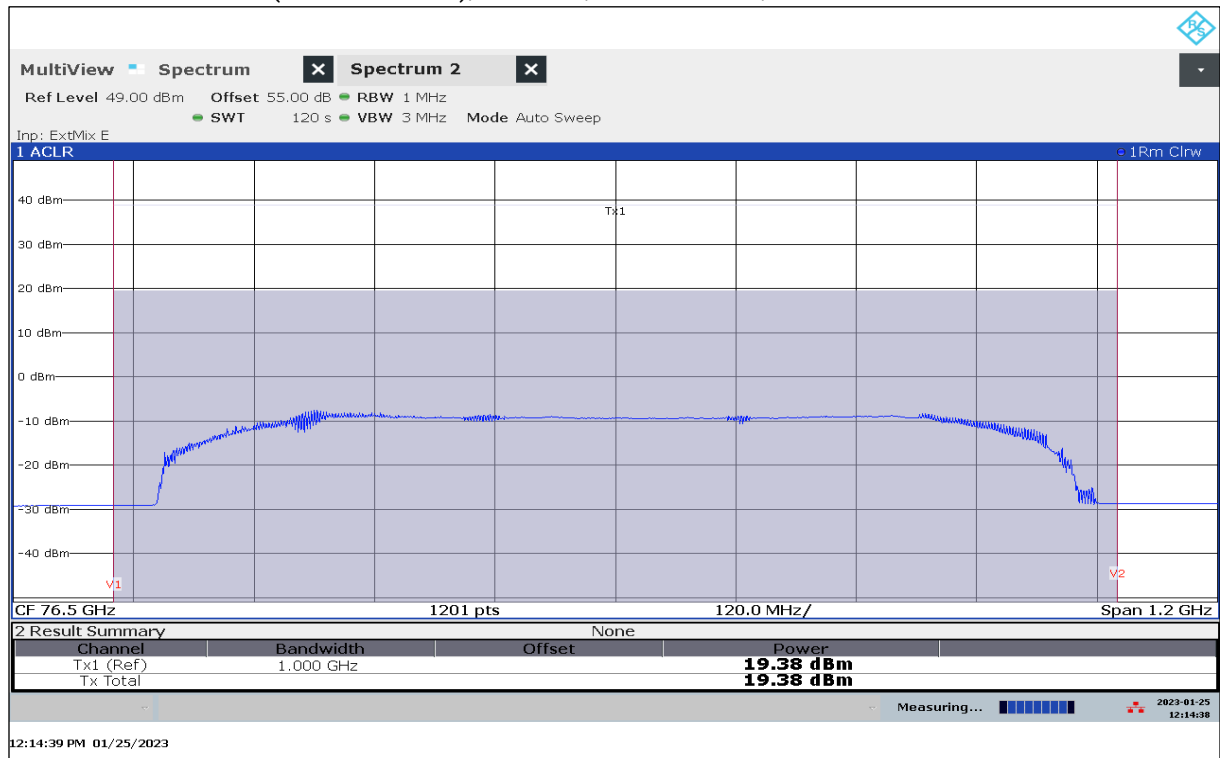
Plot 44: EIRP Mean Power (Channel Power), Mode 39, RMS detector, T_{\text{min}} / V_{\text{min-max}}
