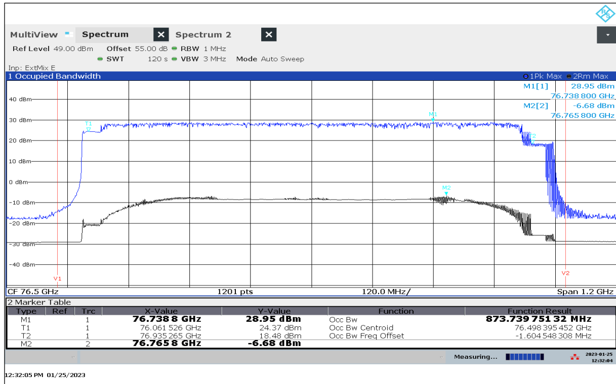
Plot 23: OBW, Mode 63, T_{\min} / V_{\min-\max}
