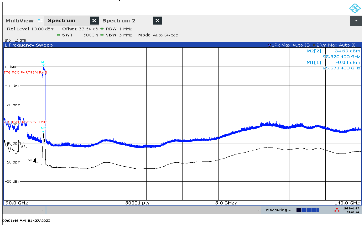
Plot 74: 90 GHz – 140 GHz, valid for specified modes, antenna vertical / horizontal
