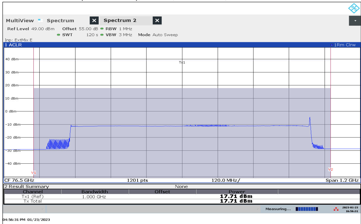
Plot 52: EIRP Mean Power (Channel Power), Mode 80, RMS detector, T_{\text{nom}} / V_{\min-\max}
