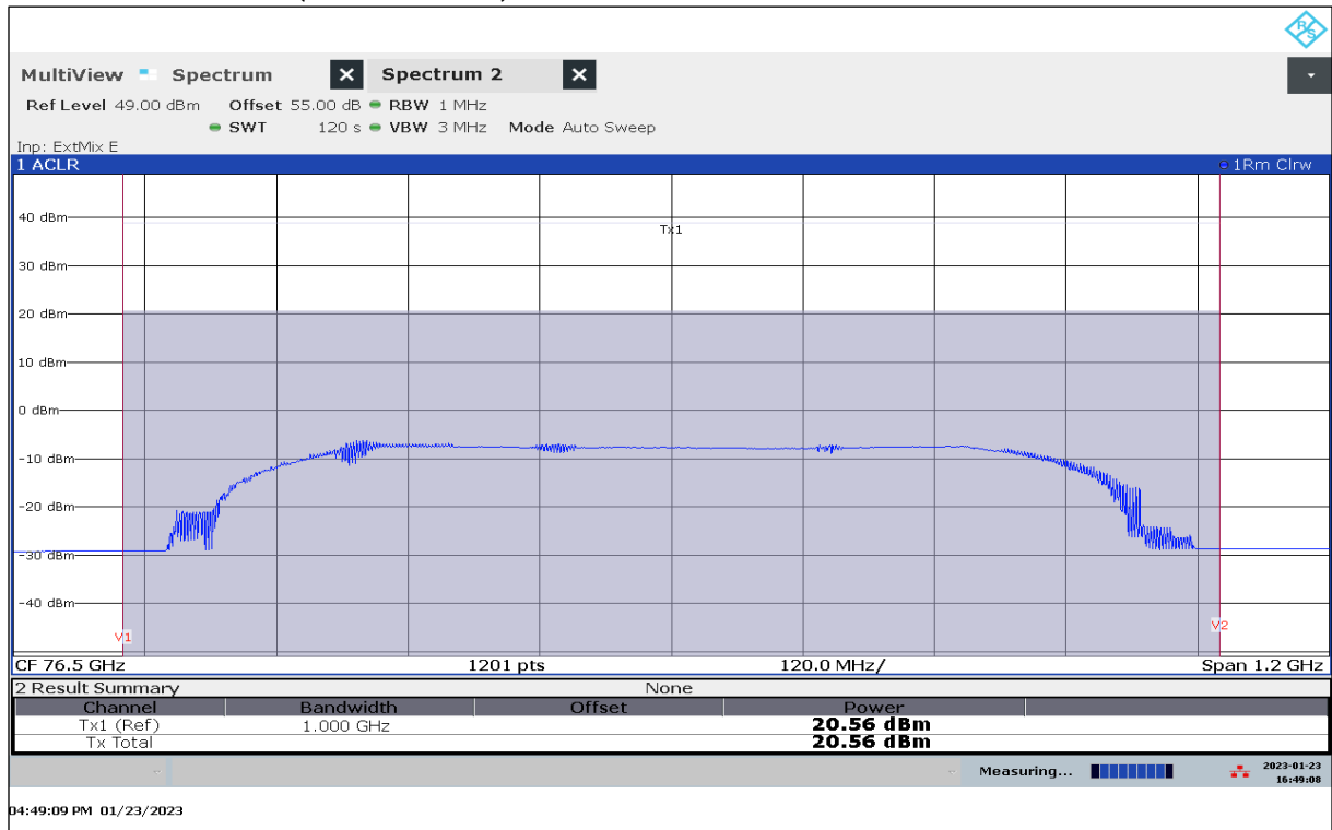
Plot 49: EIRP Mean Power (Channel Power), Mode 63, RMS detector, T_{\text{nom}} / V_{\text{min-max}}
