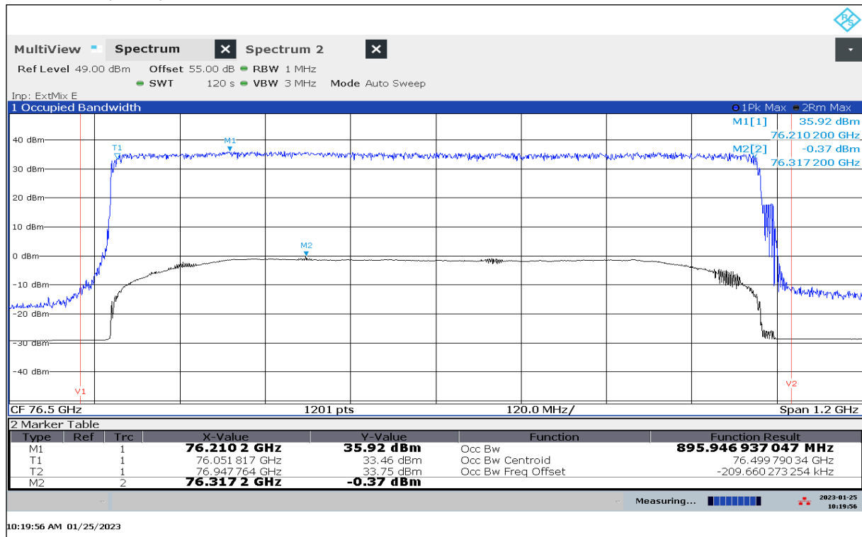
Plot 80: Mode 09, OBW, 0 °C / V min-max
