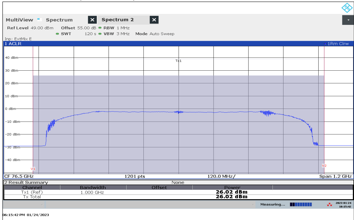
Plot 33: EIRP Mean Power (Channel Power), Mode 09, RMS detector, T_{\max} / V_{\min-\max}
