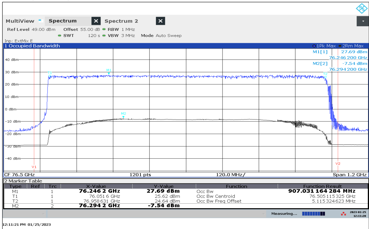
Plot 14: OBW, Mode 27, T_{\text{min}} / V_{\text{min-max}}
