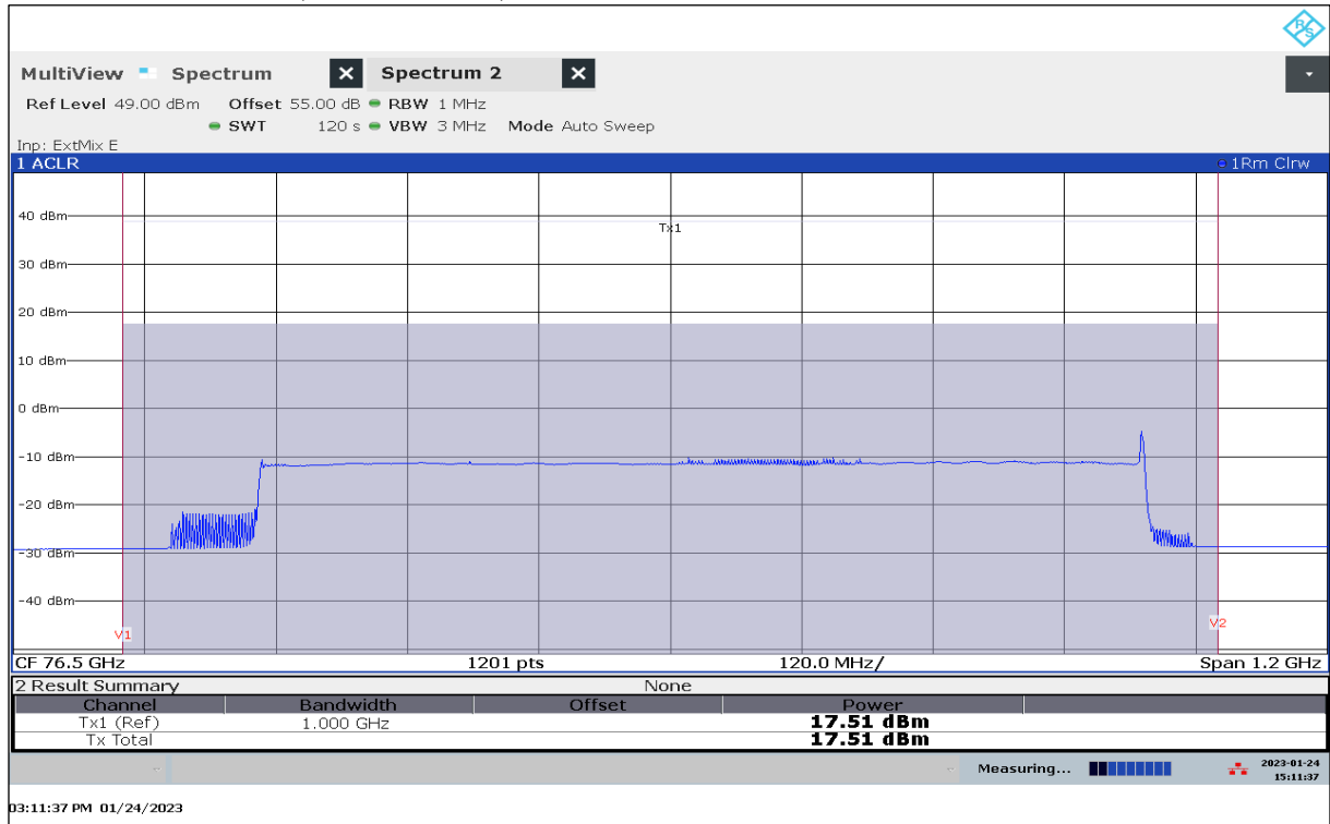
Plot 54: EIRP Mean Power (Channel Power), Mode 80, RMS detector, T_{\max} / V_{\min-max}
