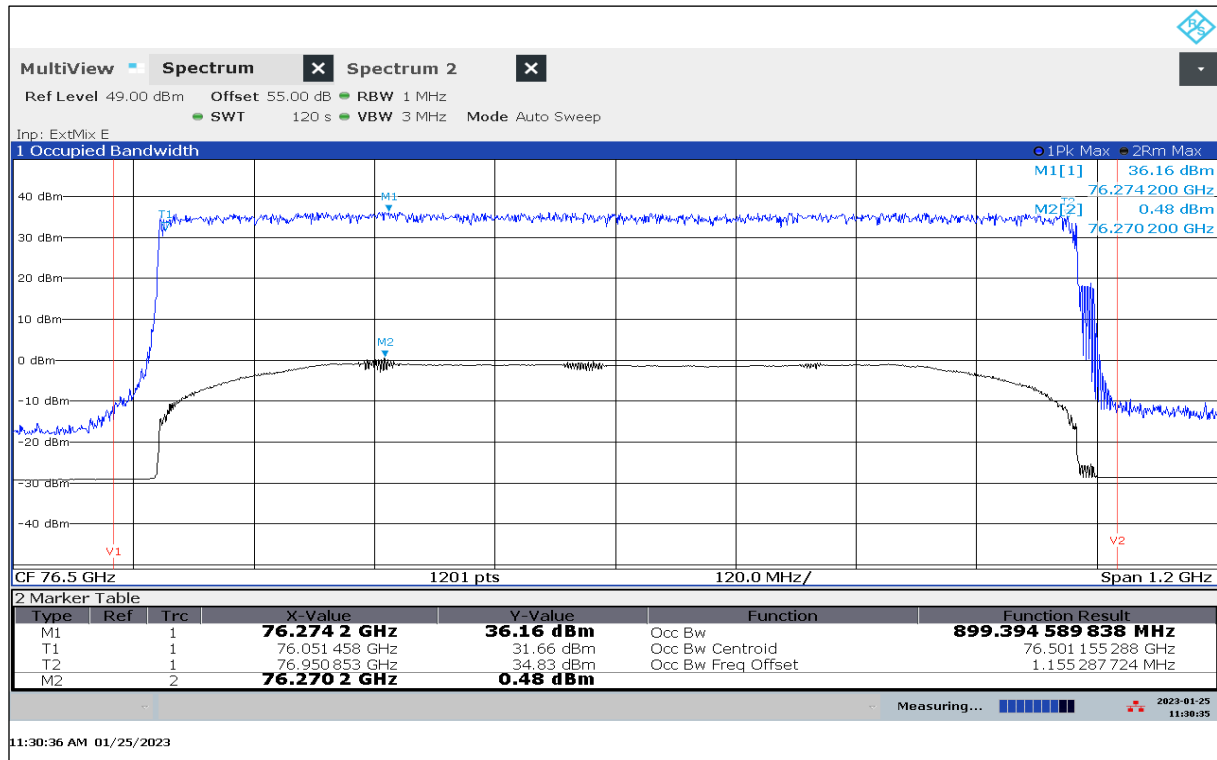
Plot 77: Mode 09, OBW, -40 °C / V min-max
