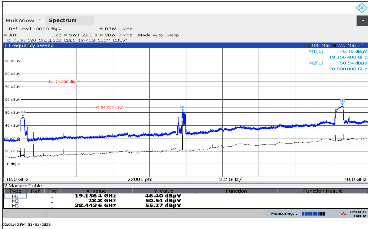
Plot 58: 18 GHz – 40 GHz, valid for specified modes, antenna vertical / horizontal (PEAK detector)
