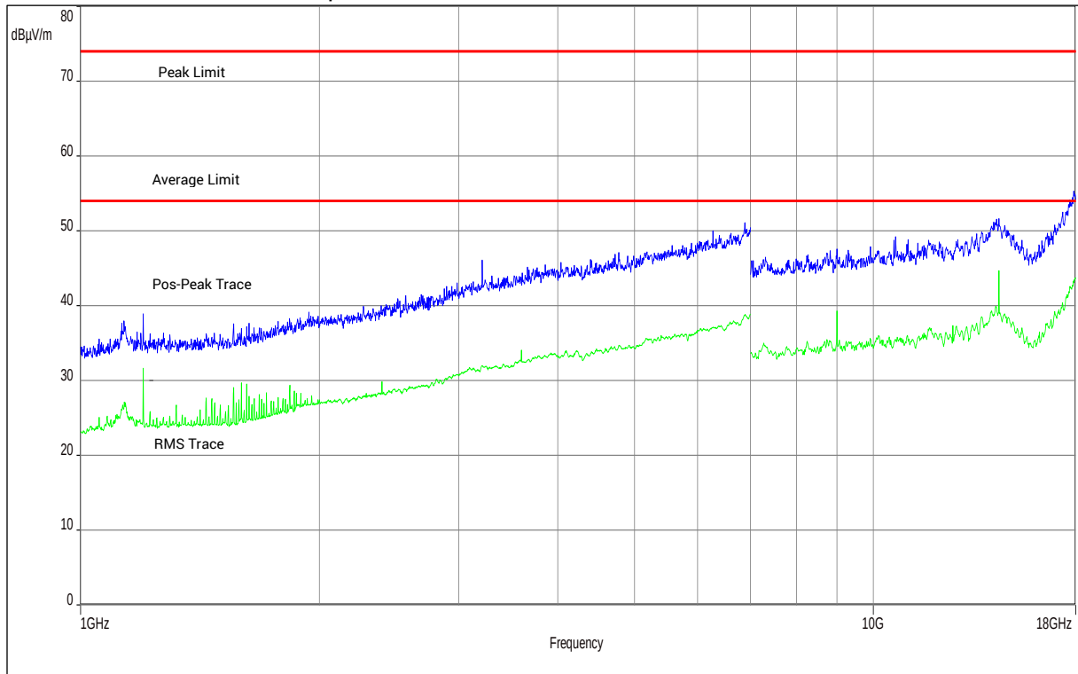
Plot 57: 1 GHz – 18 GHz, valid for specified modes, antenna vertical / horizontal
