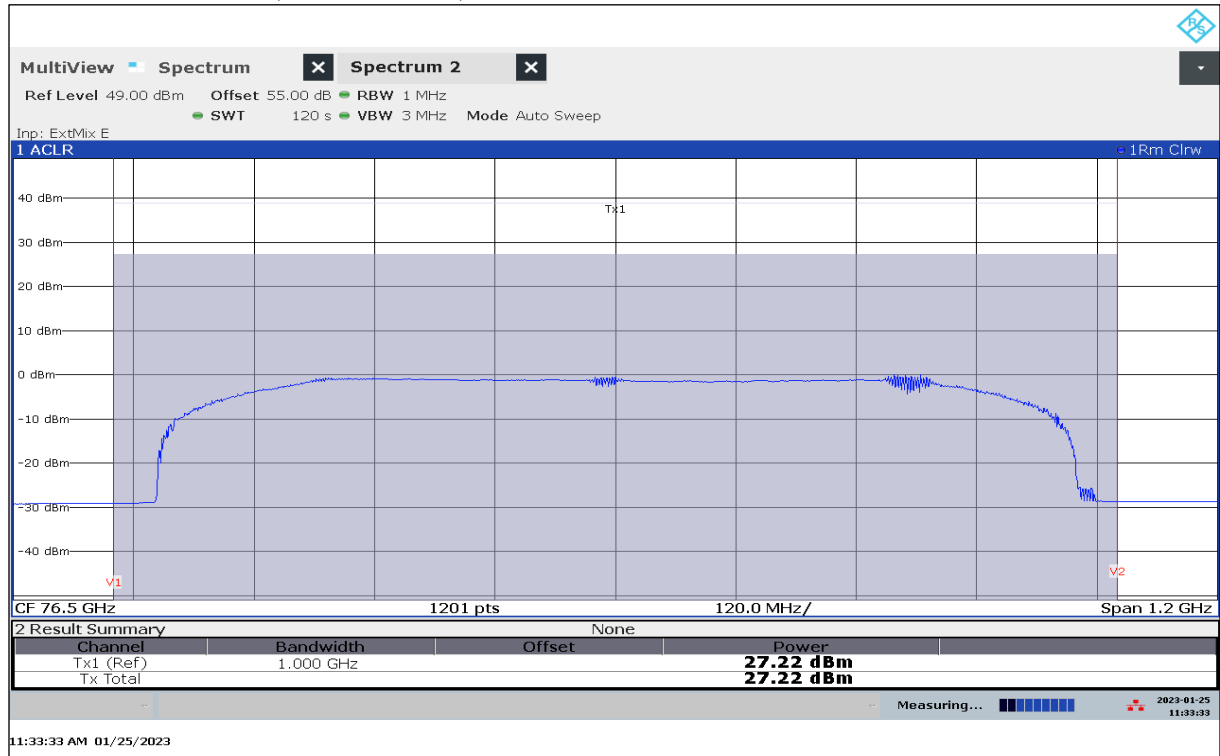
Plot 32: EIRP Mean Power (Channel Power), Mode 09, RMS detector, T_{\text{min}} / V_{\text{min-max}}
