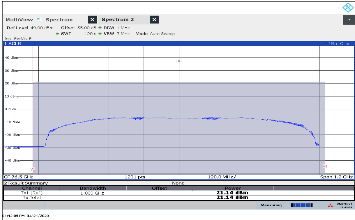
Plot 42: EIRP Mean Power (Channel Power), Mode 27, RMS detector, T_{\max} / V_{\min-\max}
