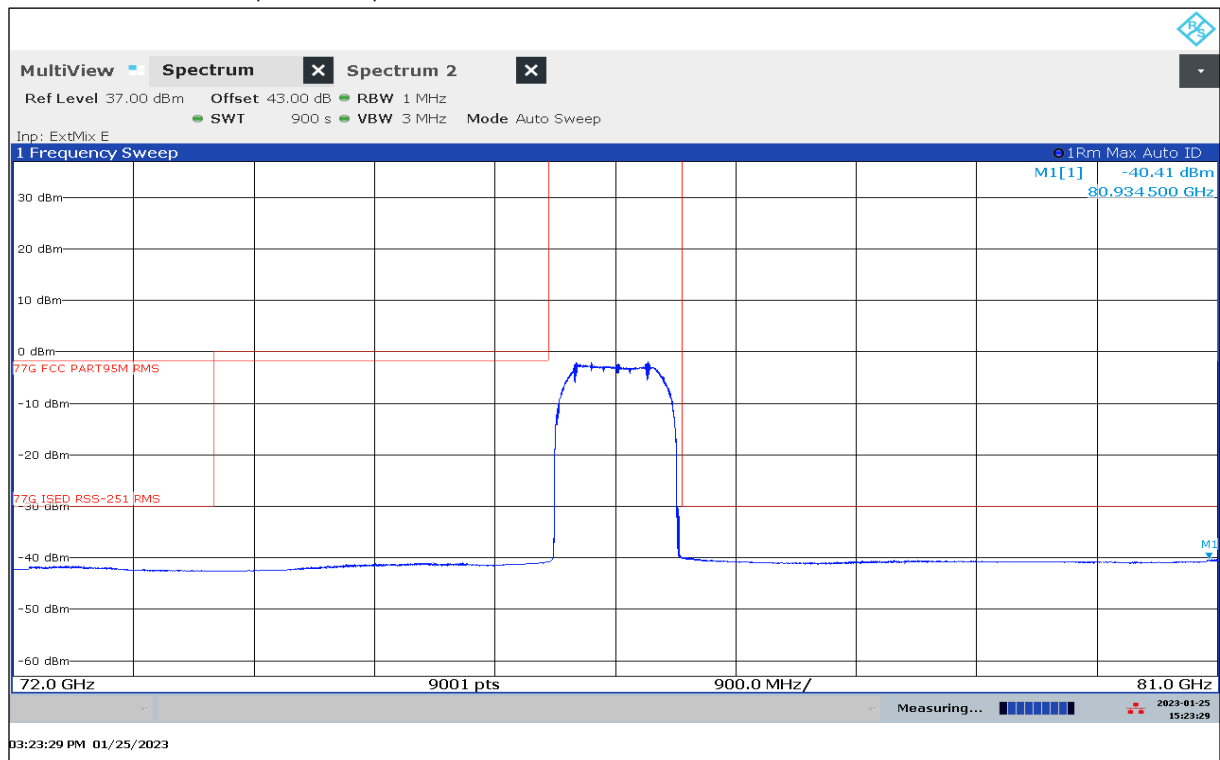
Plot 65: 72 GHz – 81 GHz, Mode 09, antenna vertical / horizontal
