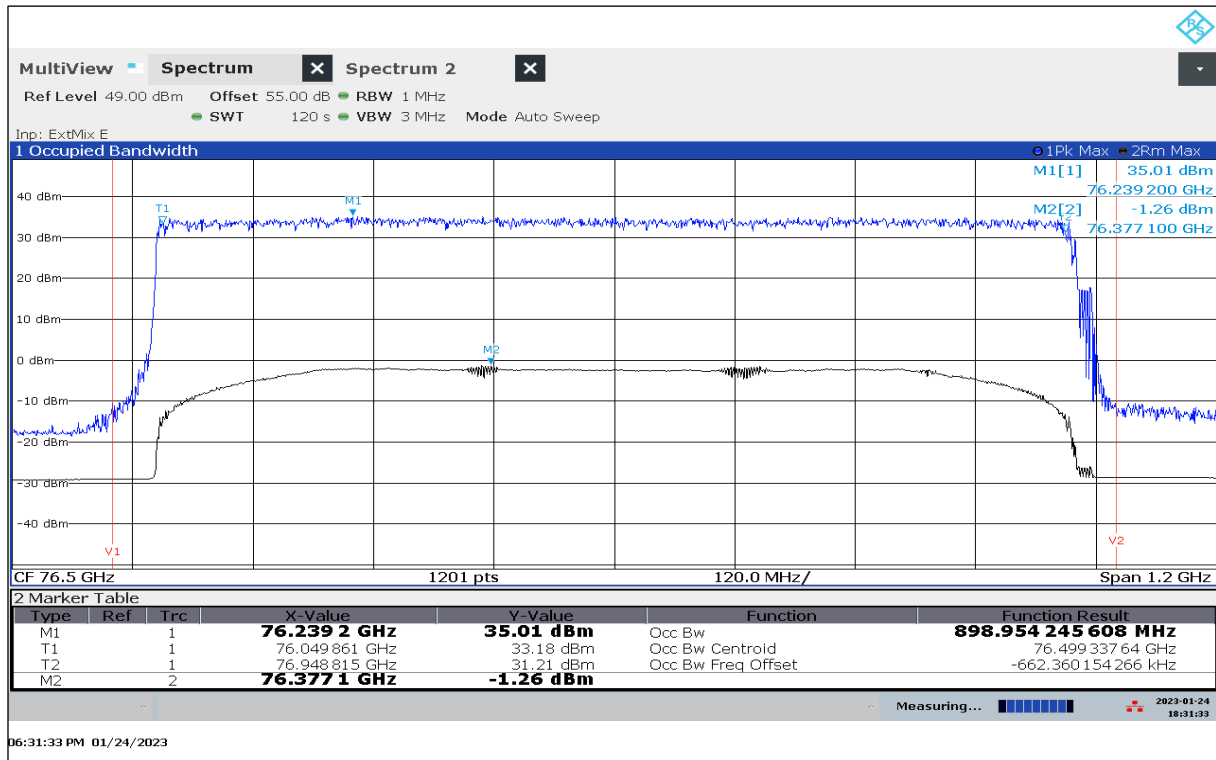
Plot 85: Mode 09, OBW, 50 °C / V min-max
