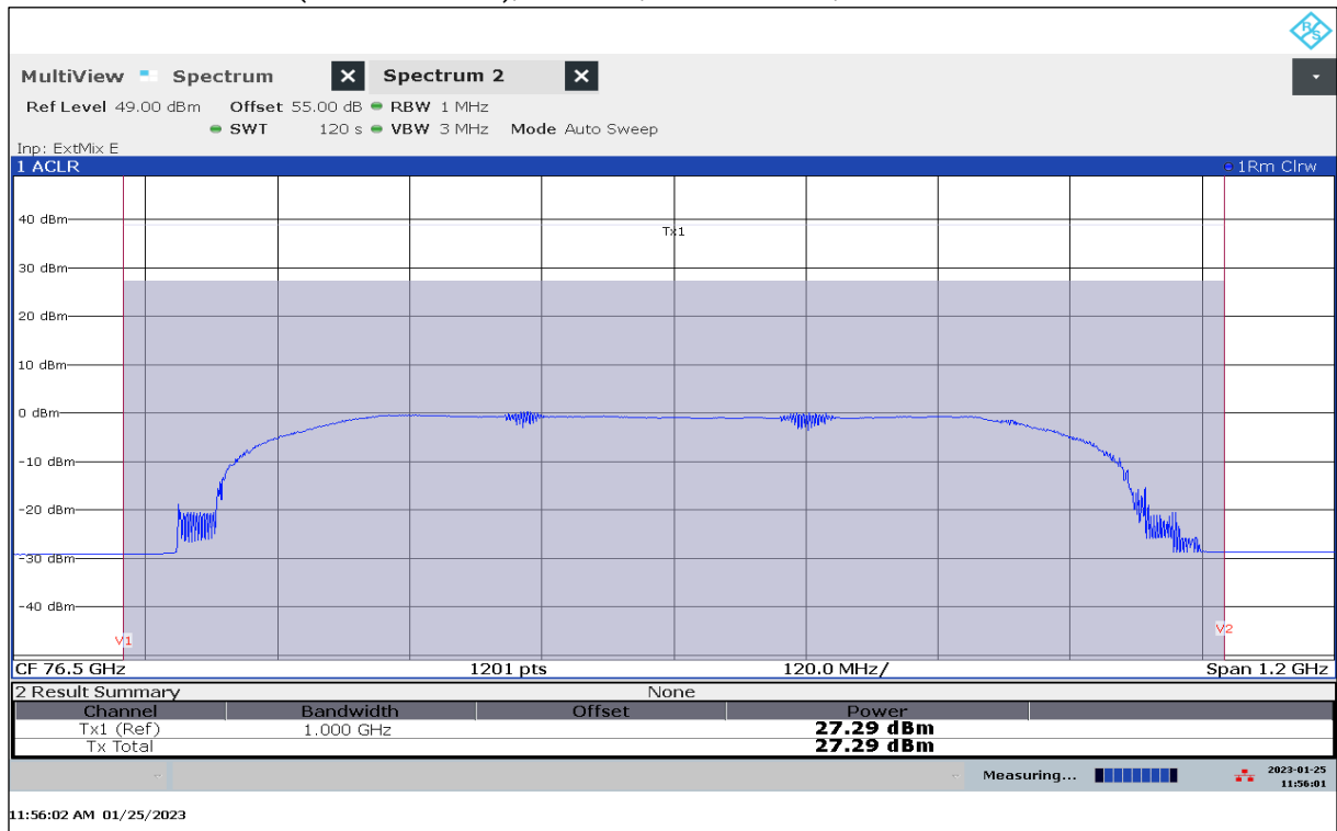
Plot 38: EIRP Mean Power (Channel Power), Mode 21, RMS detector, T_{\text{min}} / V_{\text{min-max}}
