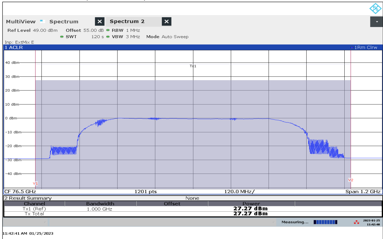
Plot 35: EIRP Mean Power (Channel Power), Mode 15, RMS detector, T_{\min} / V_{\min-\max}
