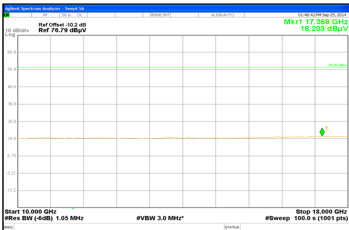
Plot No. 17: 10 GHz to 18 GHz, horizontal/vertical polarization, low/mid/high frequency
