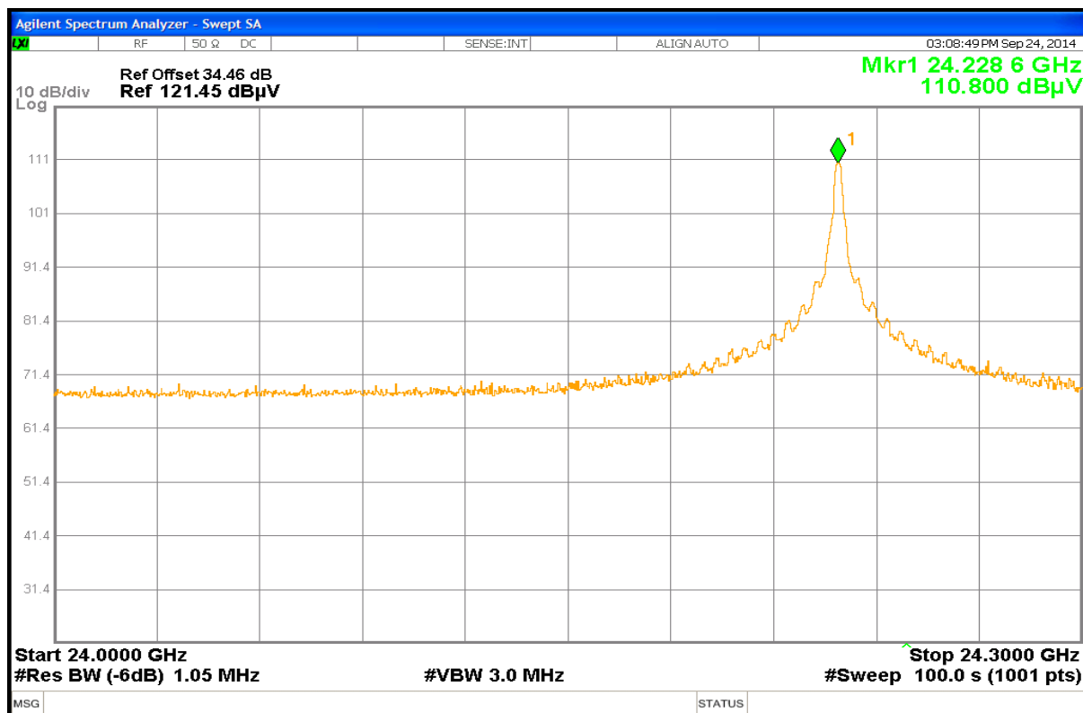
Plot No. 4: Peak measurement, stopped mode, high frequency
