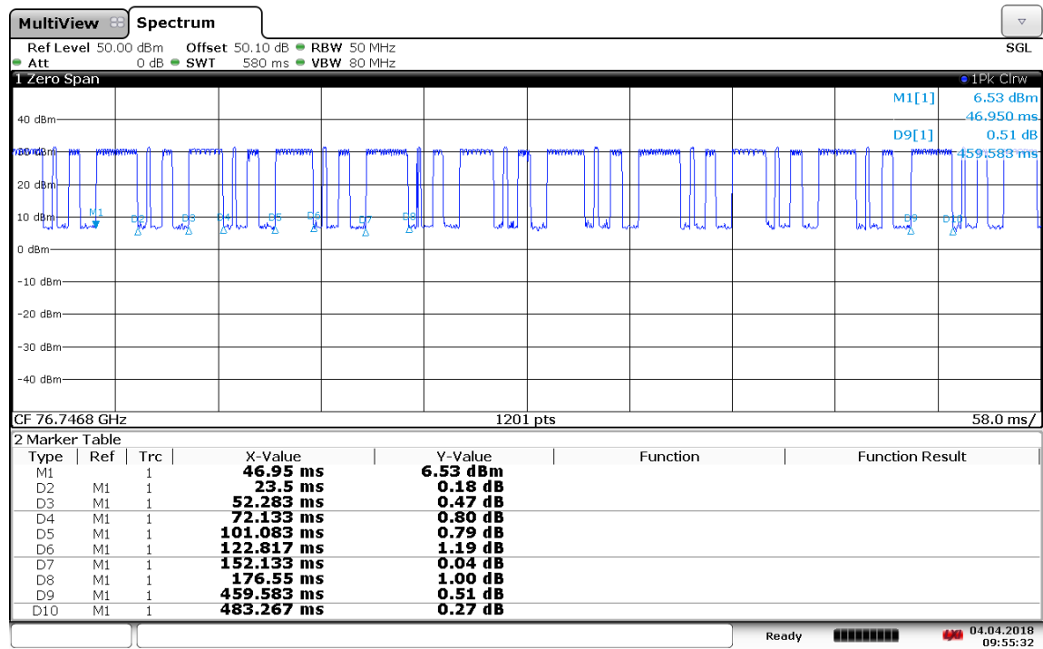
Plot 11: Mode 49, Time domain 76.7468 GHz
