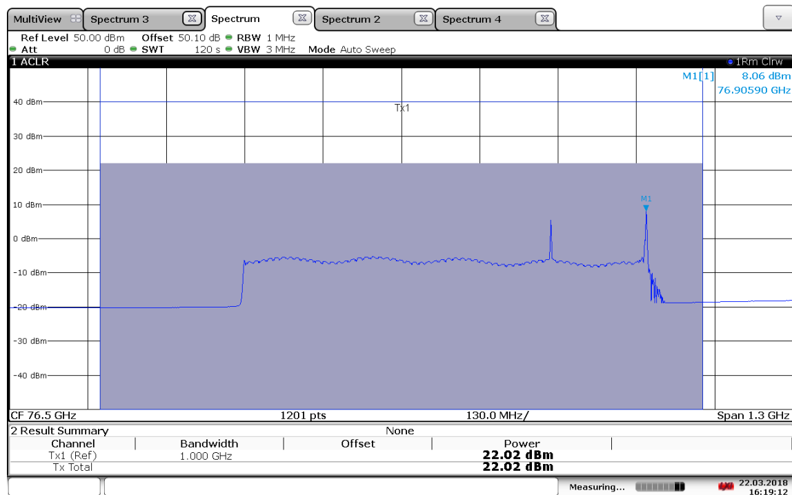
Plot 7: Mode 161, Radiated mean power, T_{\text{nom}} / V_{\text{nom}}
