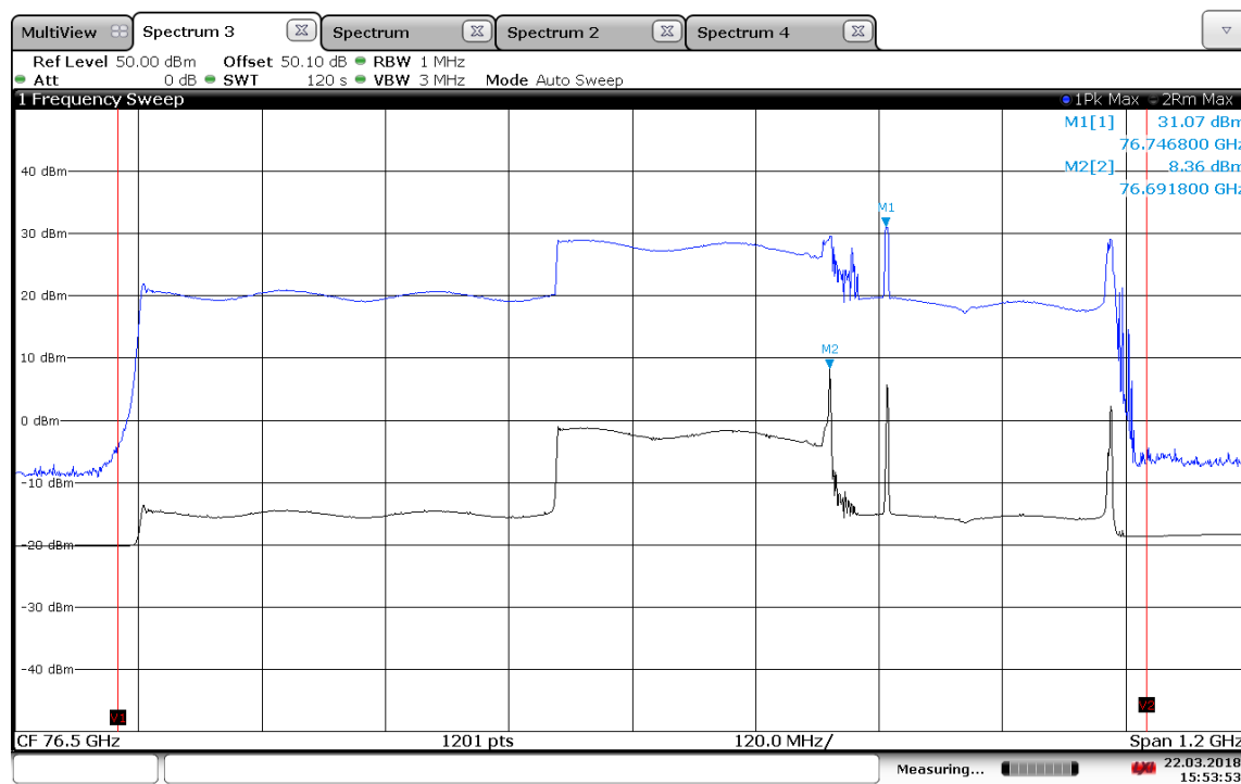
Plot 3: Mode 50, Radiated peak power, T_{\text{nom}} / V_{\text{nom}}
