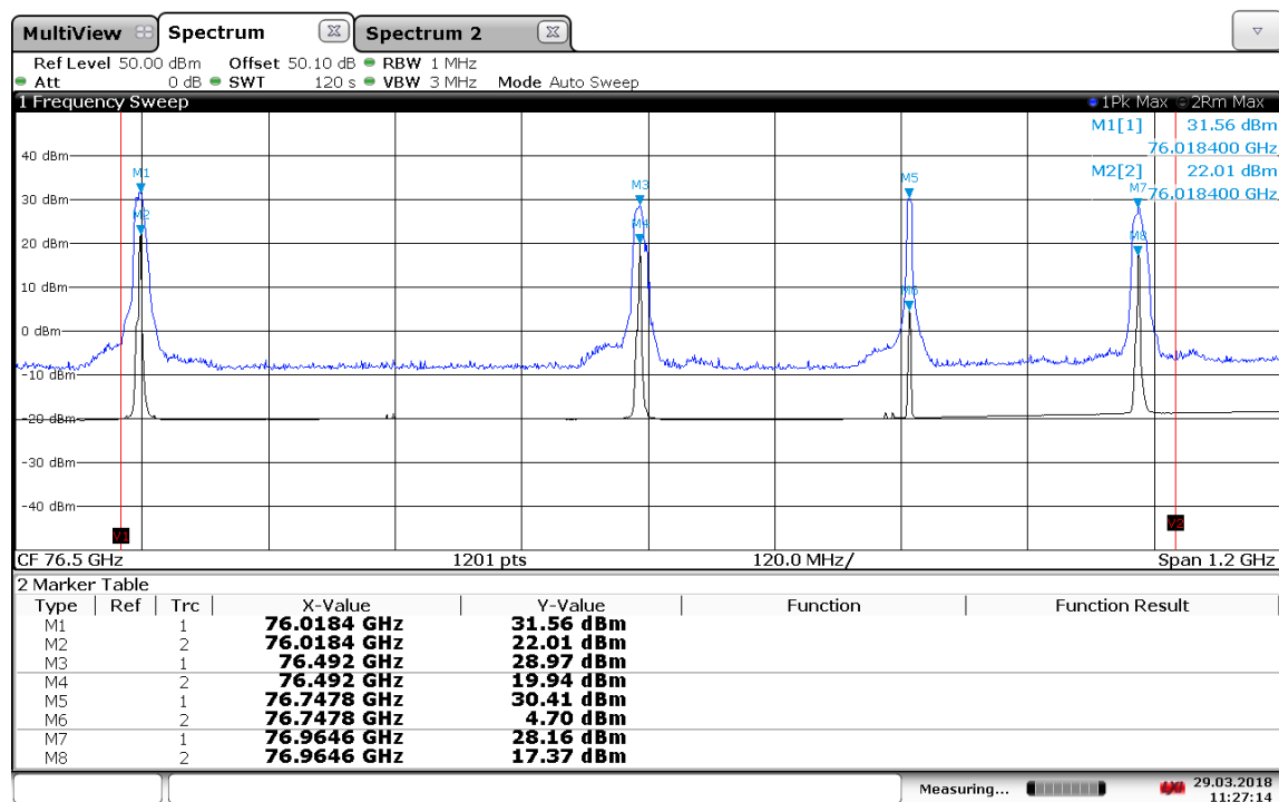
Plot 5: Bottom / Middle / Top, Radiated peak power, T_{\text{nom}} / V_{\text{nom}}
