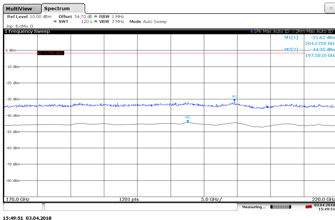
Plot 47: 170 GHz to 220 GHz, bottom, middle, top
