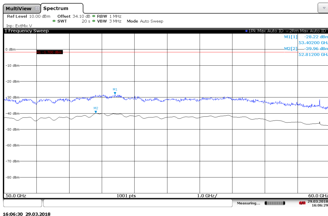
Plot 42: 50 GHz to 60 GHz, bottom, middle, top
