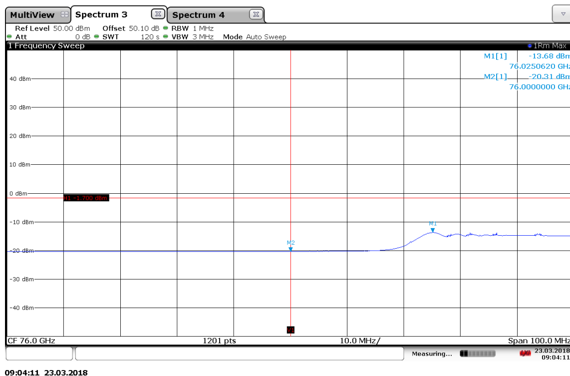
Plot 23: Mode 50, lower BEC
