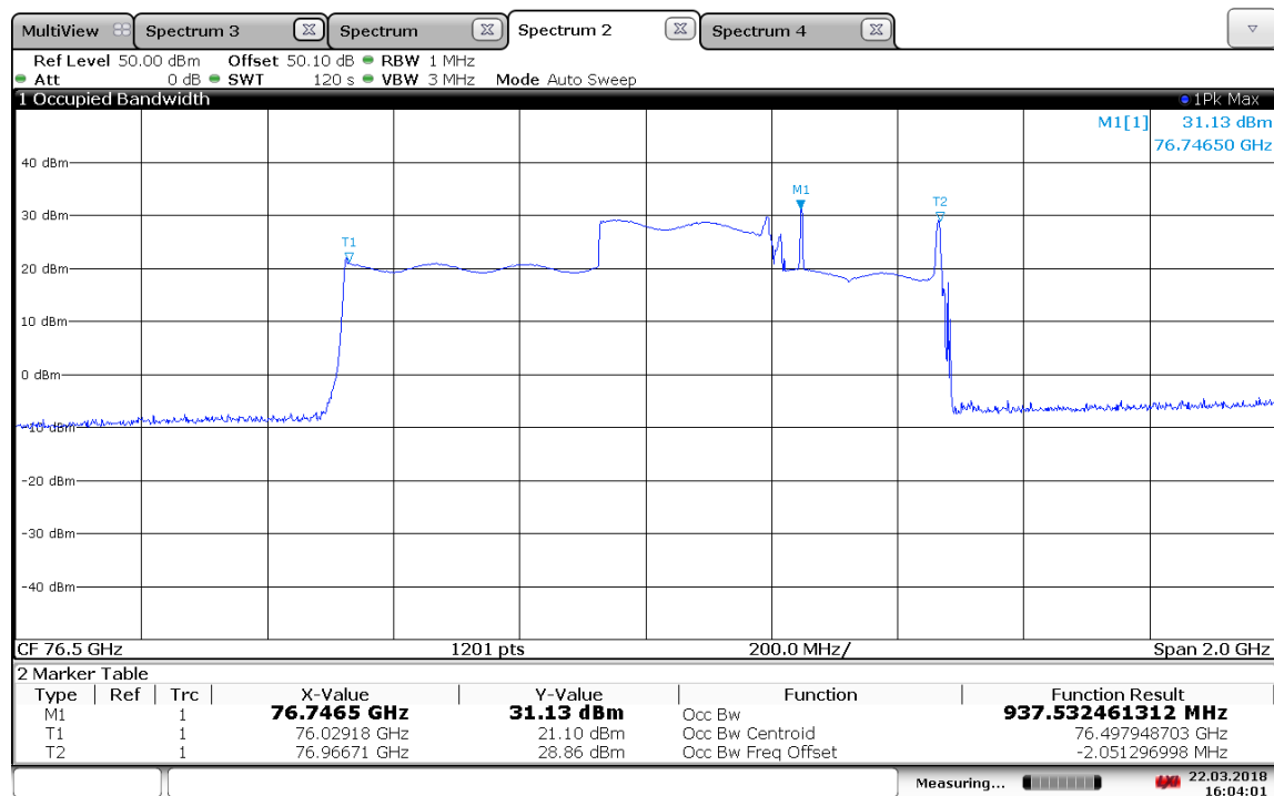
Plot 20: Mode 50, T_{\text{nom}} / V_{\text{nom}}
