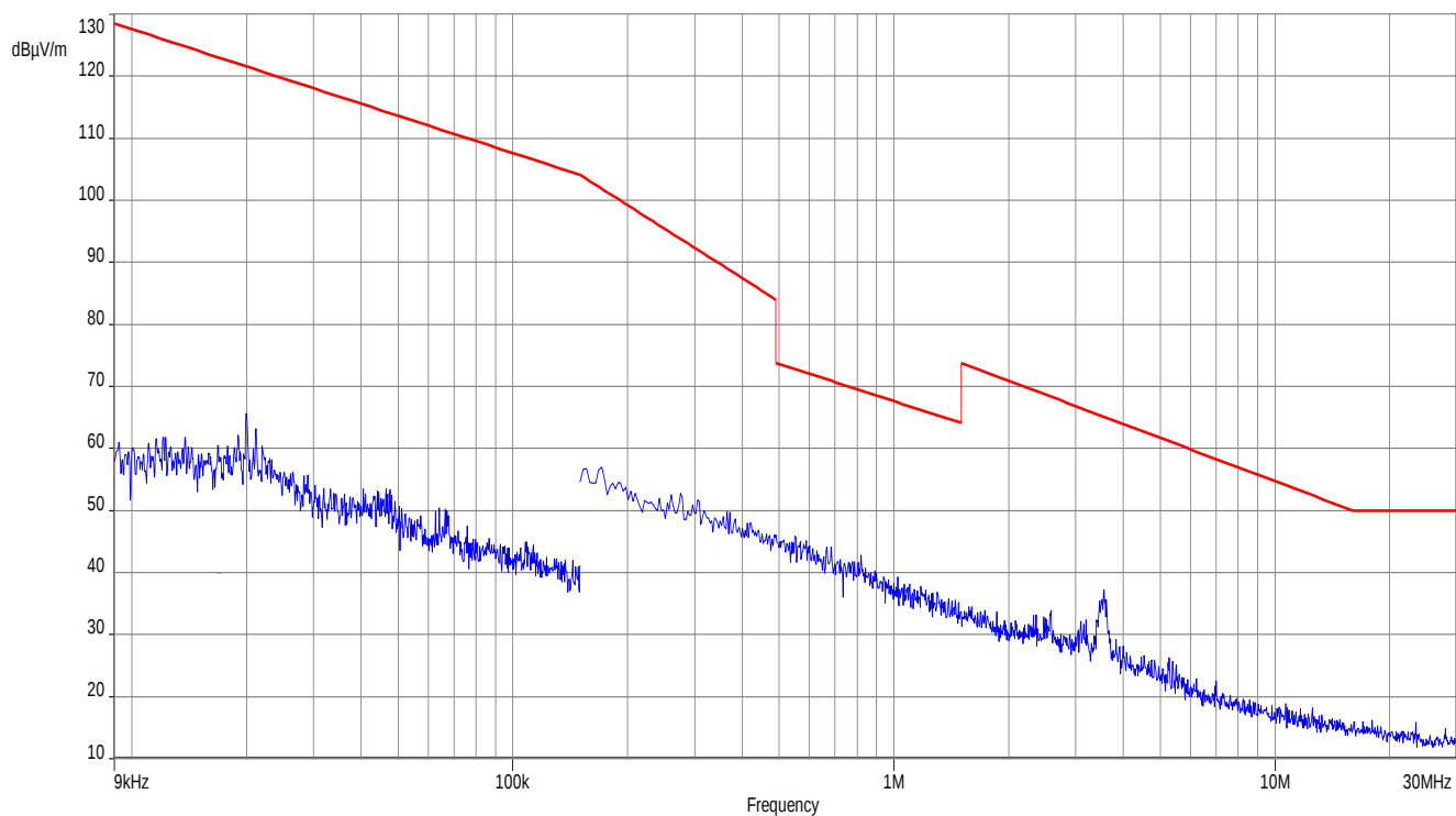
Plot 33: 9 kHz to 30 MHz, bottom
