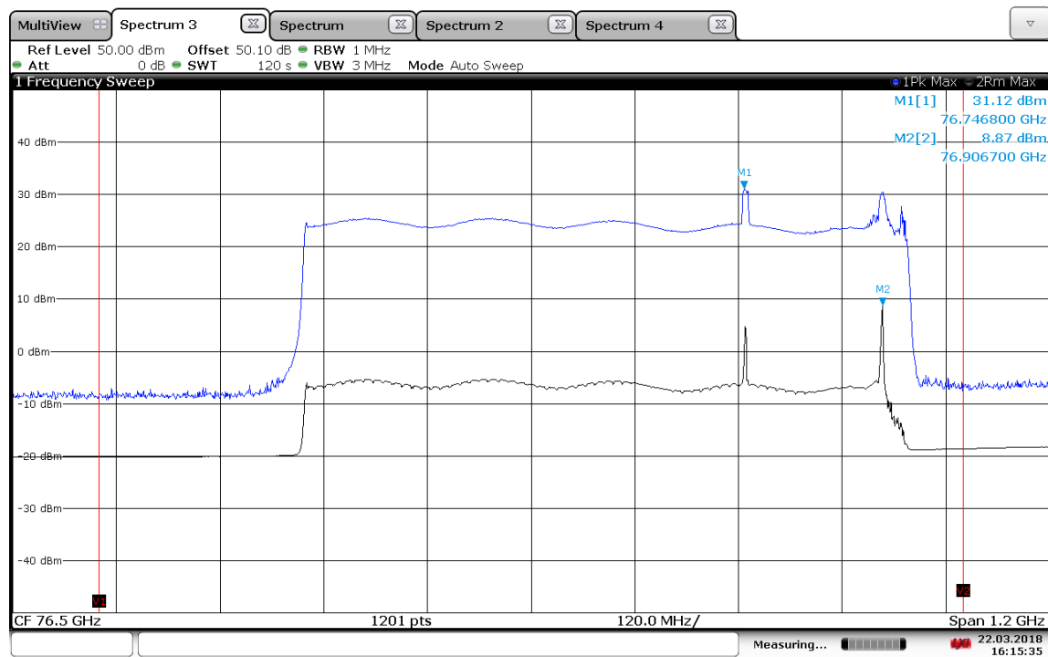
Plot 6: Mode 161, Radiated peak power, T_{\text{nom}} / V_{\text{nom}}
