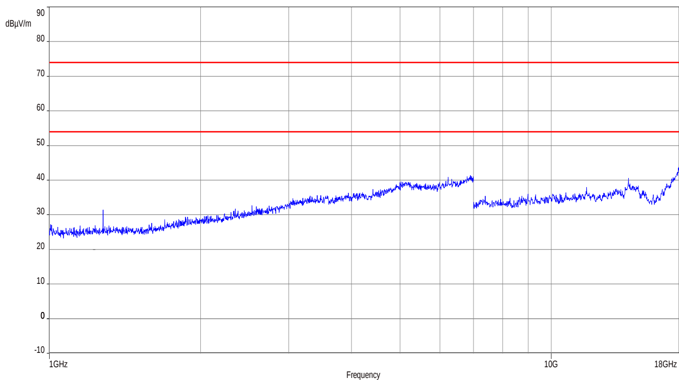
Plot 34: 1 GHz to 18 GHz, bottom
