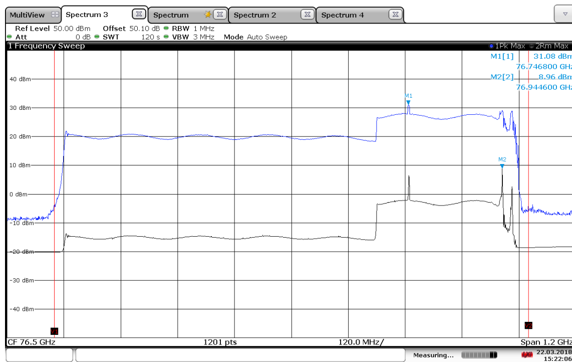
Plot 1: Mode 49, Radiated peak power, T_{\text{nom}} / V_{\text{nom}}
