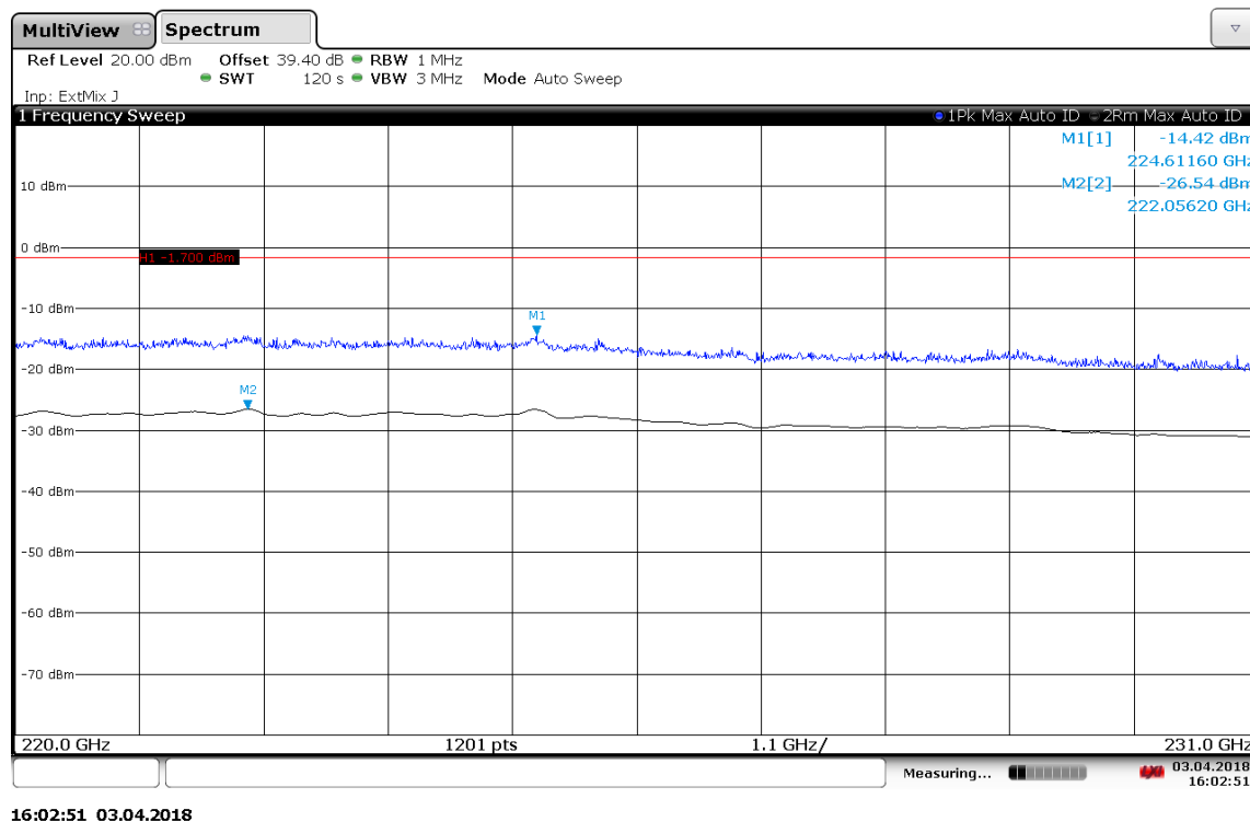
Plot 48: 220 GHz to 231 GHz, bottom, middle, top
