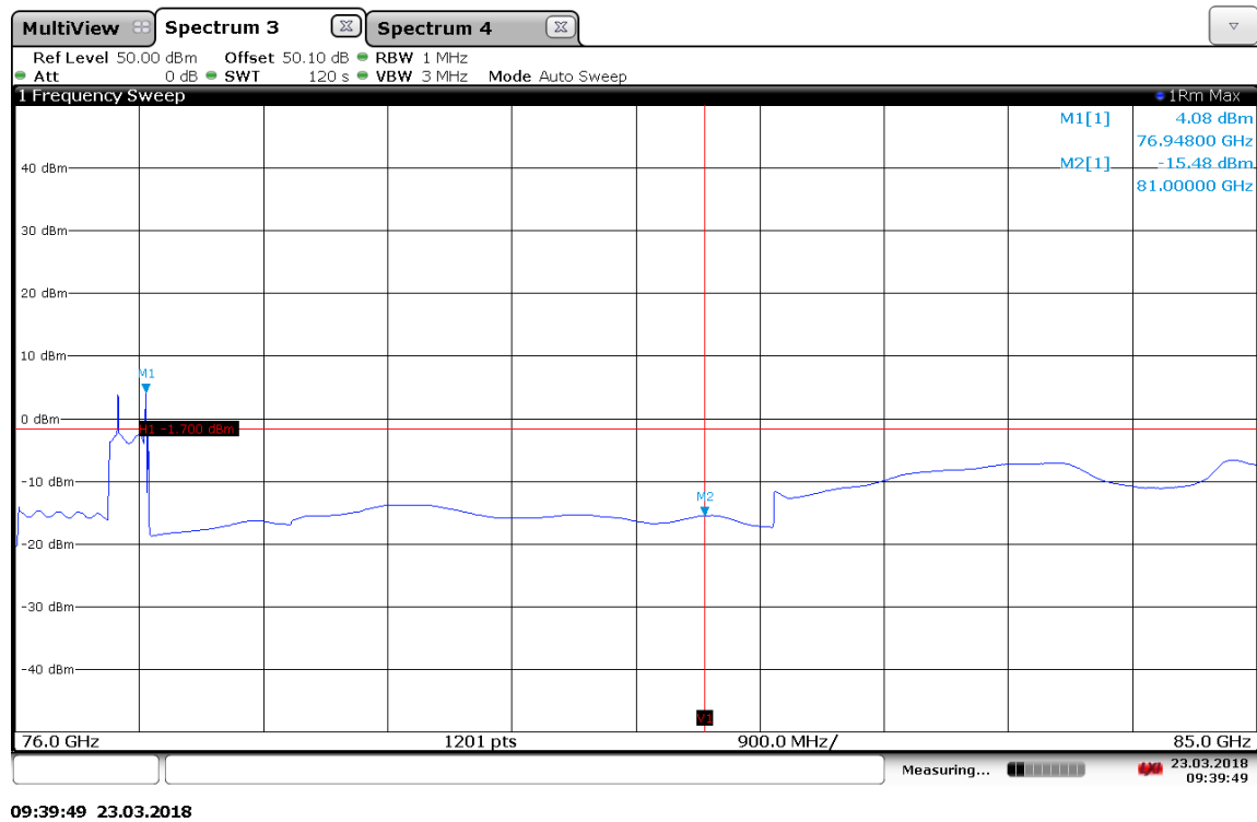
Plot 26: Mode 49, upper BEC
