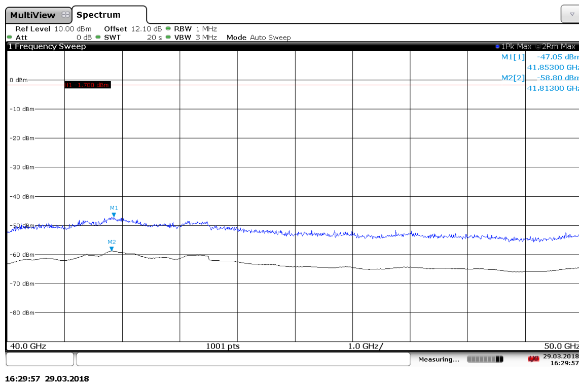
Plot 41: 40 GHz to 50 GHz, bottom, middle, top
