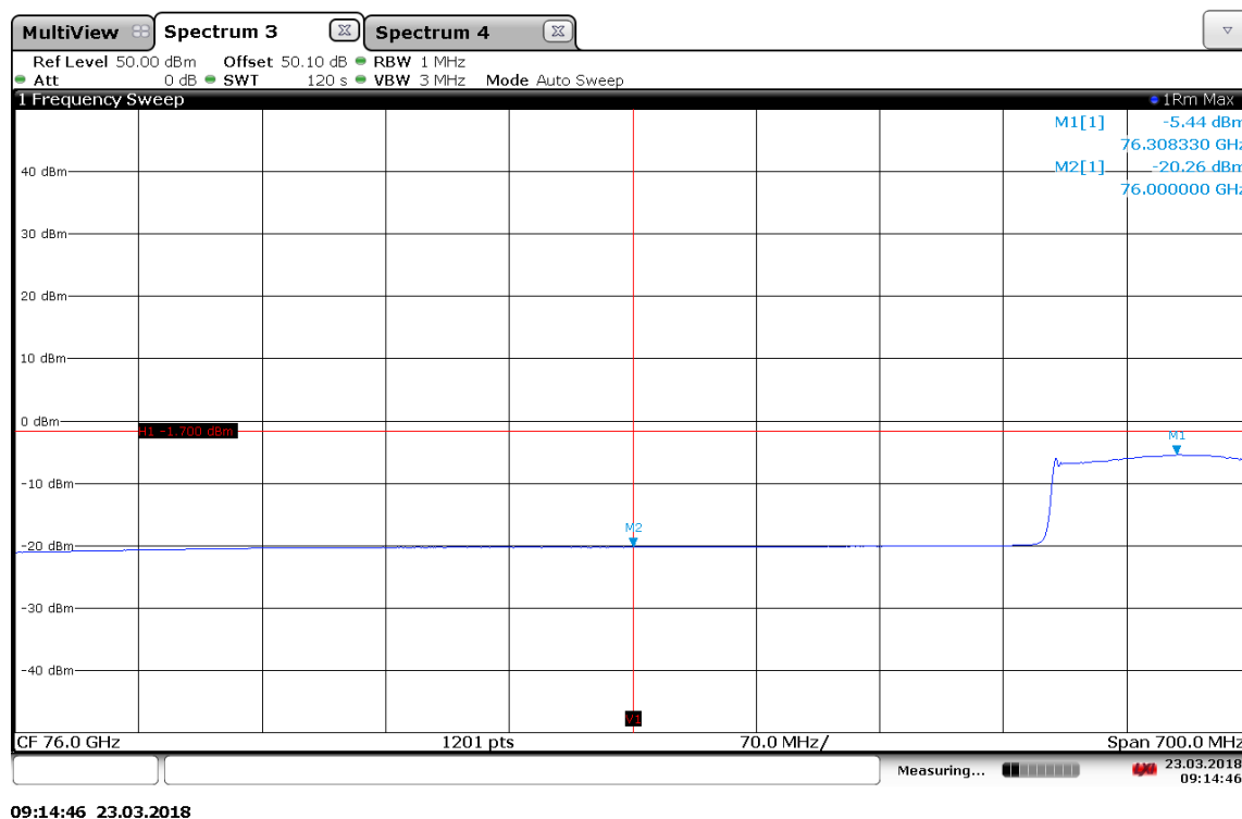
Plot 24: Mode 161, lower BEC
