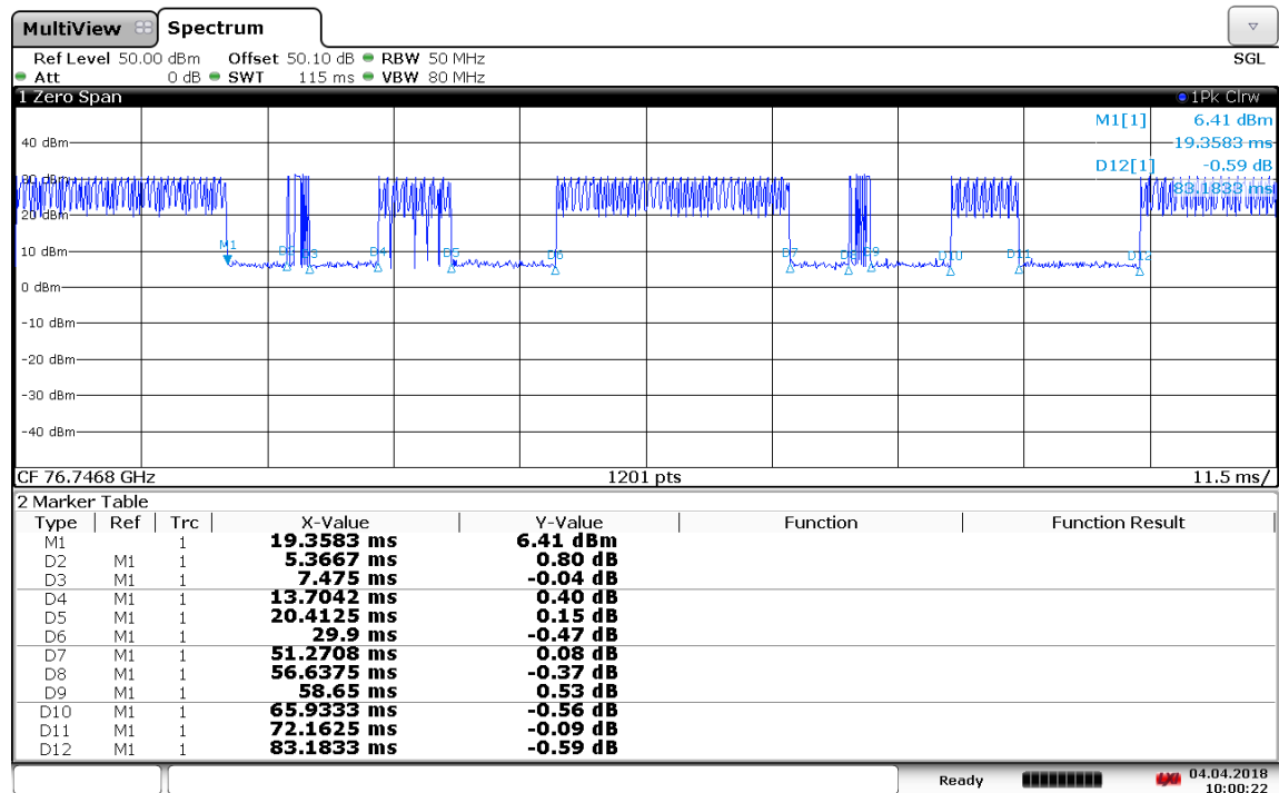
Plot 12: Mode 49, Time domain 76.7468 GHz
