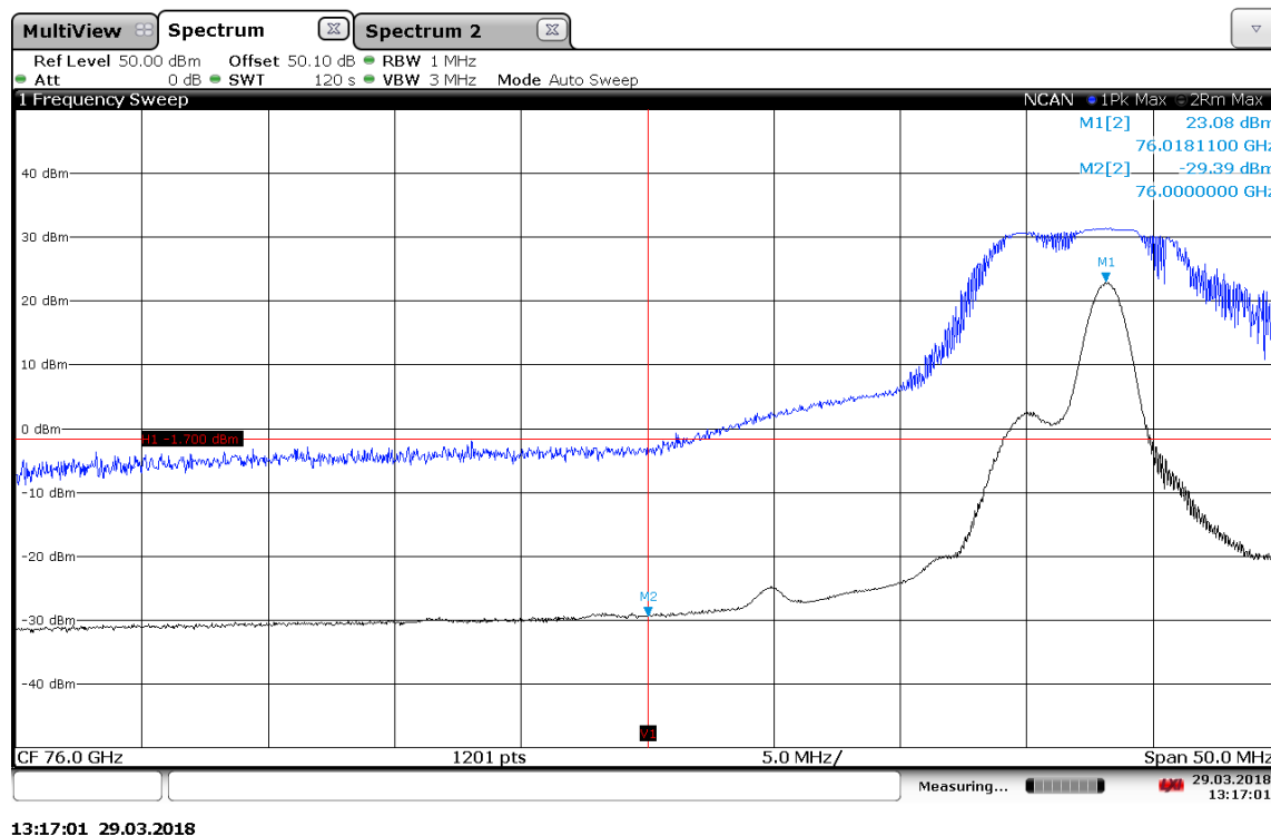
Plot 25: Bottom, lower BEC
