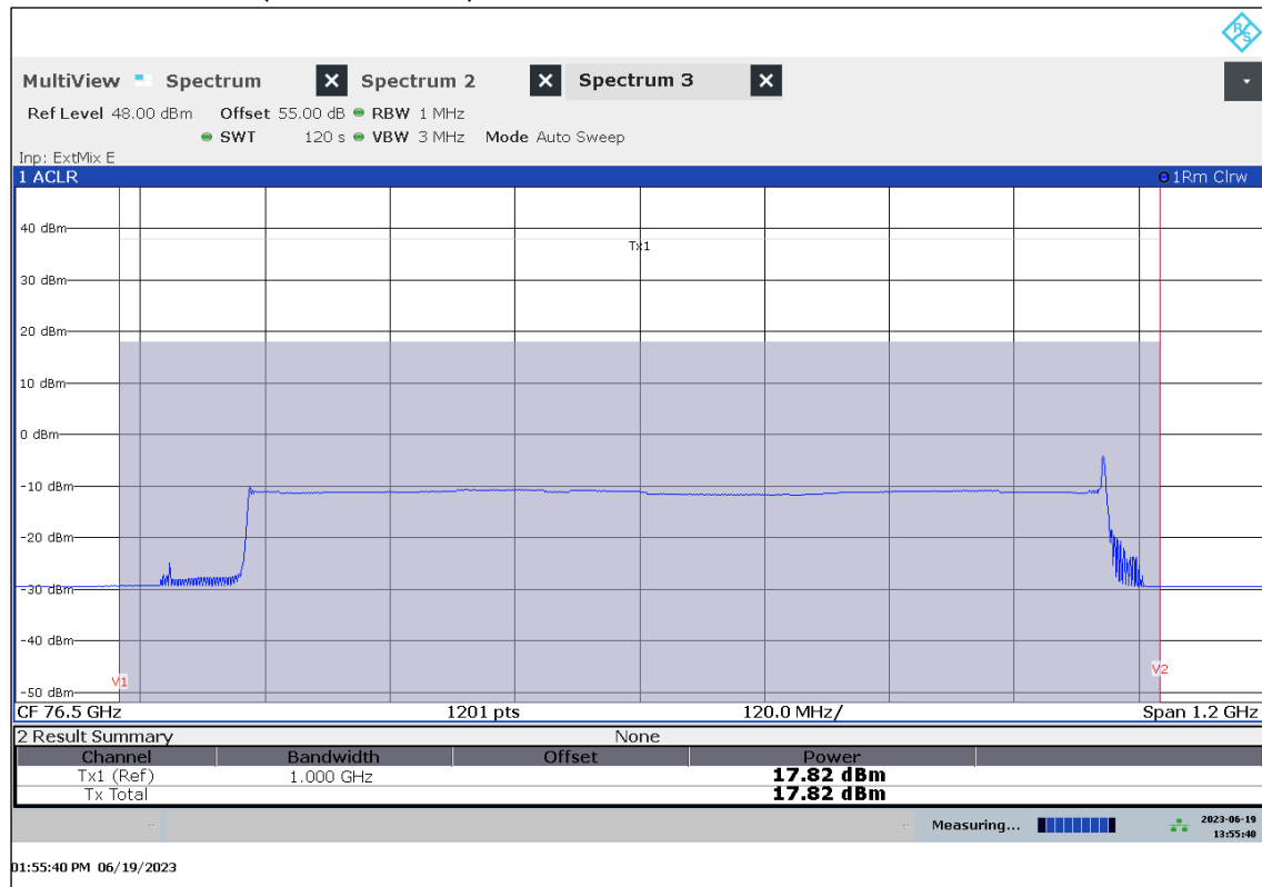
Plot 14: EIRP Mean Power (Channel Power), Mode 68, RMS detector, T_{\text{nom}} / V_{\text{nom}}
