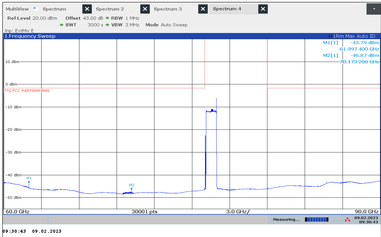
Plot 30: 60 GHz – 90 GHz, OOB, Mode 68, antenna vertical / horizontal
