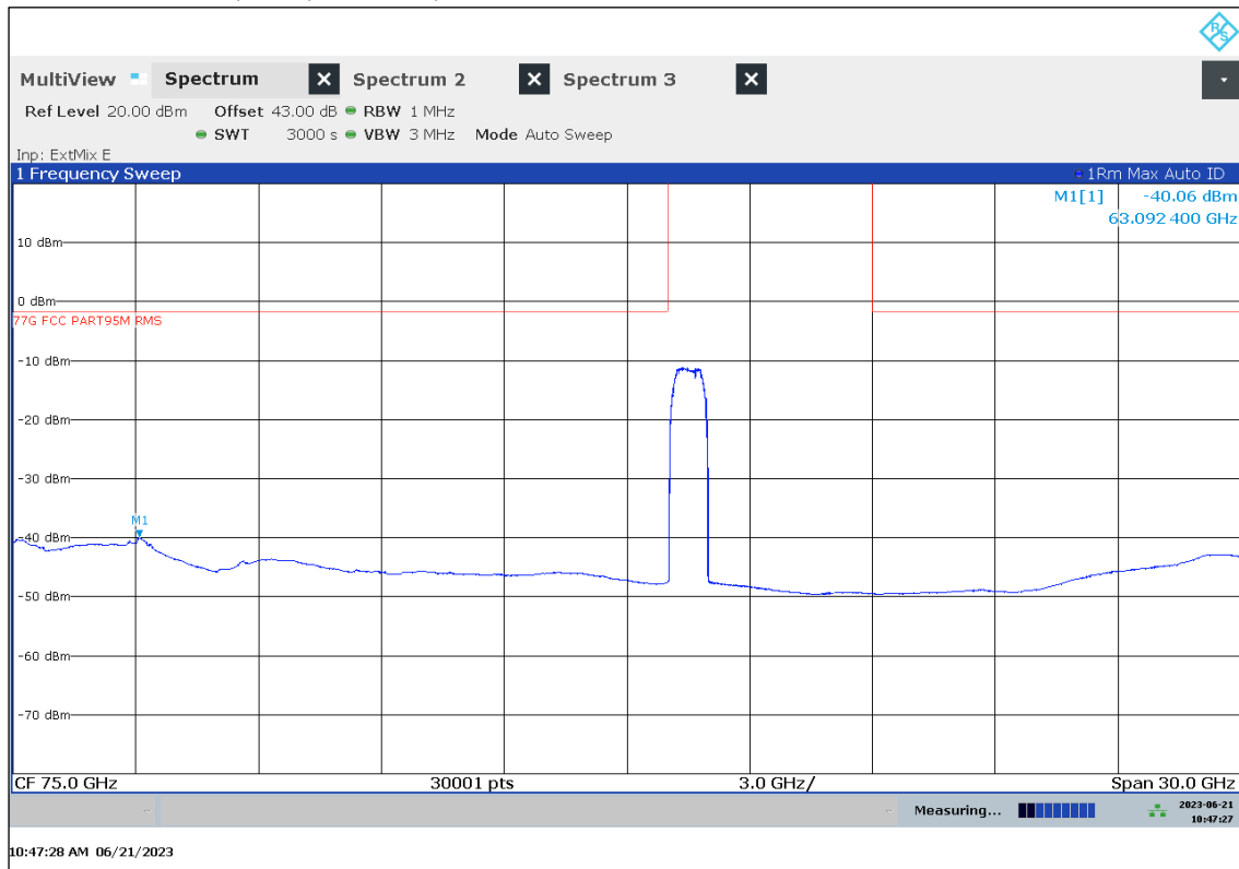
Plot 29: 60 GHz – 90 GHz, OOB, Mode 45, antenna vertical / horizontal
