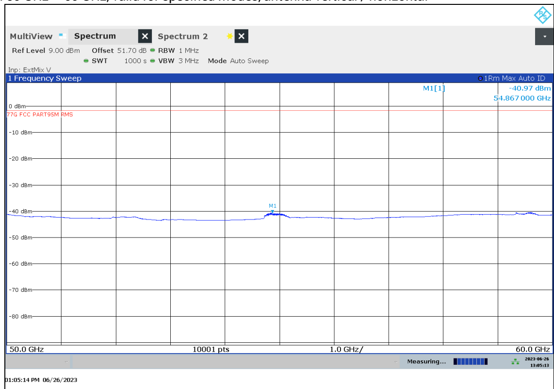
Plot 23: 50 GHz – 60 GHz, valid for specified modes, antenna vertical / horizontal
