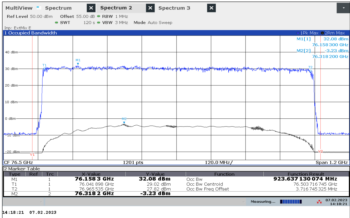
Plot 1: OBW, Mode 03, T_{\text{nom}} / V_{\text{min-max}}
