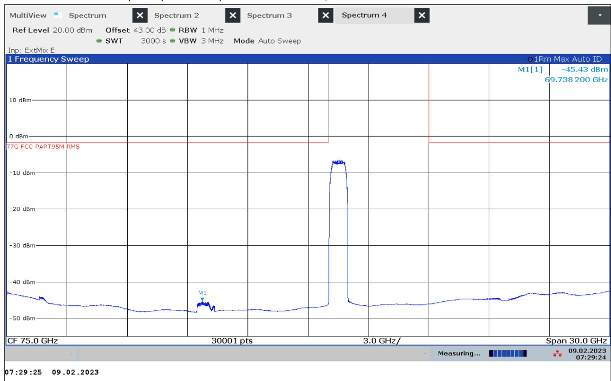
Plot 56: 60 GHz – 90 GHz, OOB, Mode 45, antenna vertical / horizontal
