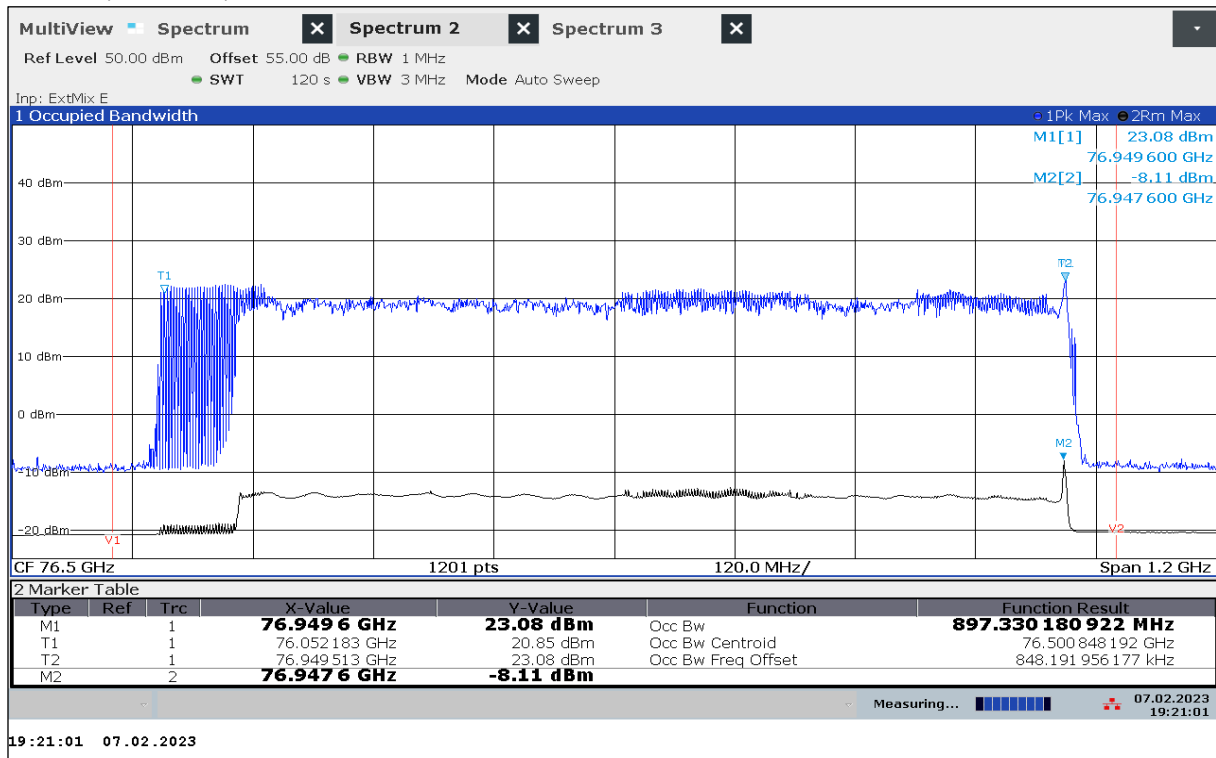
Plot 20: OBW, Mode 68, T_{\text{min}} / V_{\text{min-max}}
