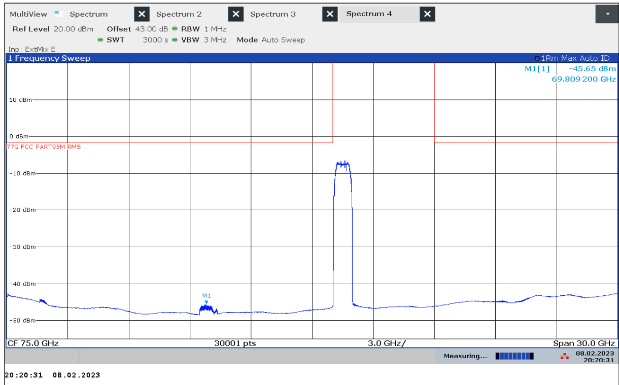
Plot 55: 60 GHz – 90 GHz, OOB, Mode 33, antenna vertical / horizontal
