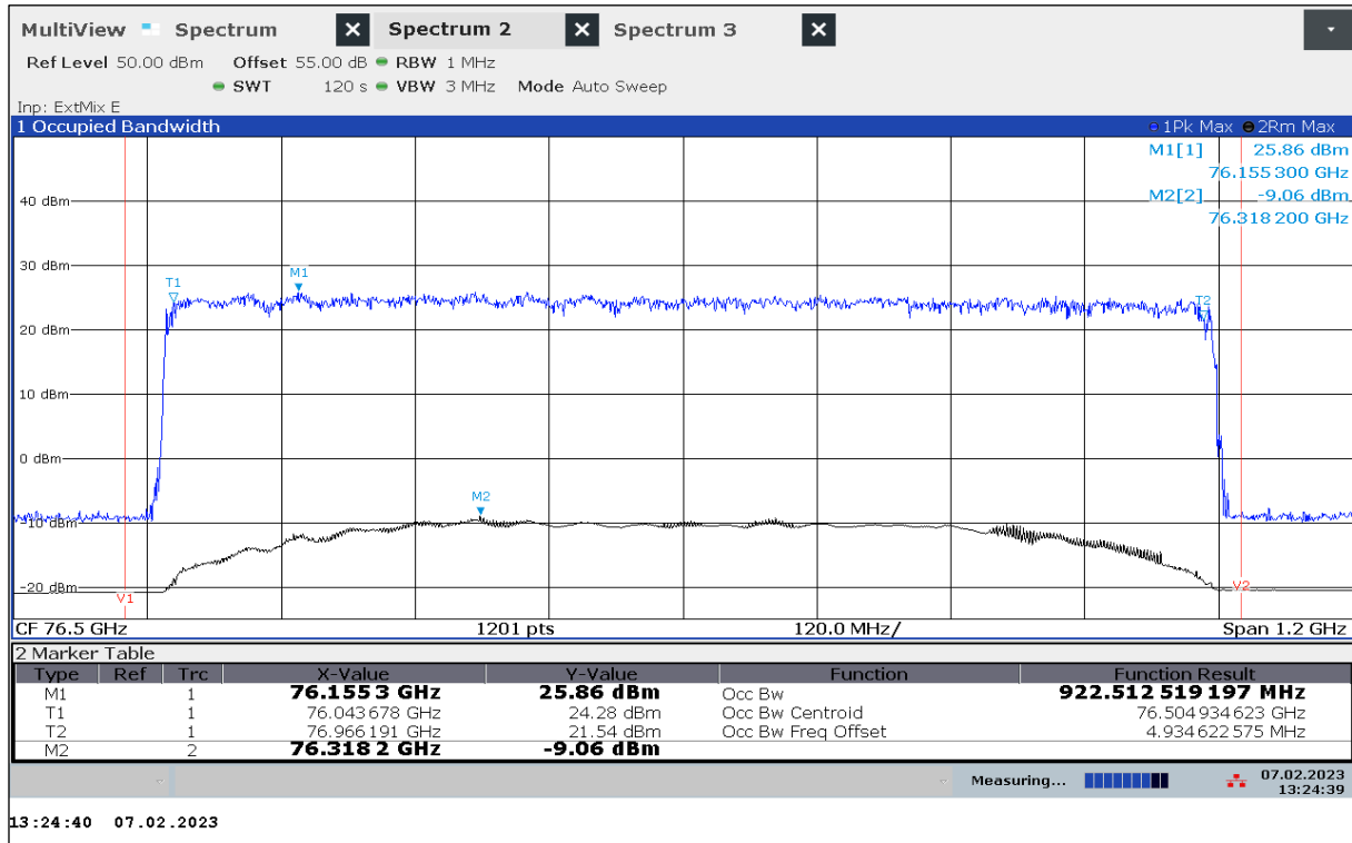
Plot 10: OBW, Mode 21, T_{\text{nom}} / V_{\min-\max}
