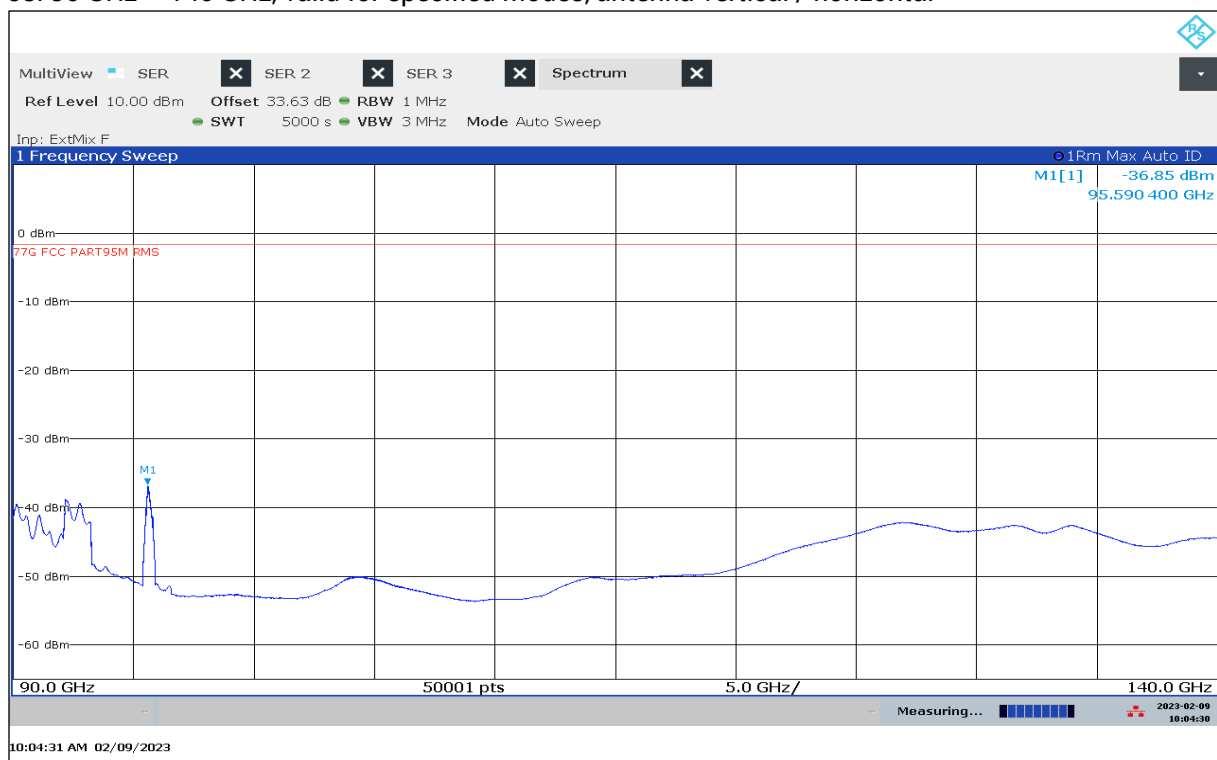
Plot 58: 90 GHz – 140 GHz, valid for specified modes, antenna vertical / horizontal
