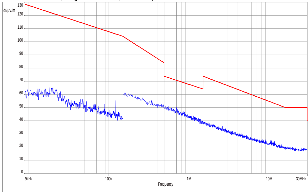
Plot 43: 9 kHz – 30 MHz, Magnetic antenna, valid for specified modes
