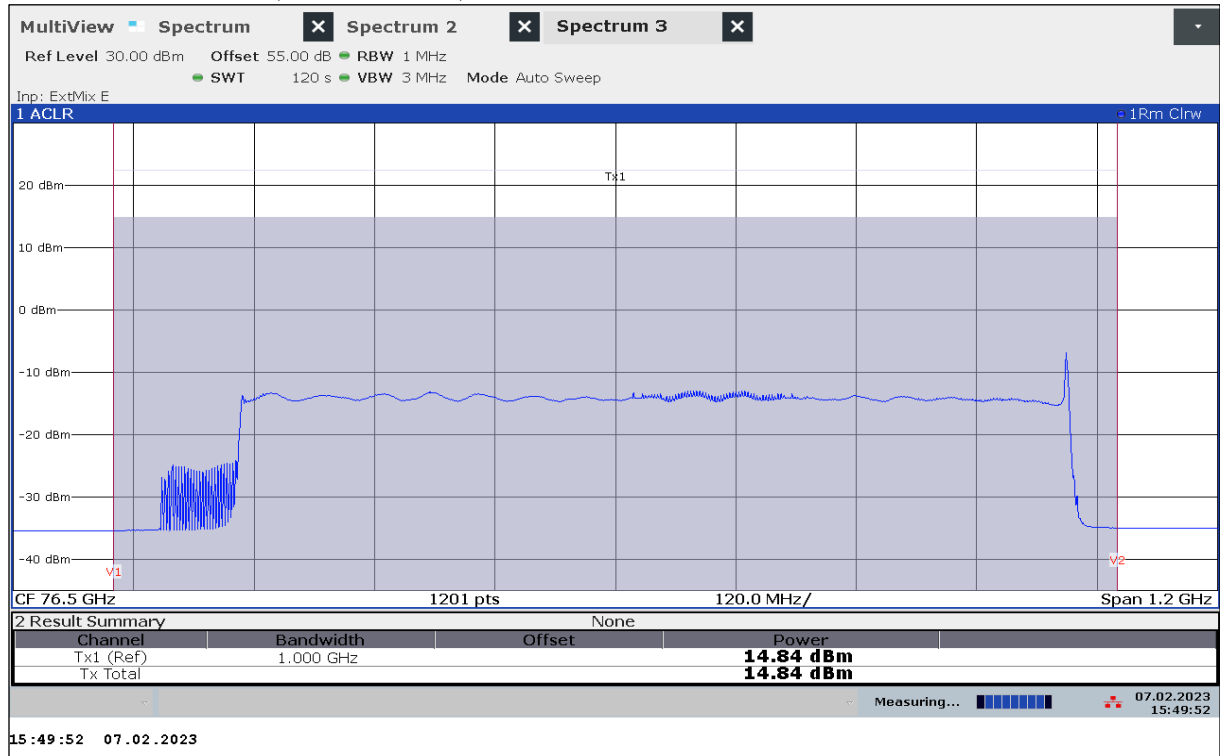
Plot 42: EIRP Mean Power (Channel Power), Mode 68, RMS detector, T_{\max} / V_{\min-max}
