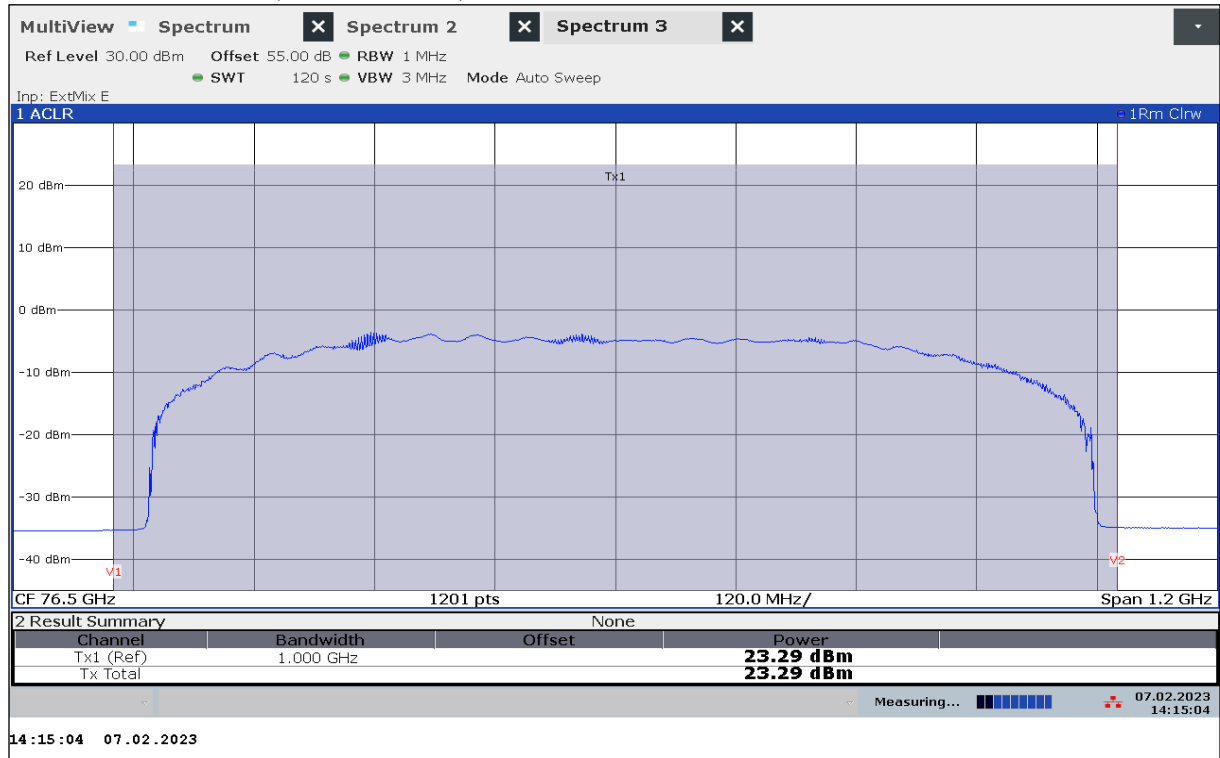
Plot 22: EIRP Mean Power (Channel Power), Mode 03, RMS detector, T_{\text{nom}} / V_{\min-\max}
