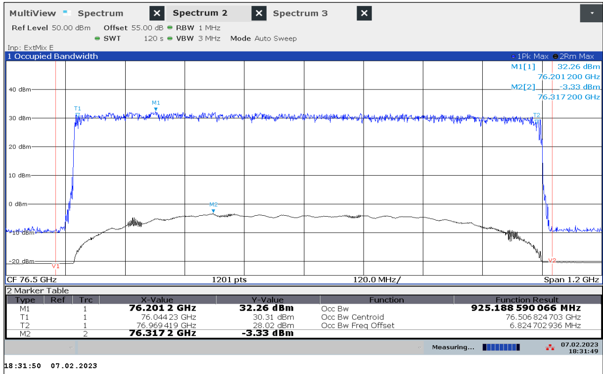
Plot 2: OBW, Mode 03, T_{\text{min}} / V_{\text{min-max}}
