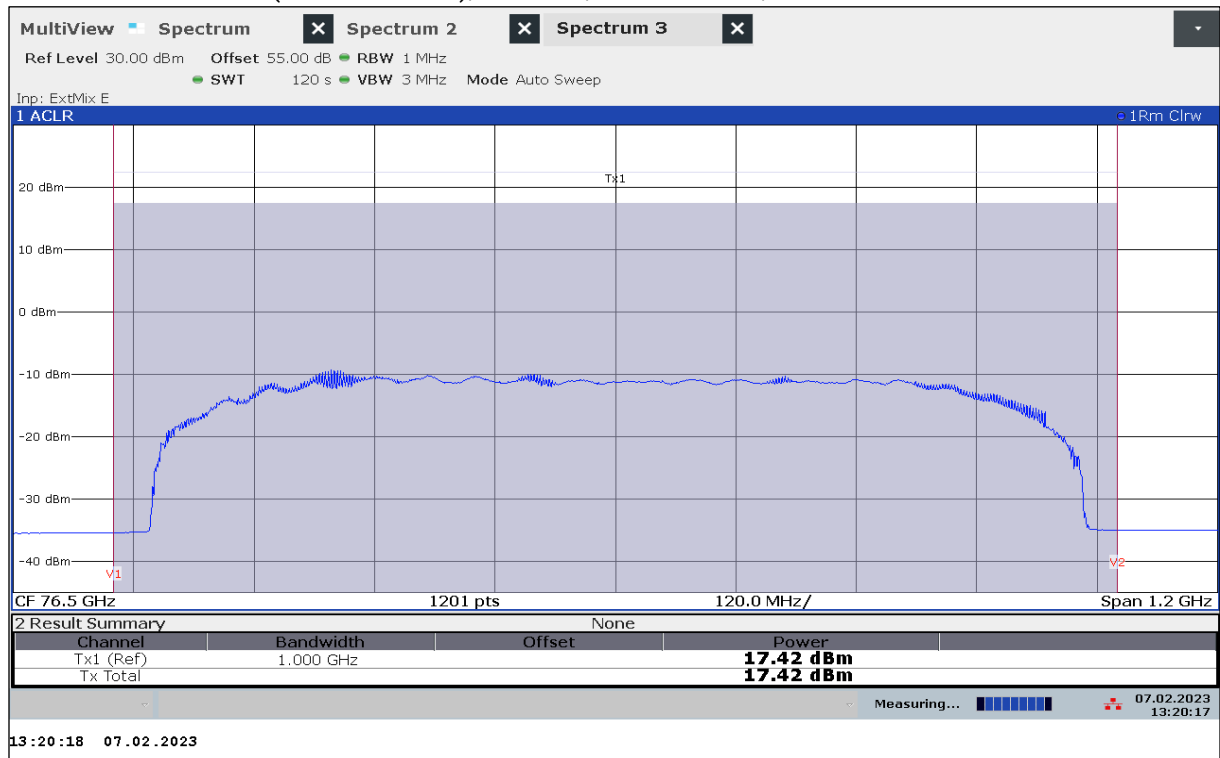
Plot 34: EIRP Mean Power (Channel Power), Mode 33, RMS detector, T_{\text{nom}} / V_{\min-\max}
