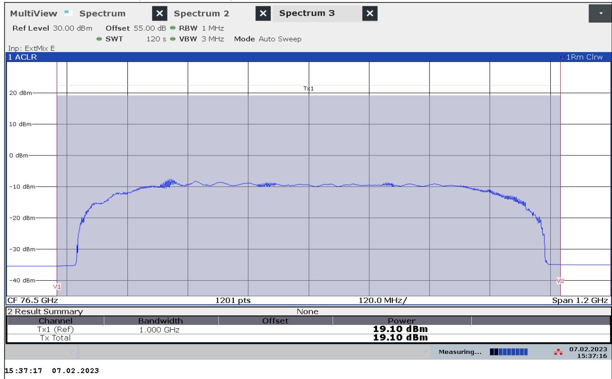
Plot 36: EIRP Mean Power (Channel Power), Mode 33, RMS detector, T_{\max} / V_{\min-max}
