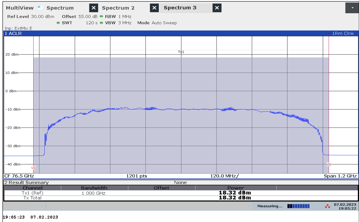
Plot 32: EIRP Mean Power (Channel Power), Mode 21, RMS detector, T_{min} / V_{min-max}
