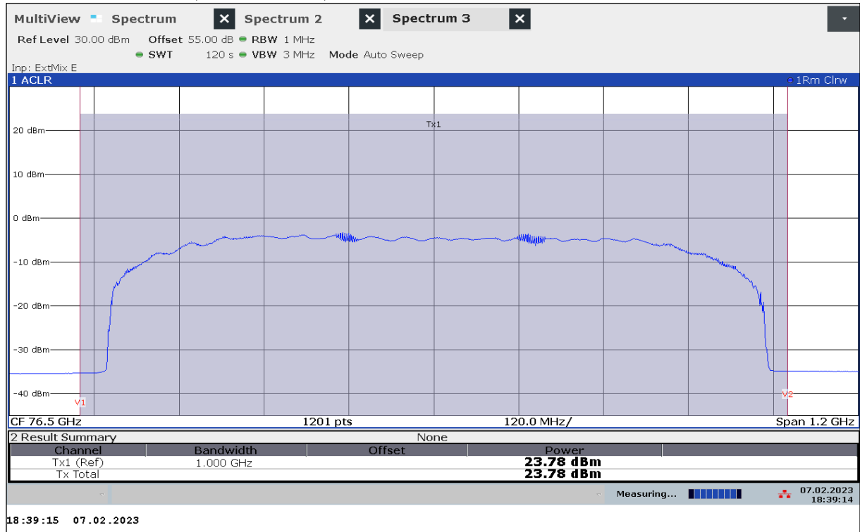
Plot 26: EIRP Mean Power (Channel Power), Mode 09, RMS detector, T_{min} / V_{min-max}
