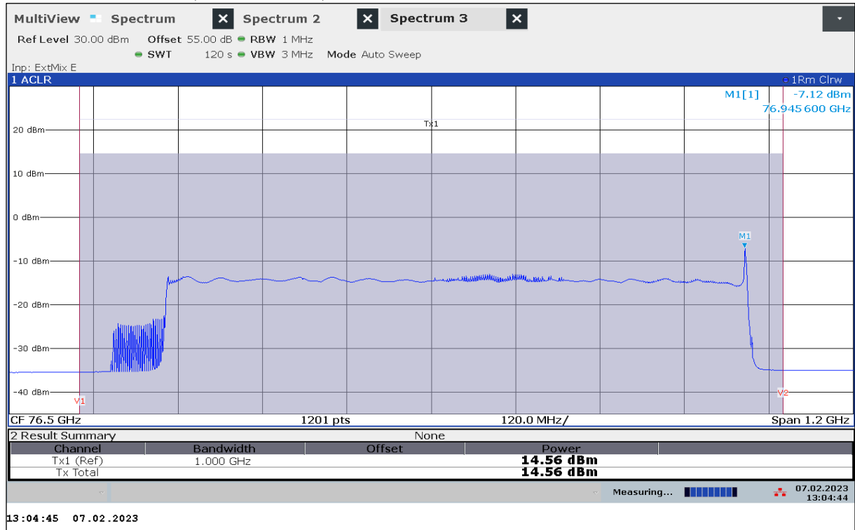
Plot 40: EIRP Mean Power (Channel Power), Mode 68, RMS detector, T_{\text{nom}} / V_{\min-\max}
