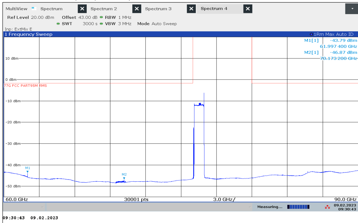
Plot 57: 60 GHz – 90 GHz, OOB, Mode 68, antenna vertical / horizontal
