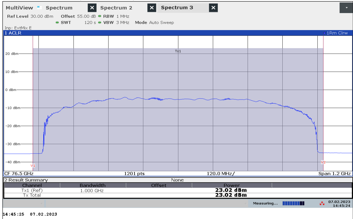
Plot 24: EIRP Mean Power (Channel Power), Mode 03, RMS detector, T_{\max} / V_{\min-\max}
