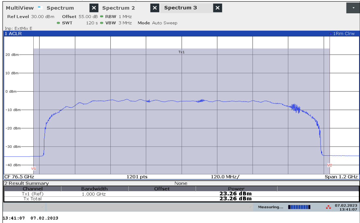
Plot 28: EIRP Mean Power (Channel Power), Mode 15, RMS detector, T_{\text{nom}} / V_{\min-\max}
