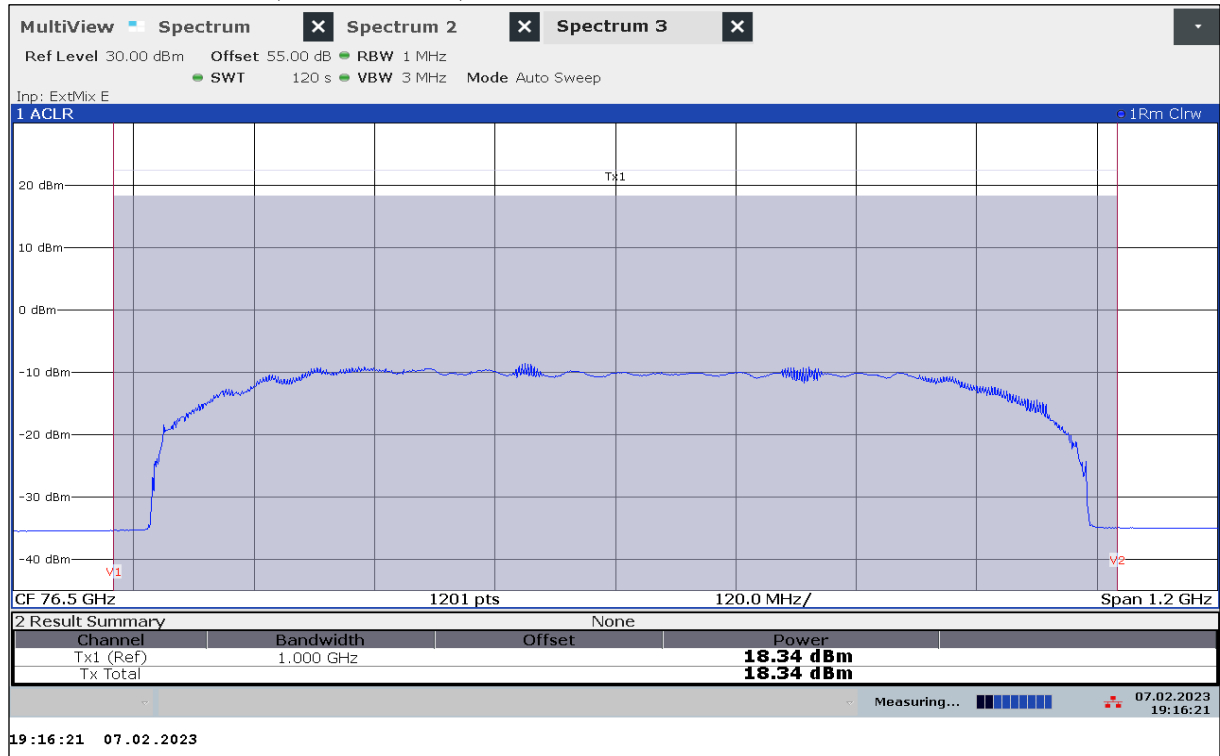
Plot 38: EIRP Mean Power (Channel Power), Mode 45, RMS detector, T_{min} / V_{min-max}
