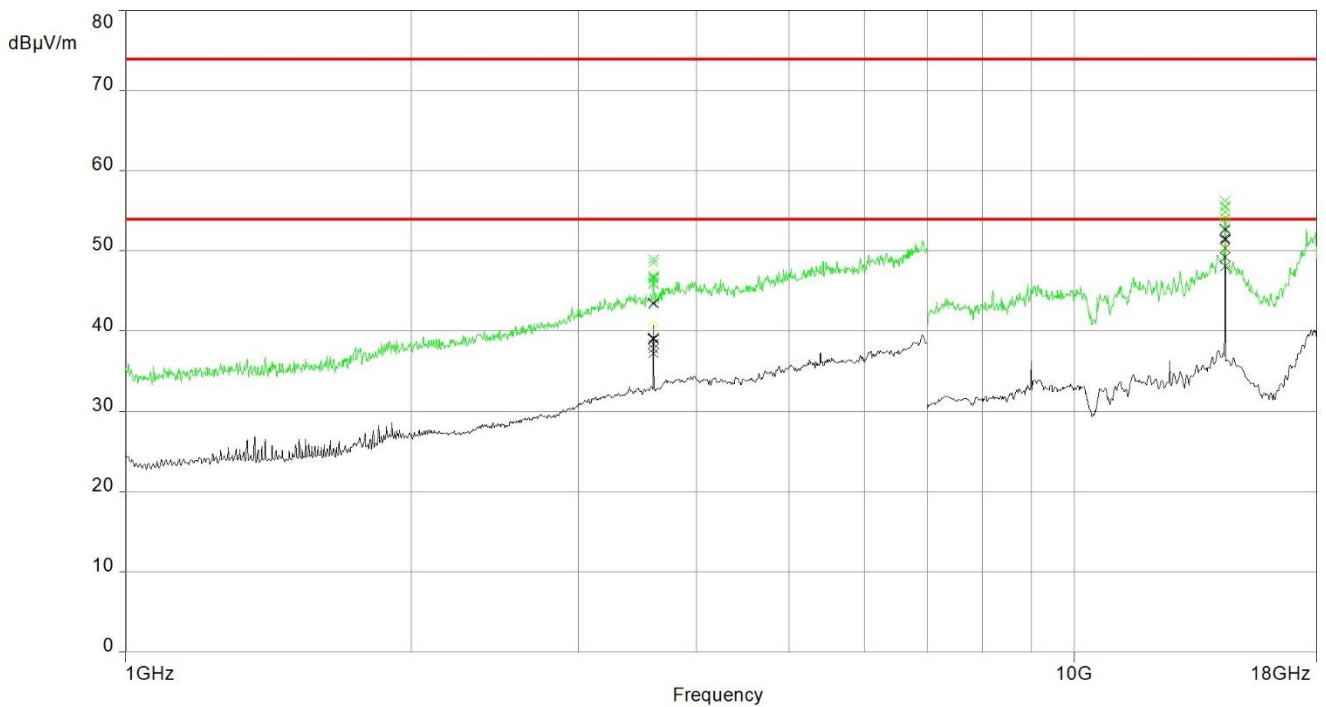
Plot 3: 1 GHz – 18 GHz, DUT4, Mode 01
