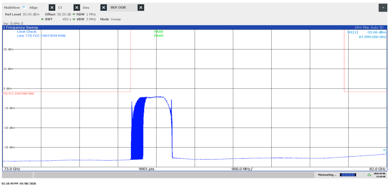
Plot 10: 73 GHz – 82 GHz, including OOB, DUT4, Mode 17
