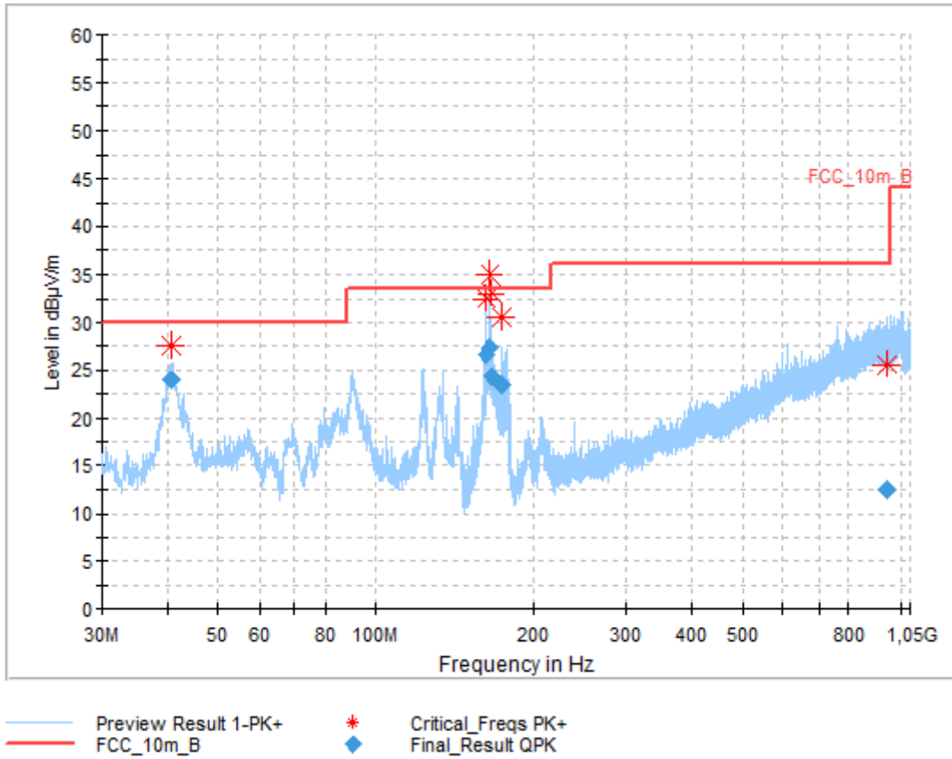
Plot 18: 30 MHz – 1 GHz, DUT4, Mode 4 (c0)
