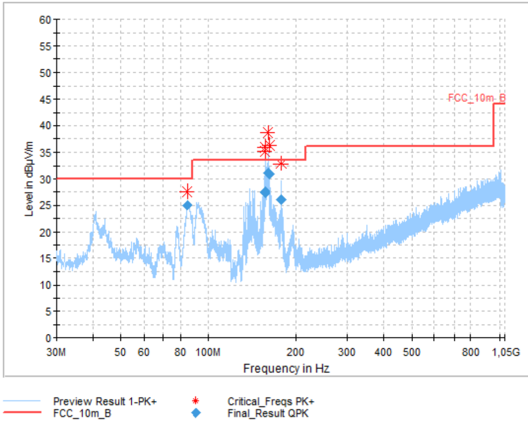
Plot 2: 30 MHz – 1 GHz, DUT4, Mode 01
