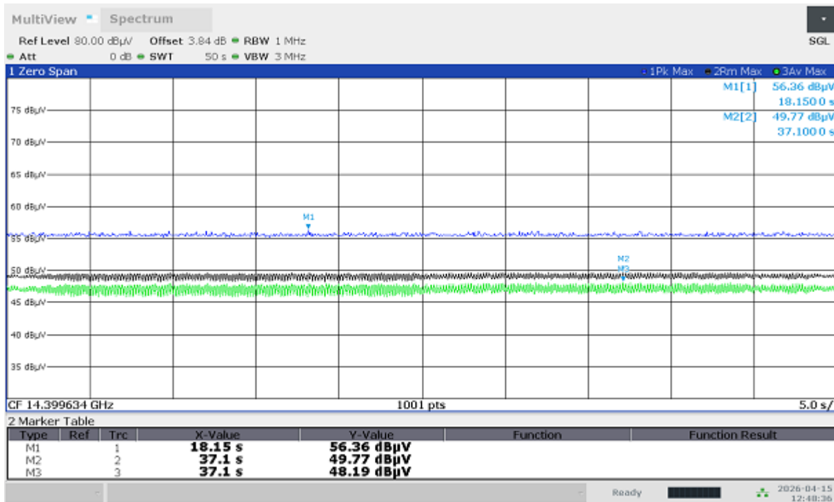
Plot 20: Emission at 14.4 GHz, final zero span measurement, DUT4, Mode 4 (c0)
