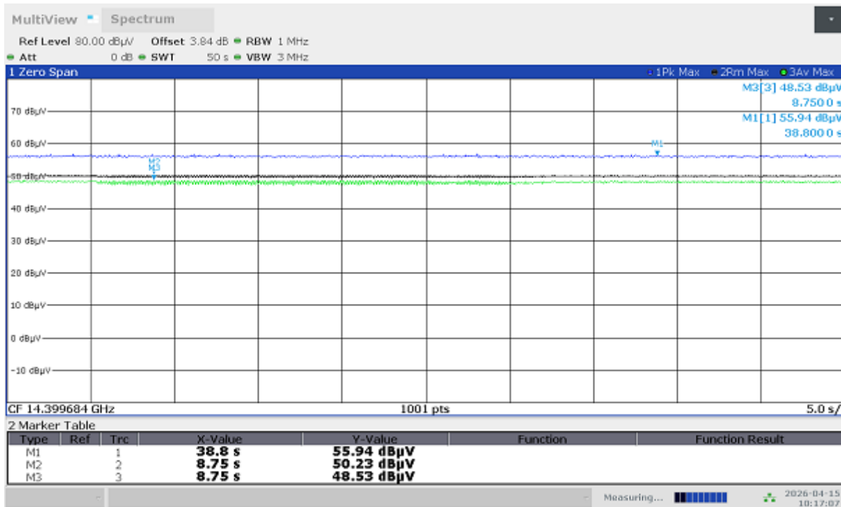
Plot 4: Emission at 14.4 GHz, final zero span measurement, DUT4, Mode 01
