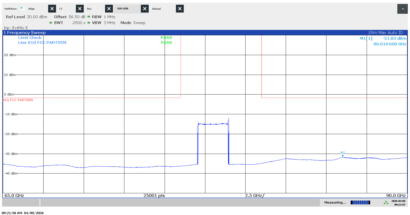
Plot 26: 65 GHz – 90 GHz, including OOB, DUT4, Mode 7 (c0)
