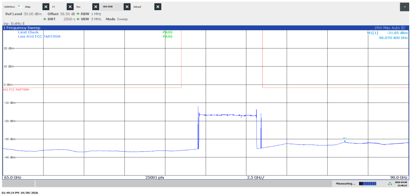
Plot 26: 65 GHz – 90 GHz, including OOB, DUT4, Mode 7 (c0)
