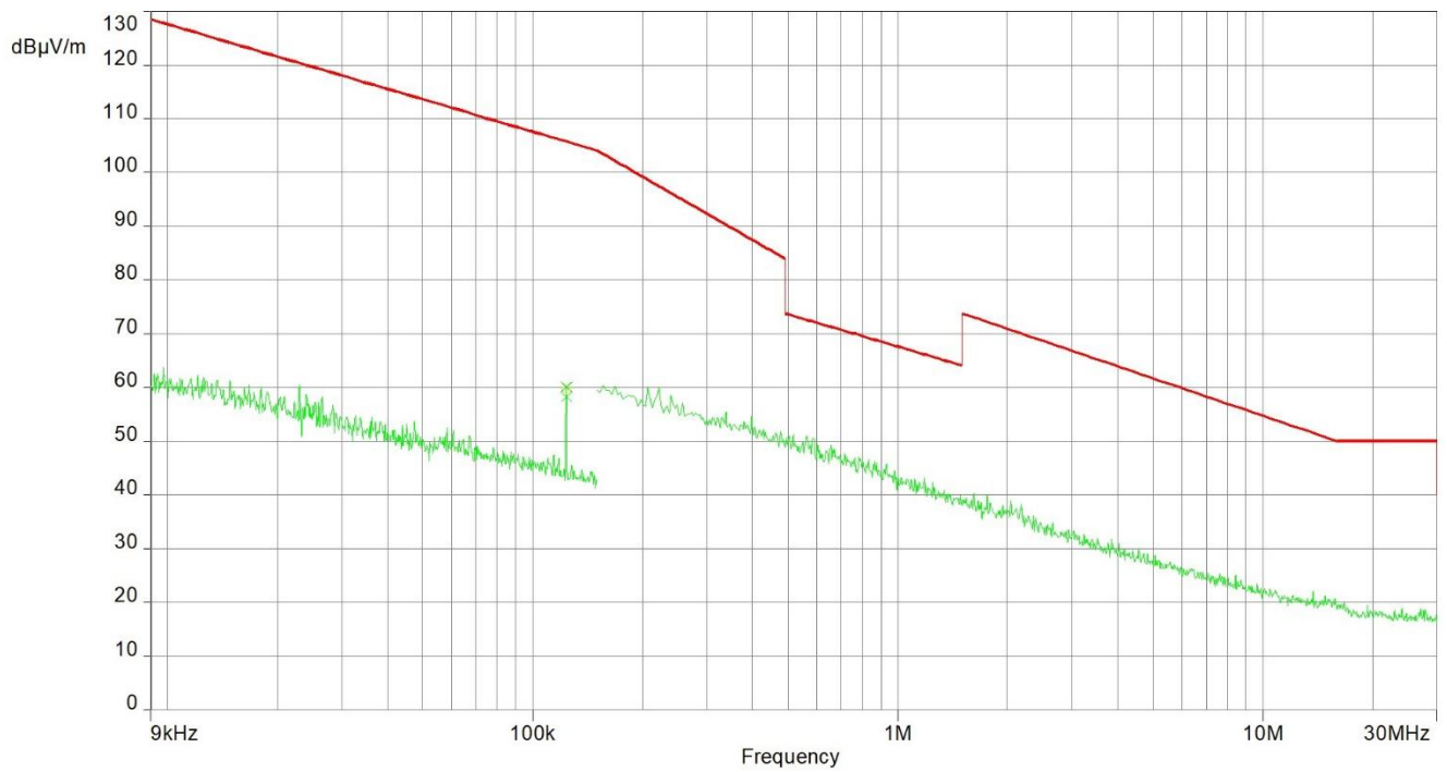
Plot 17: 9 kHz – 30 MHz, DUT4, Mode 4 (c0)
