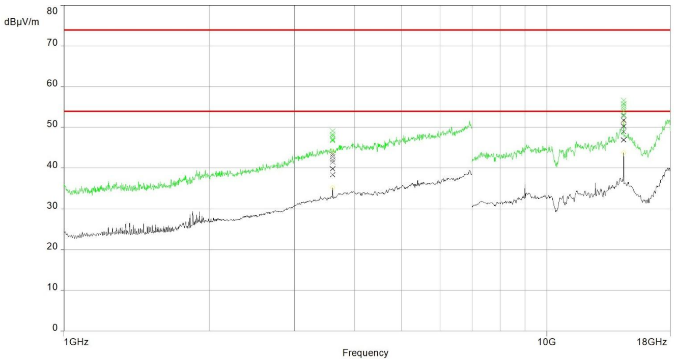
Plot 19: 1 GHz – 18 GHz, DUT4, Mode 4 (c0)
