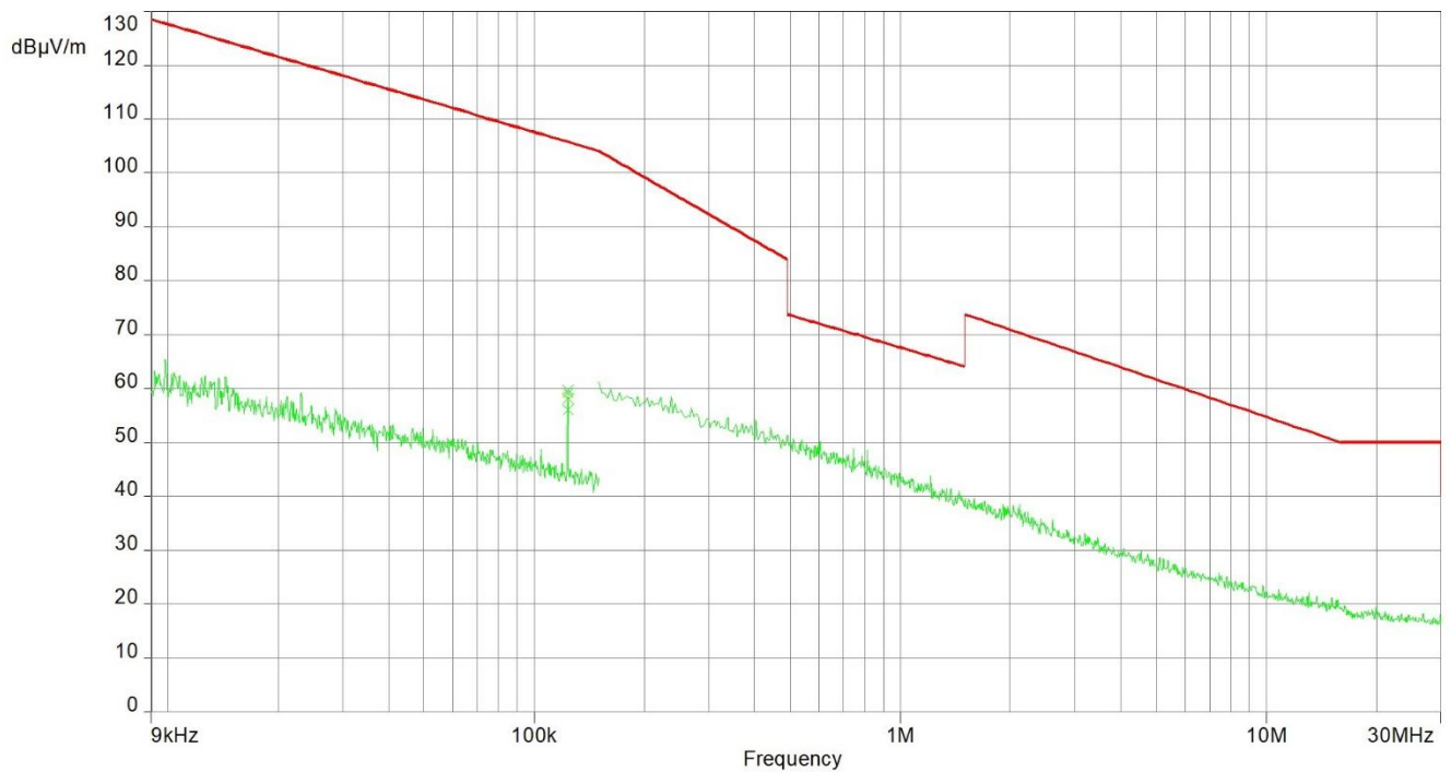
Plot 1: 9 kHz – 30 MHz, DUT4, Mode 01
