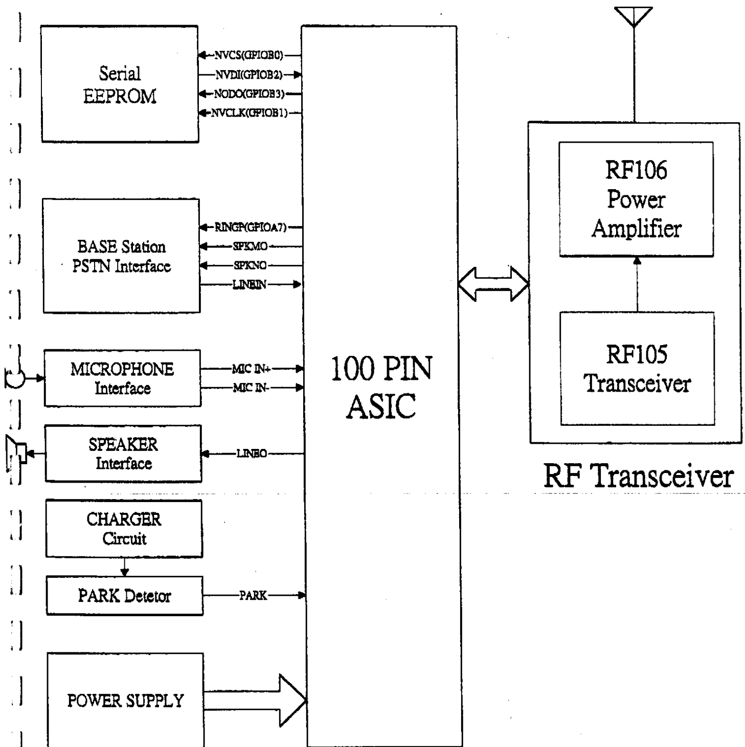
System Block Diagram for DCT-2000 Base Station
