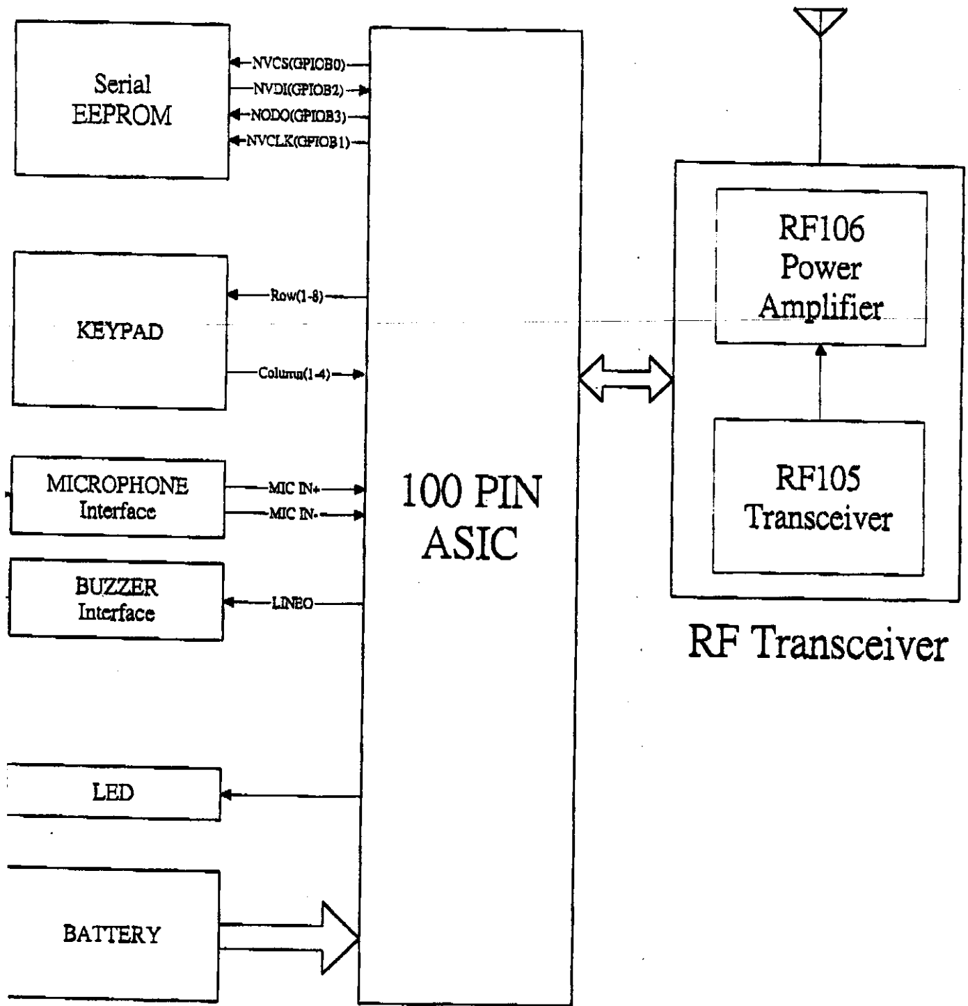
System Block Diagram for DCT-2000 Handset
