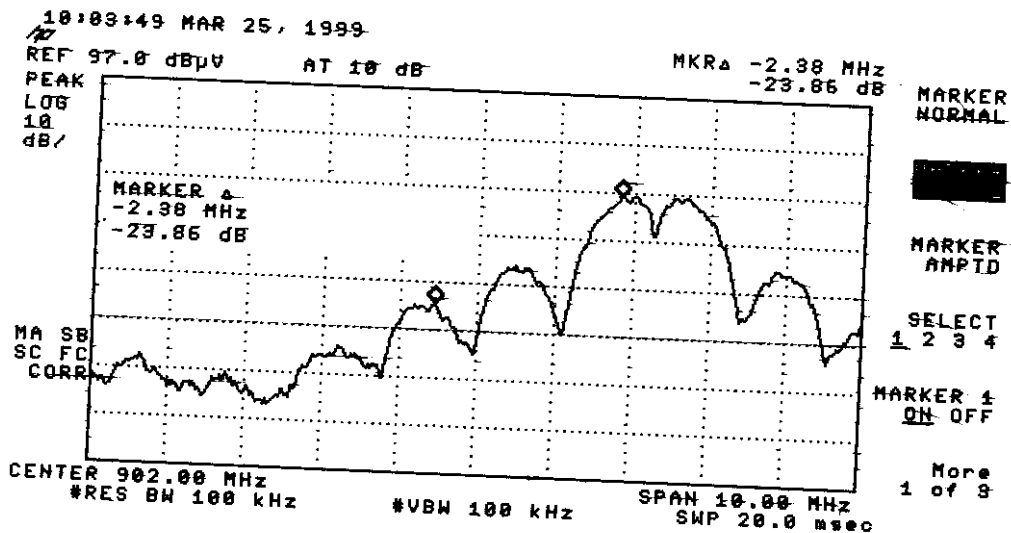
Handset CH01
