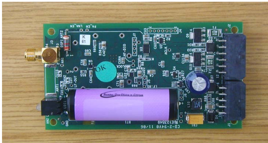
Figure 2 PCB Side 2
