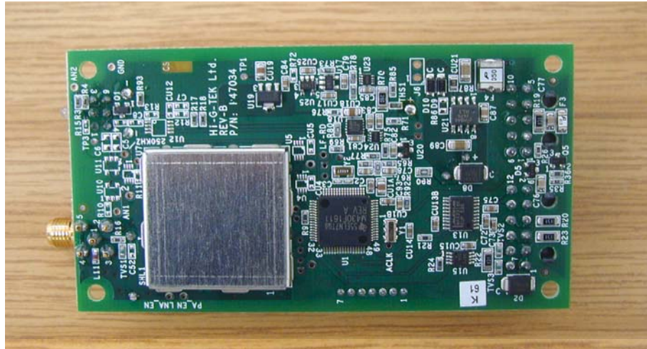
Figure 1 PCB Side 1
