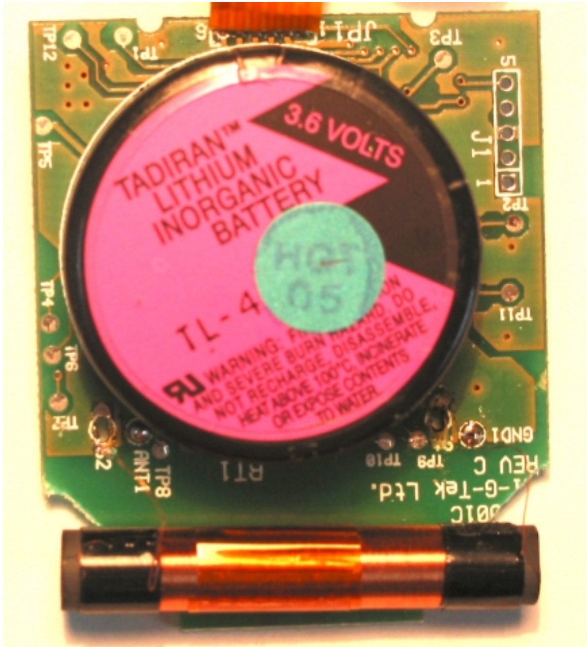
Digital PCB, printed side
