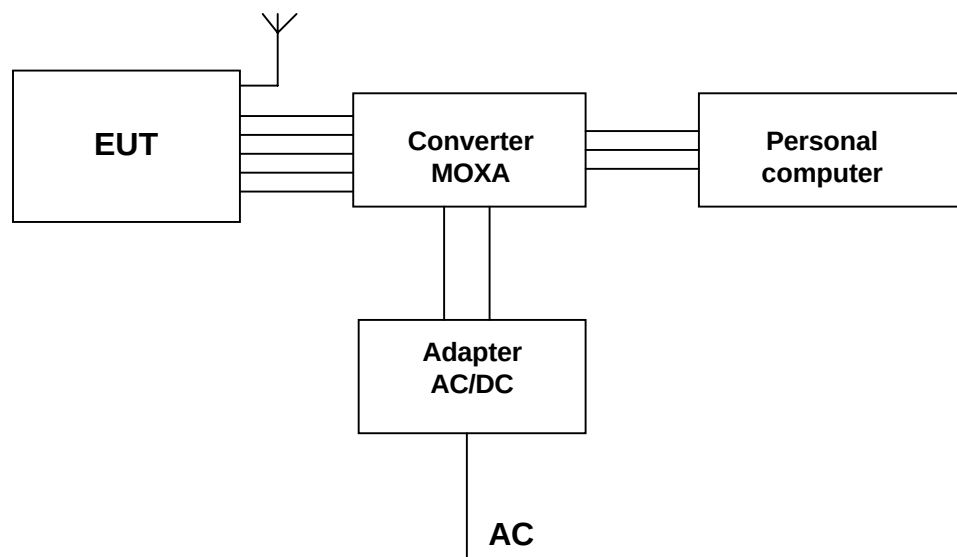
b) Conducted emission test configuration
