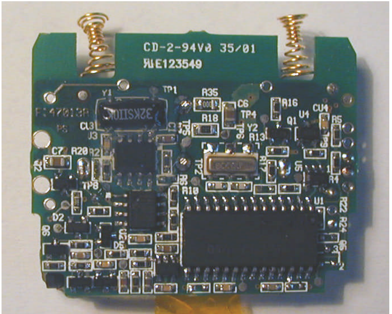
Photograph No.2 PCB printed side
