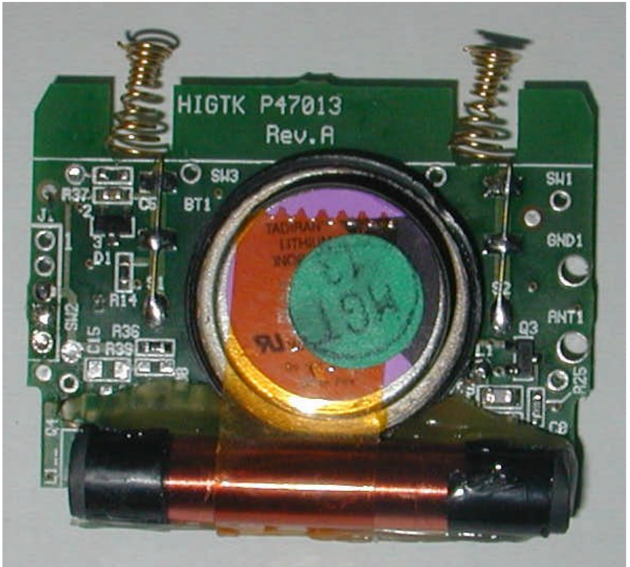
Photograph No.1 PCB component side
