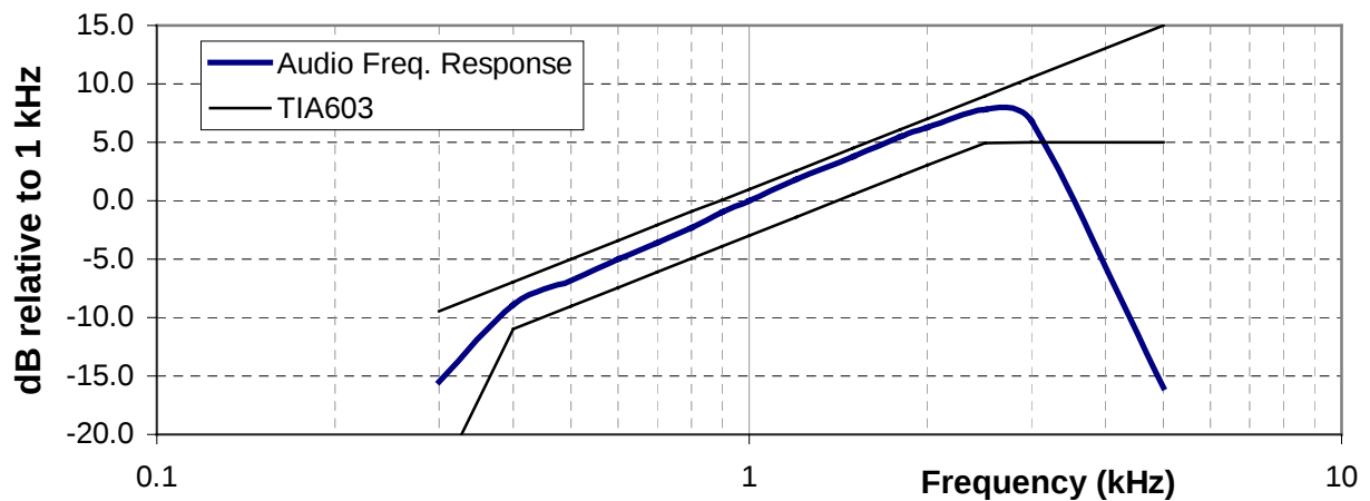
Transmitter Audio Frequency Response
