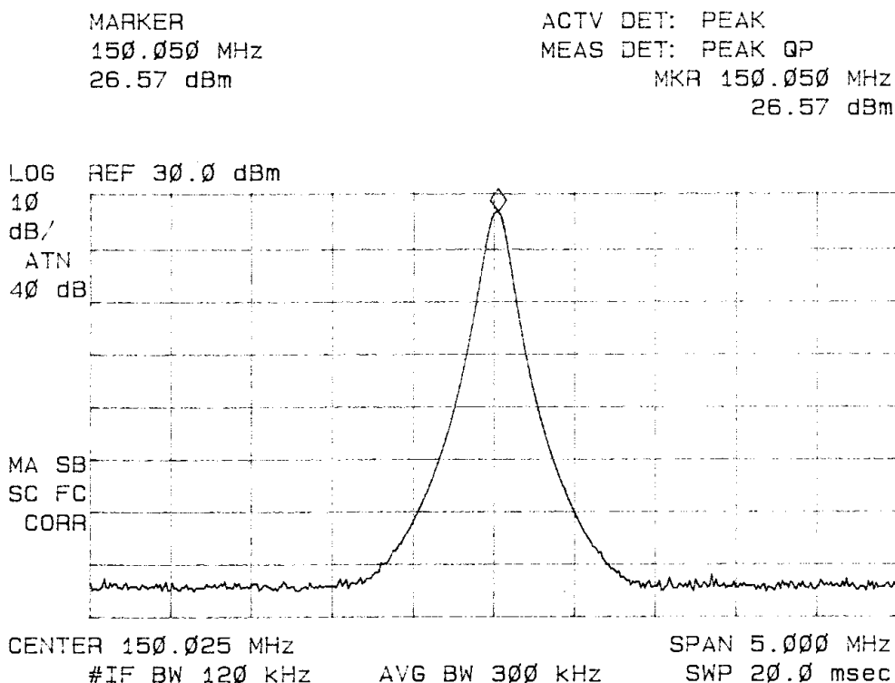
Figure 1: Power Output Channel 150.025
