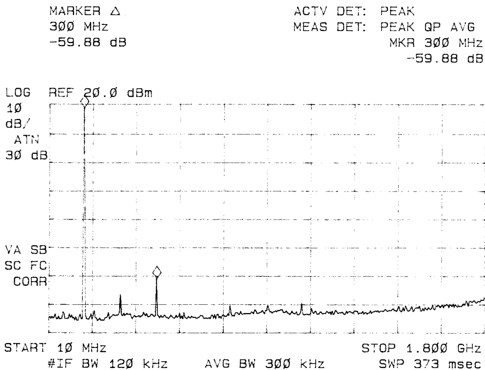
Figure 9: Emissions at Antenna Terminal (150.025 MHz)
