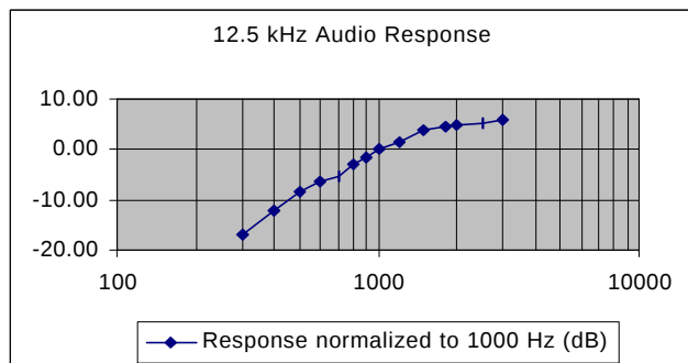
Figure 4: Audio Response Characteristics.
