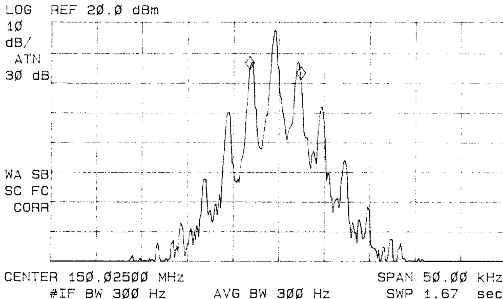
Figure 7: Occupied Band Width, Channel Width 12.5 kHz
