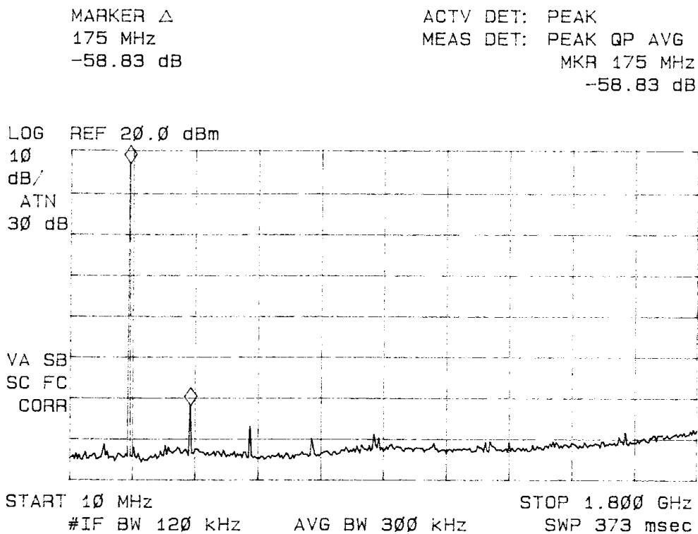
Figure 10: Emissions at Antenna Terminal(173.9875 MHz)
