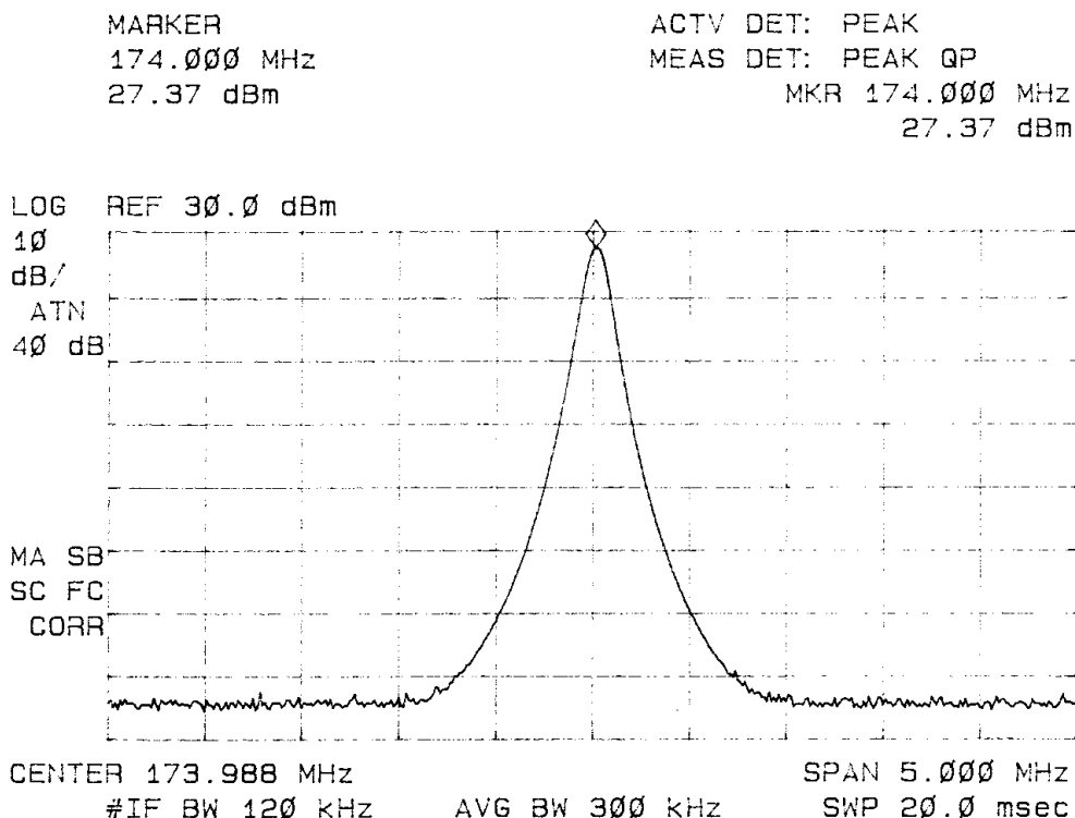
Figure 3: Power Output Channel 173.9875
