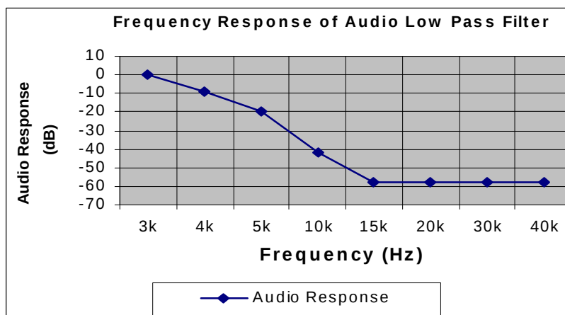
Figure 6: Frequency Response of Audio low Pass Filter.
