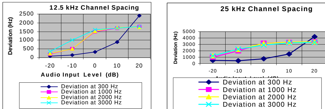
Figure 5: Deviation Characteristics.
