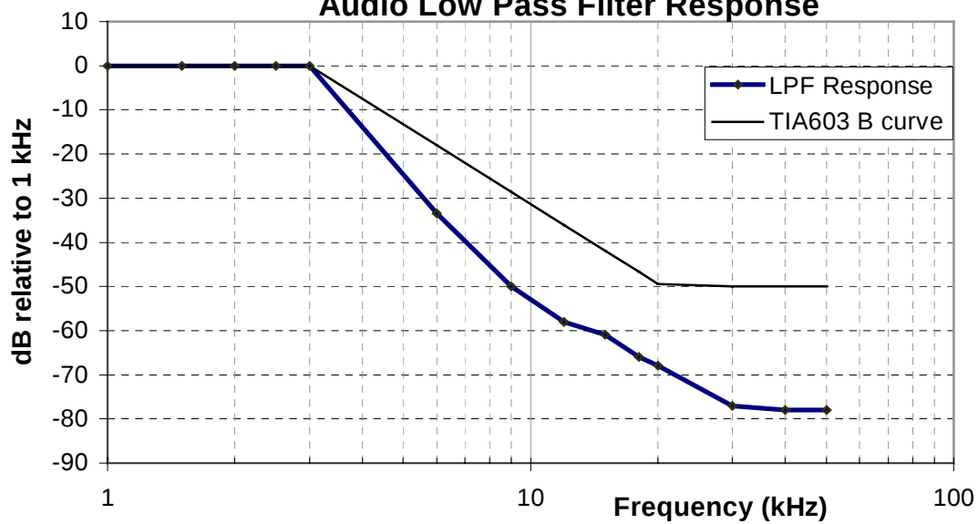
Audio Low Pass Filter Response
