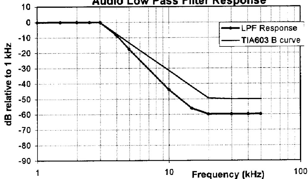
Audio Low Pass Filter Response
