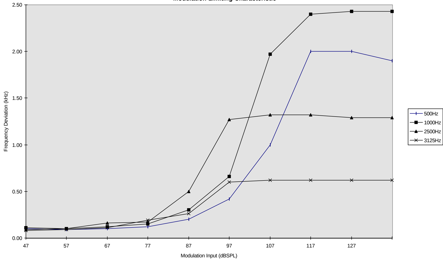
Modulation Limiting Characteristic
