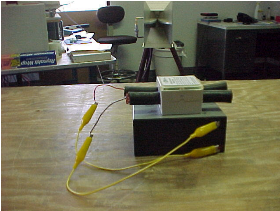
RADIATED EMISSIONS PRE-SCAN - REAR OF UNIT
