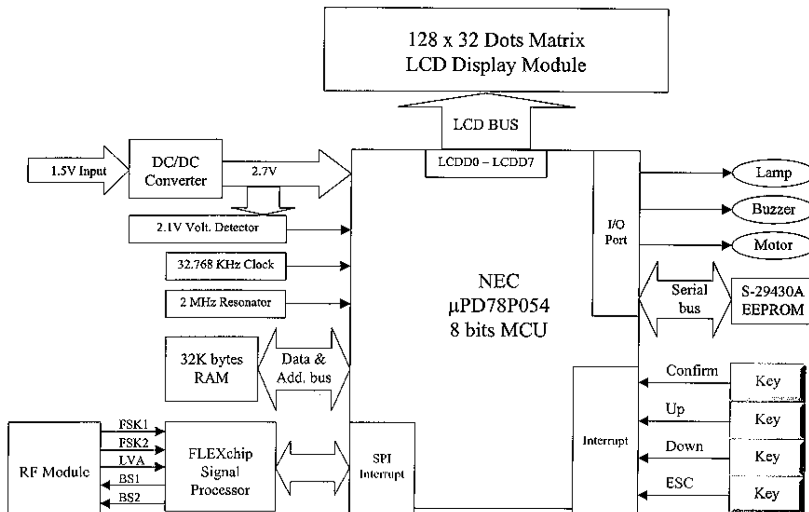
Figure 1 Block diagram of 6011N digital module
