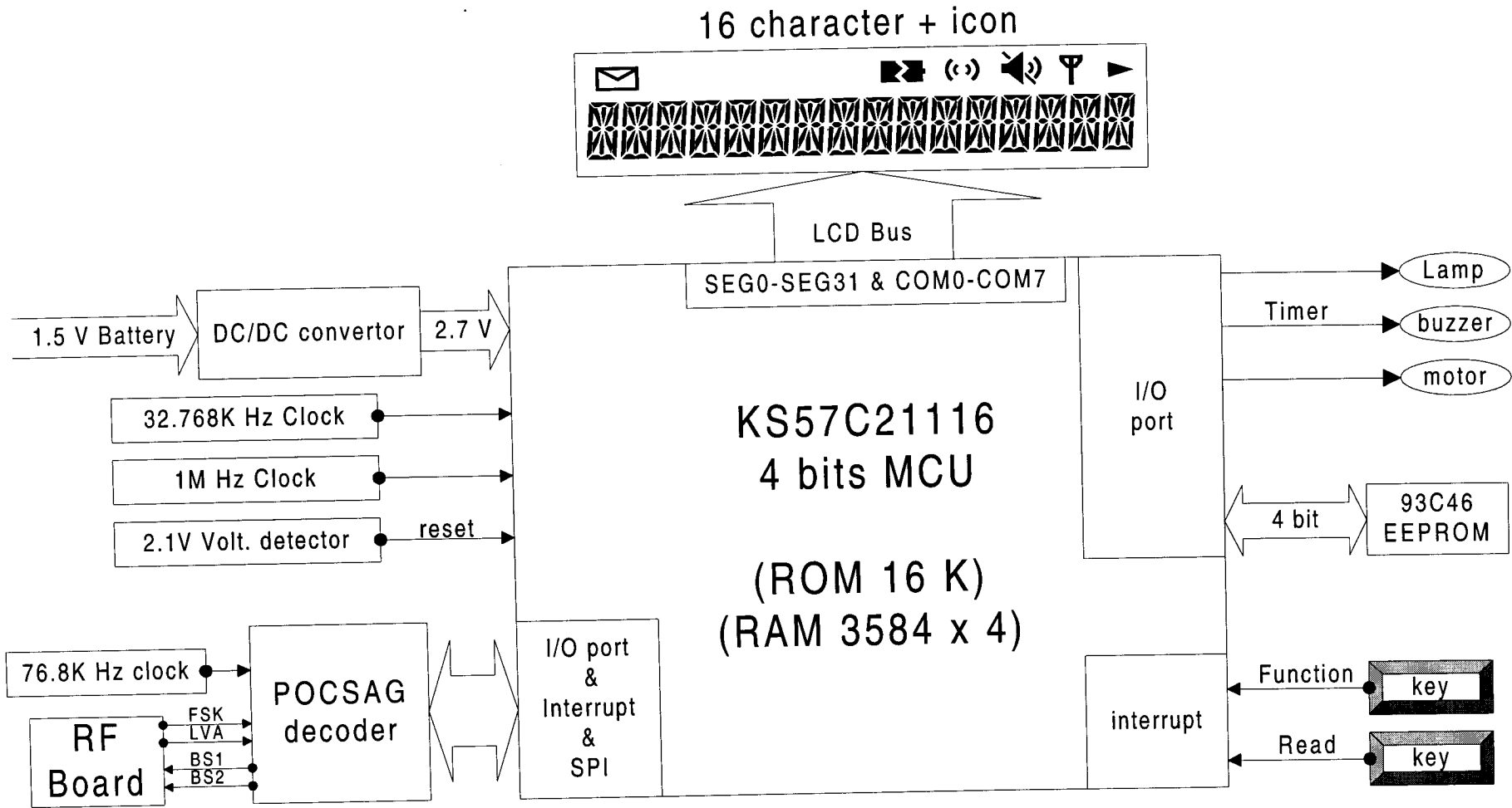
Block diagram of 6015N digital board
