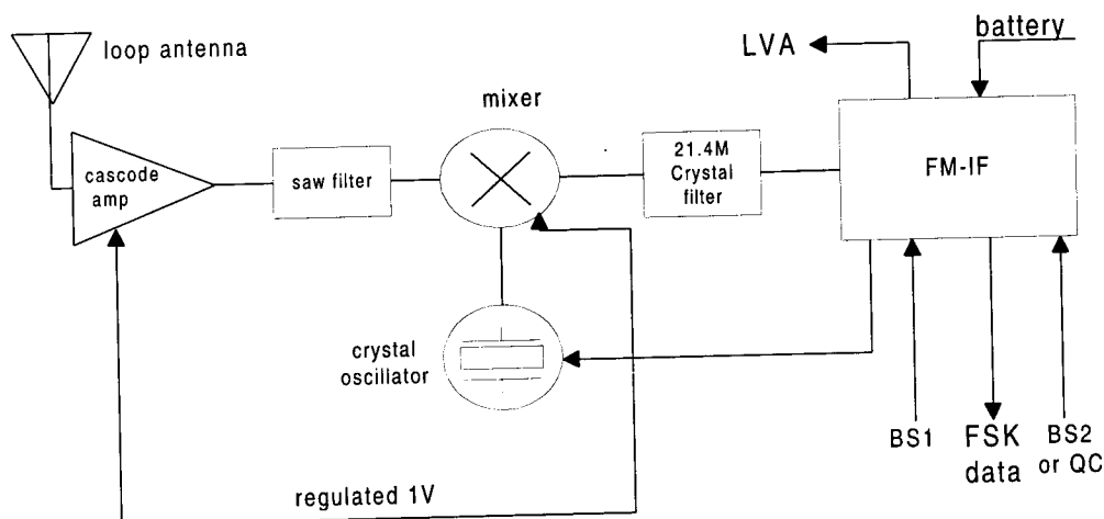
Figure 1: Block diagram of 2-level FSK RF demodulation architecture.
