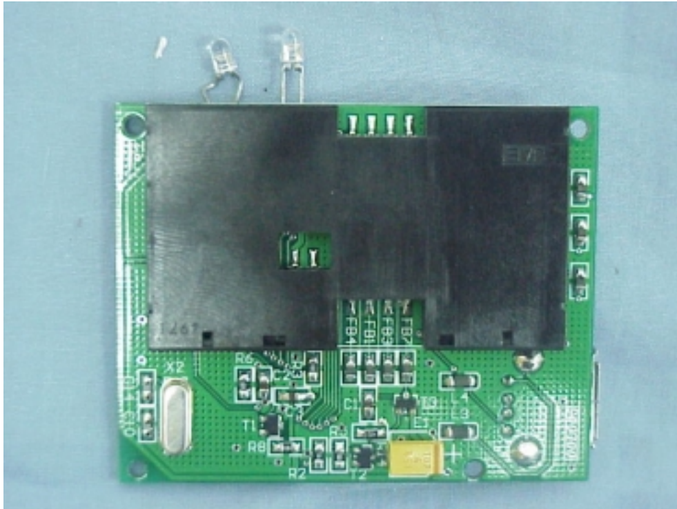
Figure 3 Smart Card Reader (M/N: ARUSB2000) MAIN BOARD (SOLDERED SIDE)
