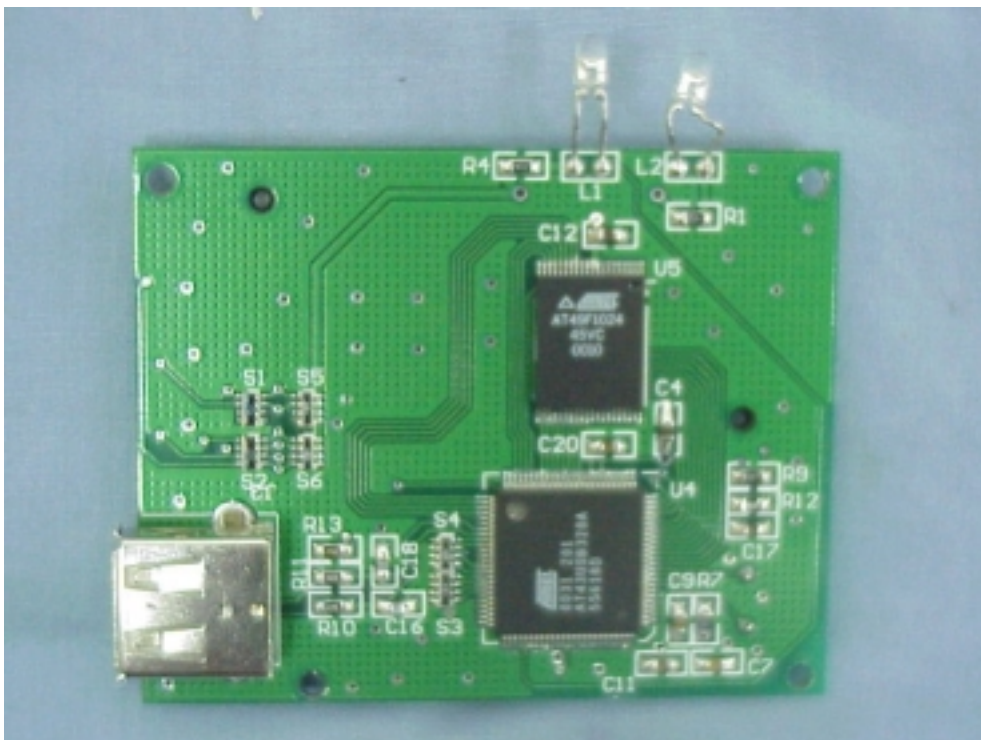
Figure 2 Smart Card Reader (M/N: ARUSB2000) MAIN BOARD (COMPONENT SIDE)
