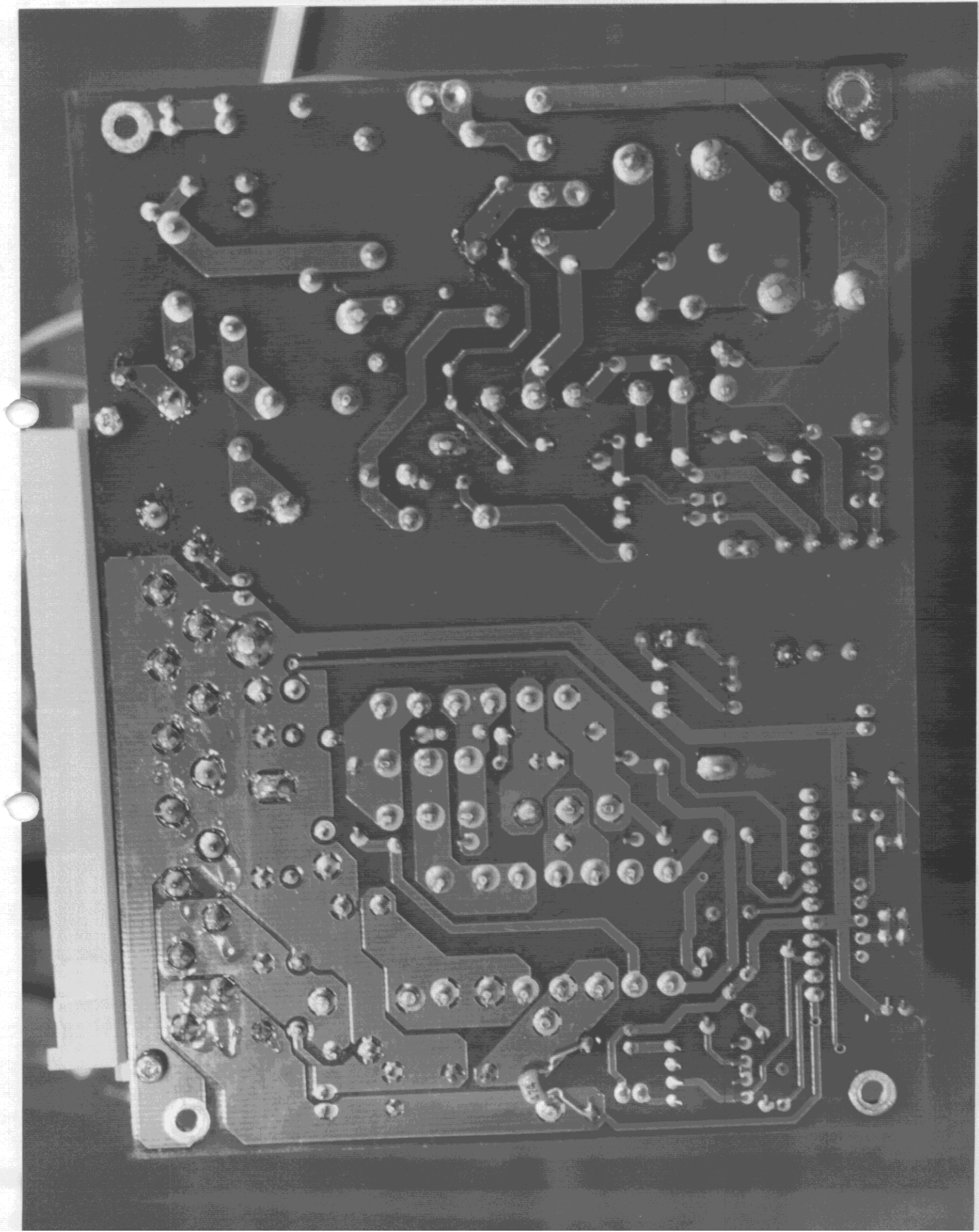
PHOTO 26. POWER SUPPLY SOLDERING SIDE VIEW
