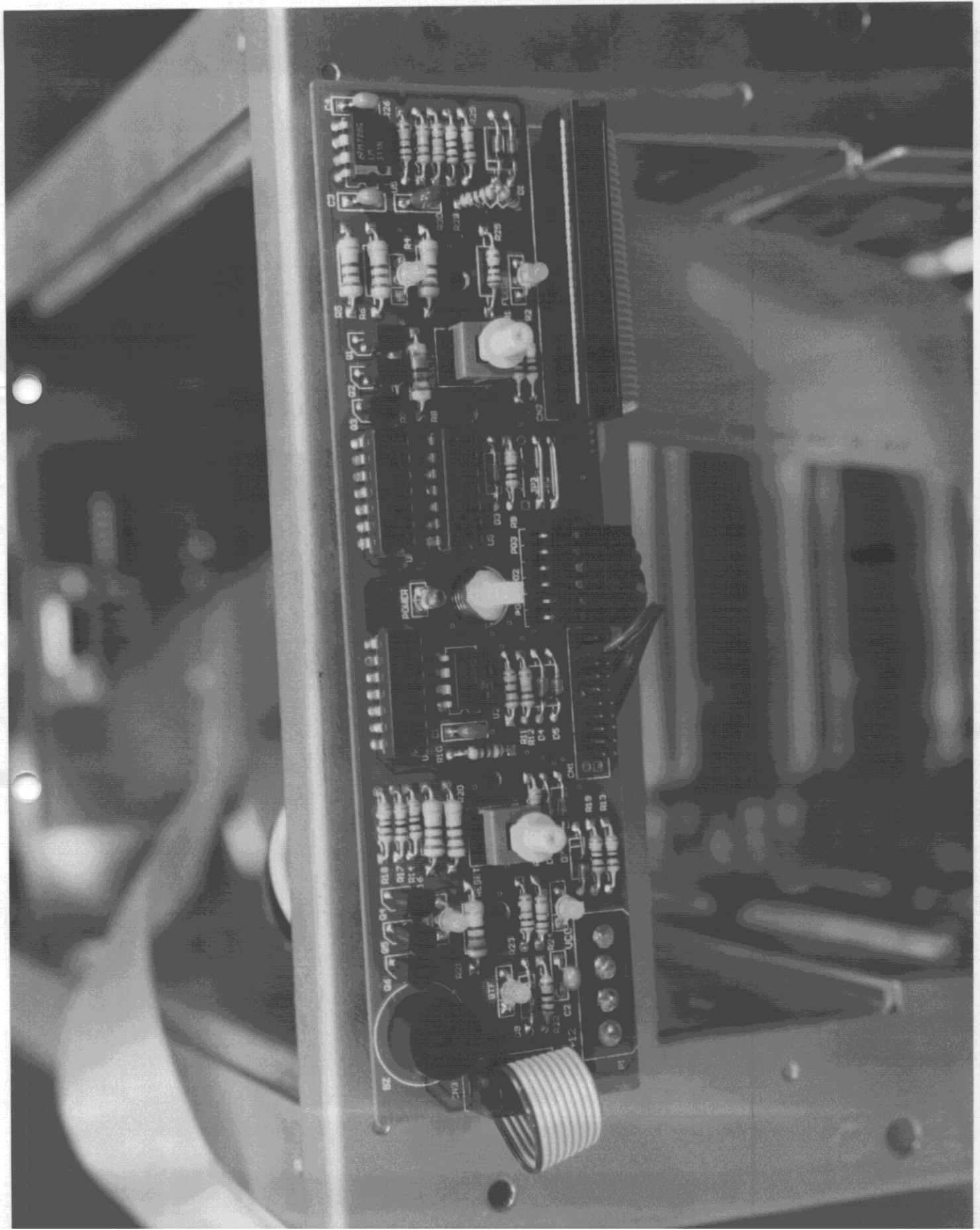
PHOTO 18. EUT COMPONENT SIDE VIEW
