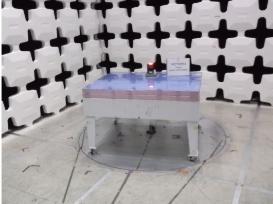
Radiated Test Setup – Front
