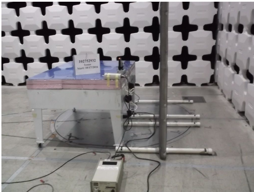
Conducted Test Setup – Side
