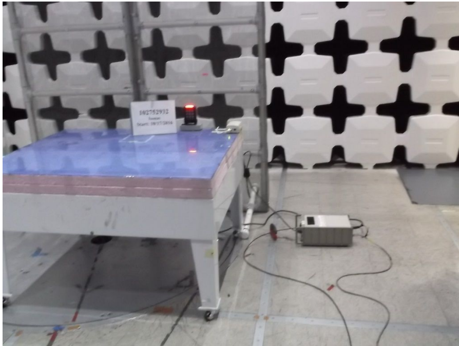
Conducted Test Setup – Front
