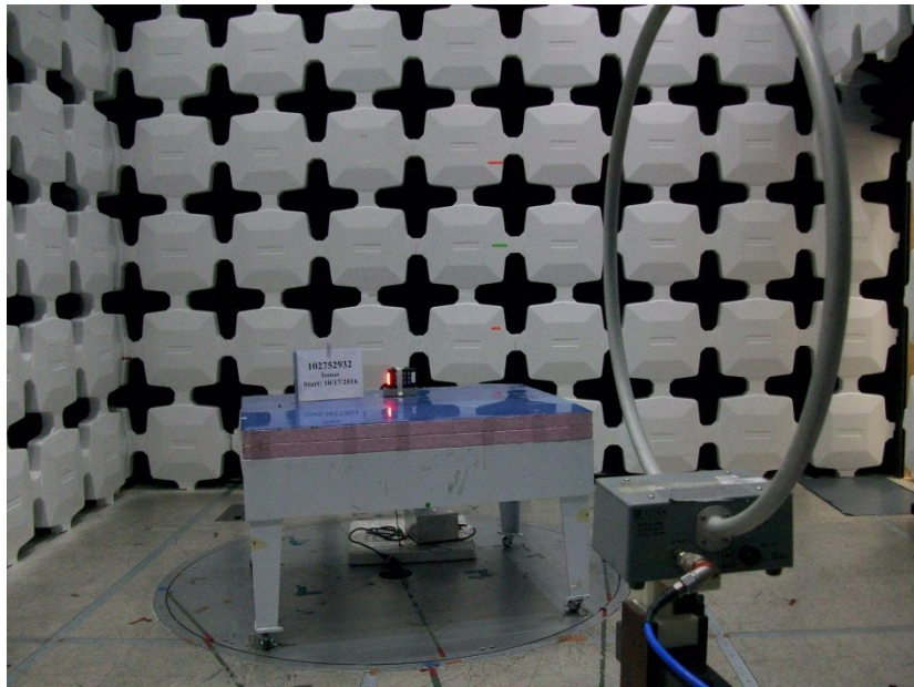
Radiated Test Setup – Front (9kHz – 30MHz)
