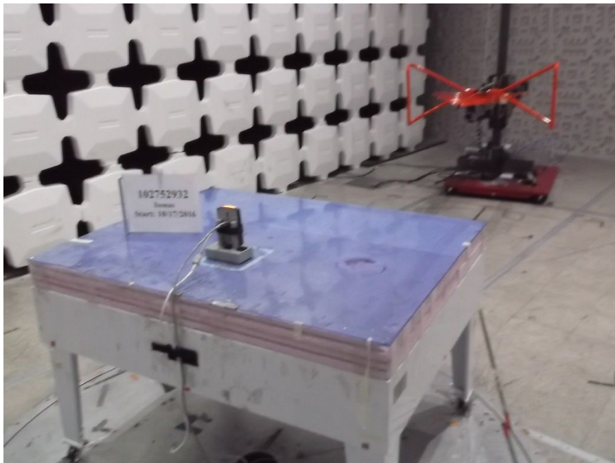
Radiated Test Setup – Rear (30MHz – 1GHz)
