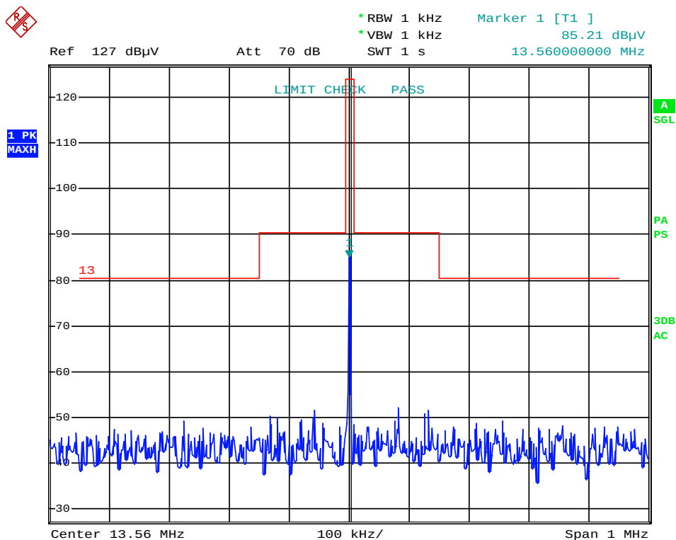
Figure 4: Spectrum Mask
