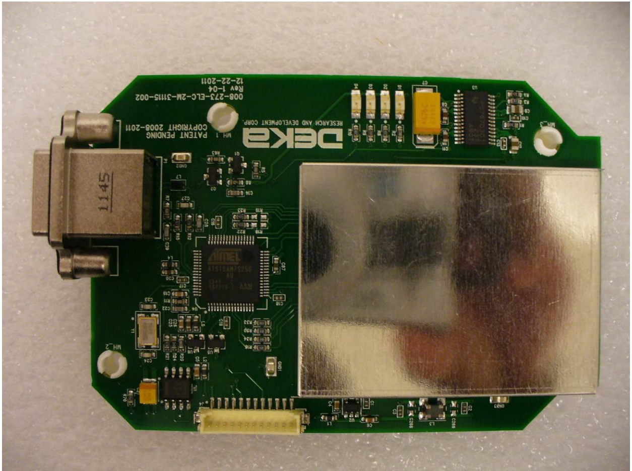
Figure 7: RFID Reader with Shield – Top
