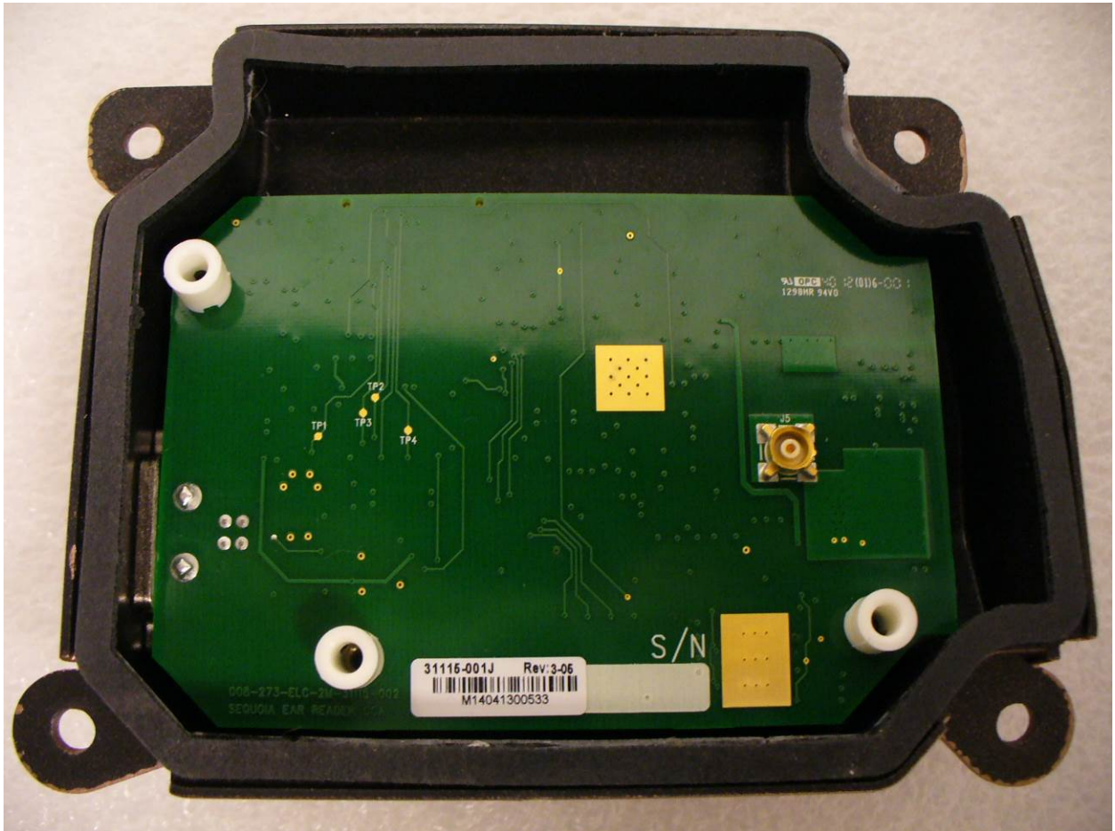
Figure 5: RFID Reader Board Assembled
