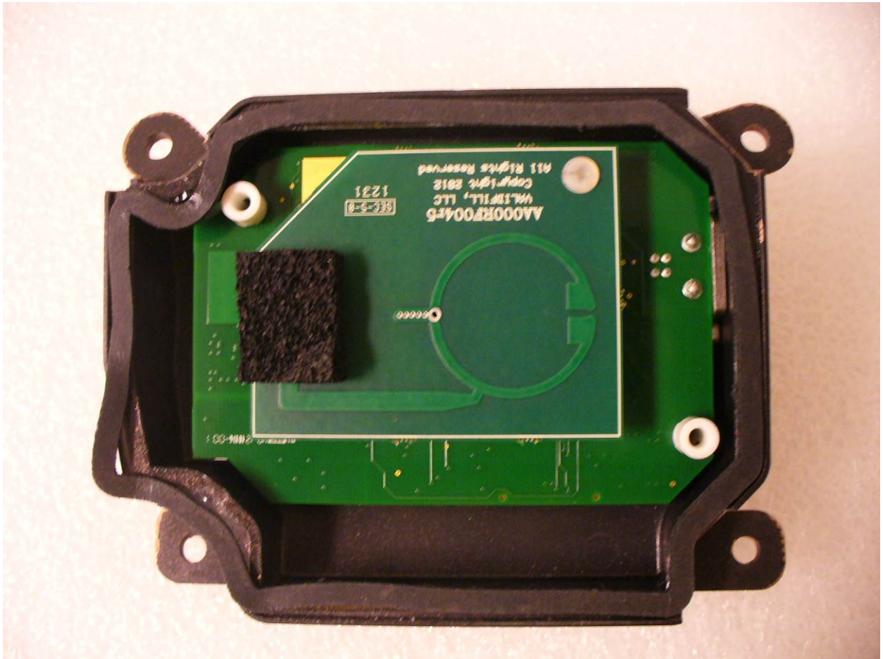
Figure 4: RFID Reader Antenna Assembled
