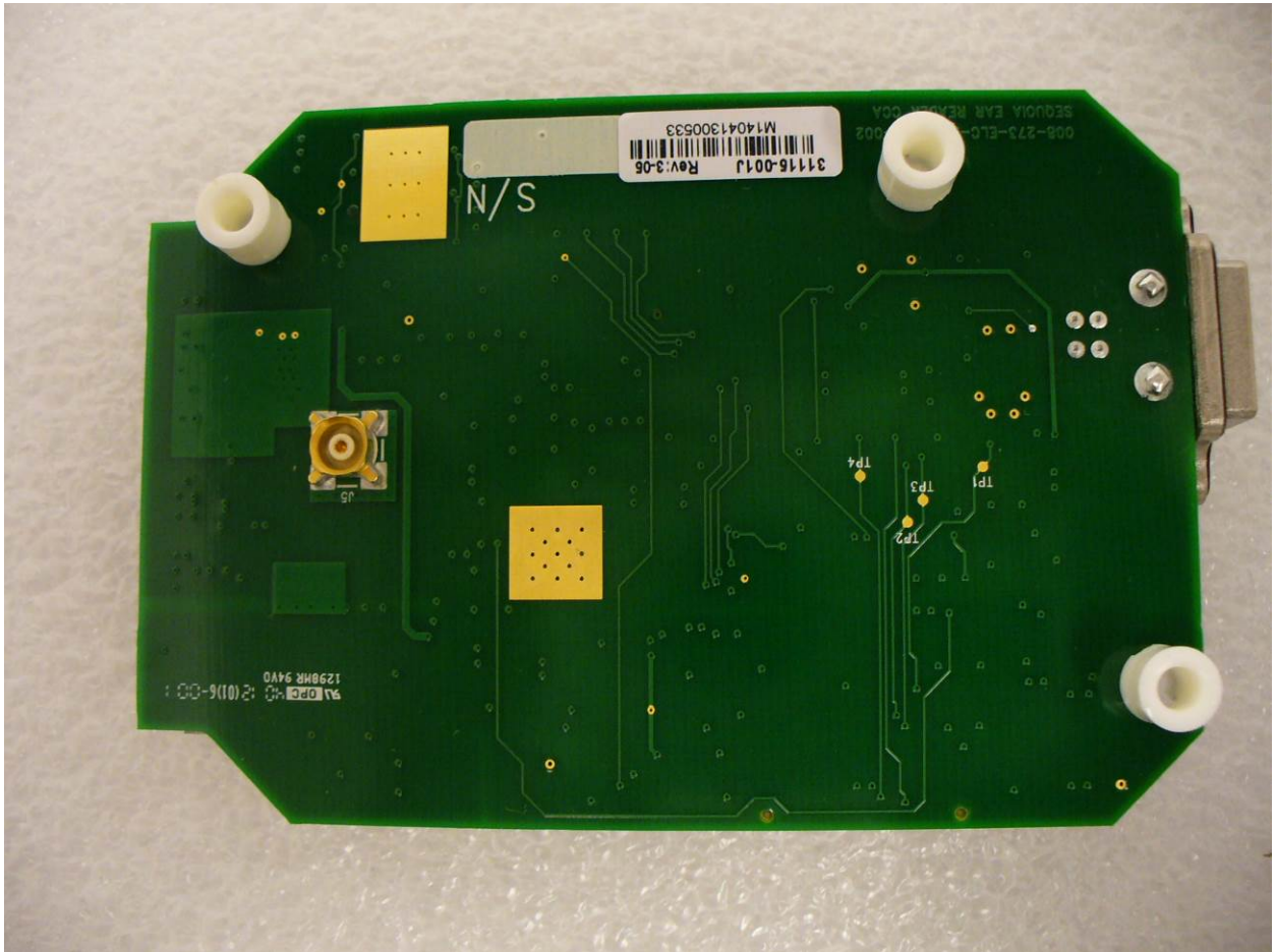
Figure 9: RFID Reader – Bottom
