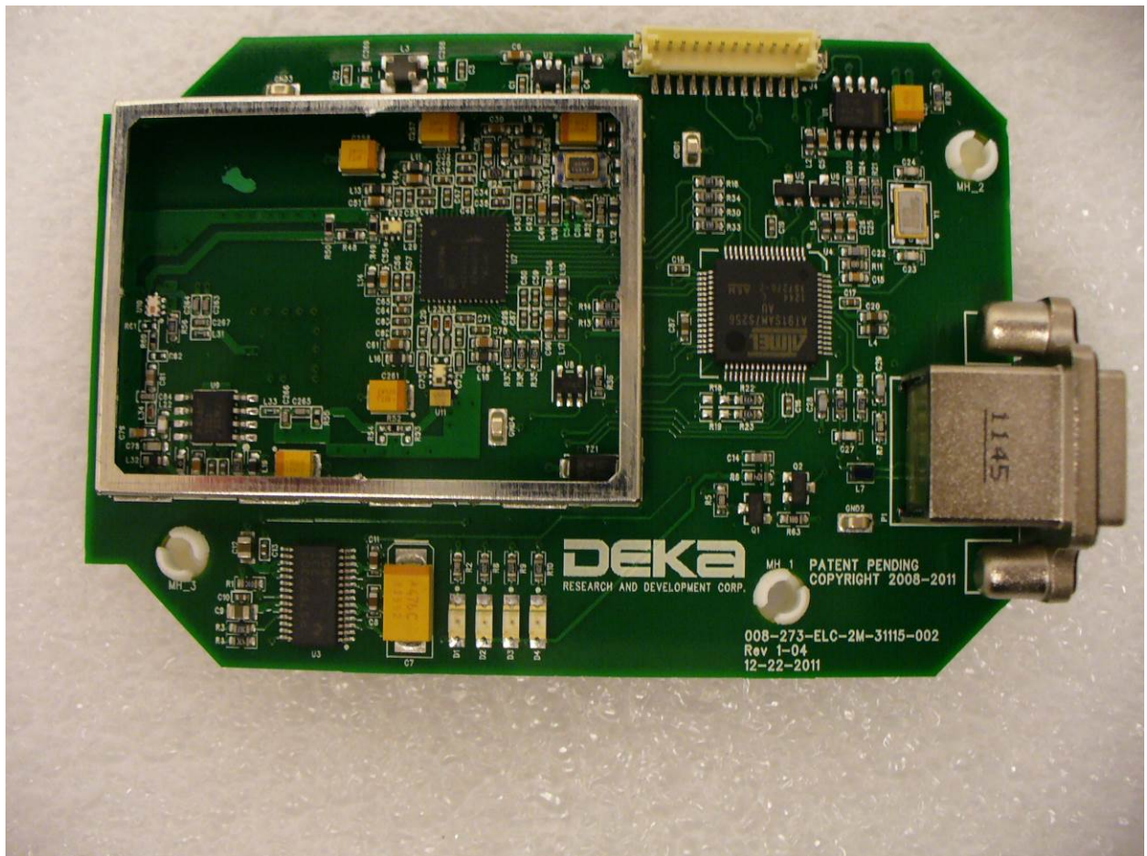
Figure 8: RFID Reader without Shield – Top
