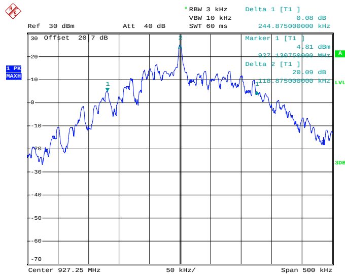
Figure 7.3.4.2-8: 20 dB BW – Middle Channel - Antenna port 1
