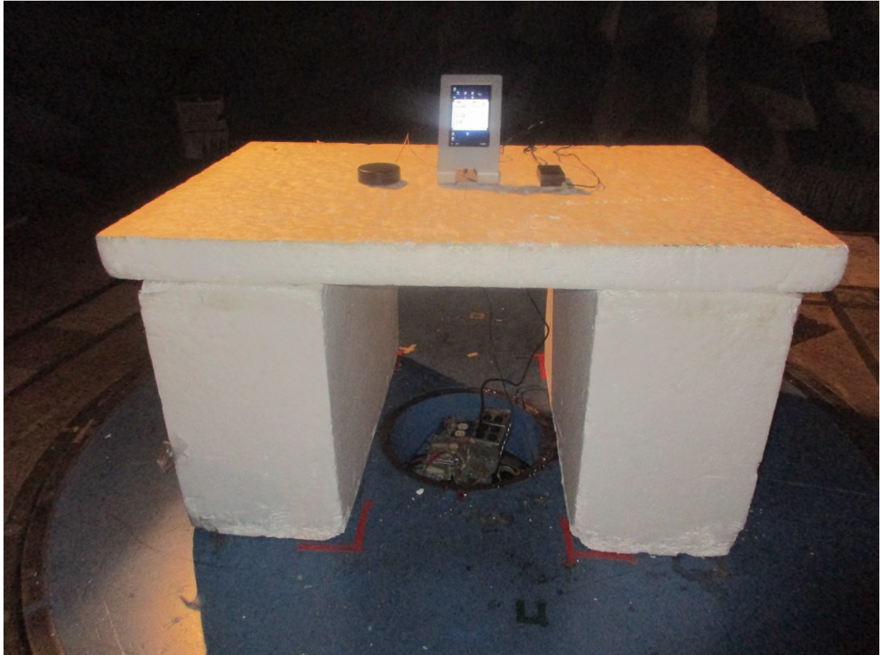
Figure 1: Radiated Emissions – below 1 GHz – Front View
