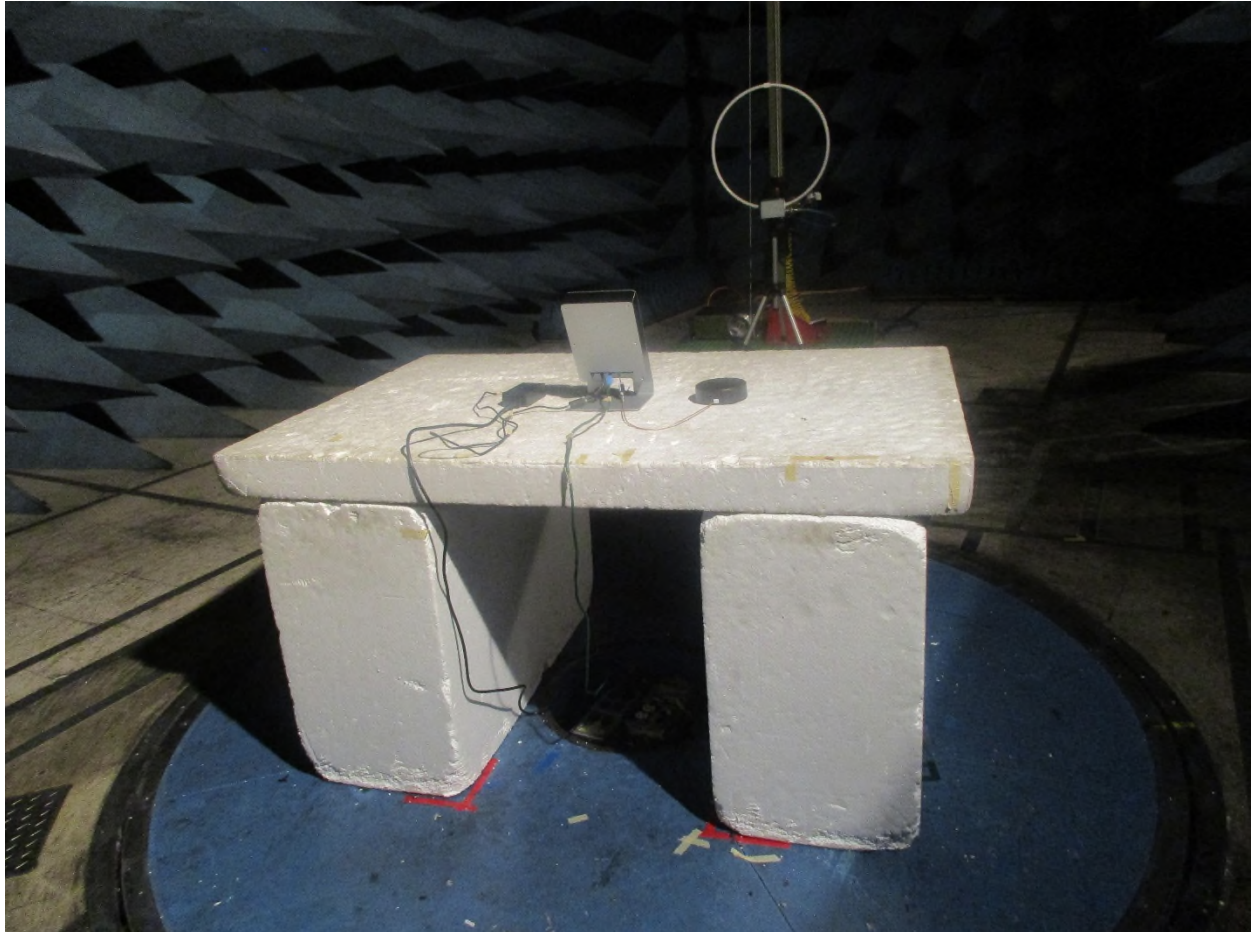
Figure 2: Radiated Emissions – 9 kHz – 30 MHz – Rear View
