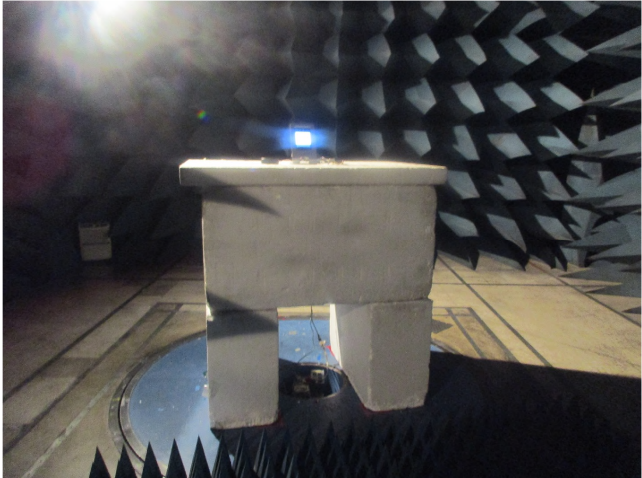
Figure 5: Radiated Emissions – above 1 GHz – Front View
