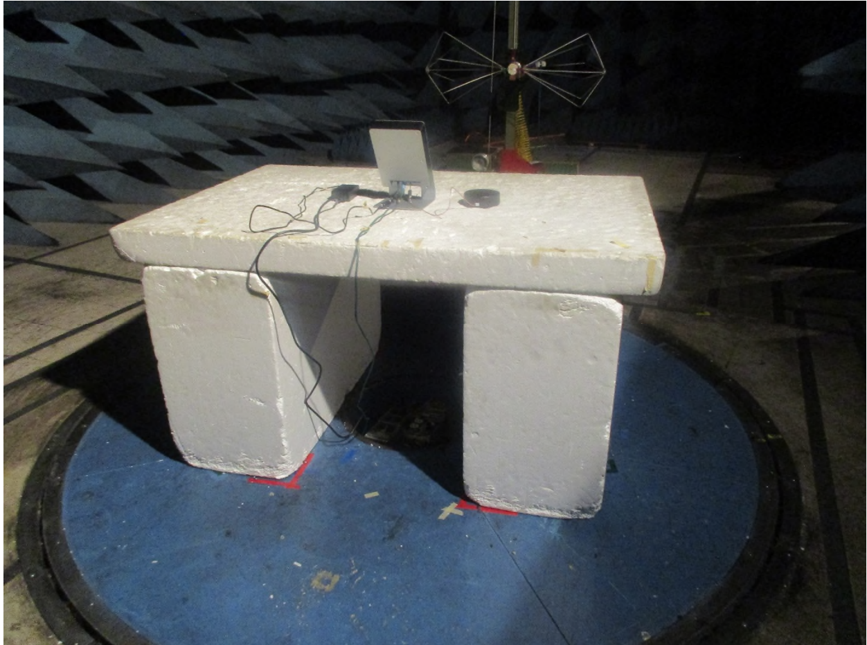
Figure 3: Radiated Emissions – 30 MHz – 200 MHz – Rear View
