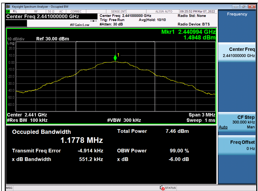
Test_Graph_LE1M_ANT1_2441_1Mbps_DTSBW
