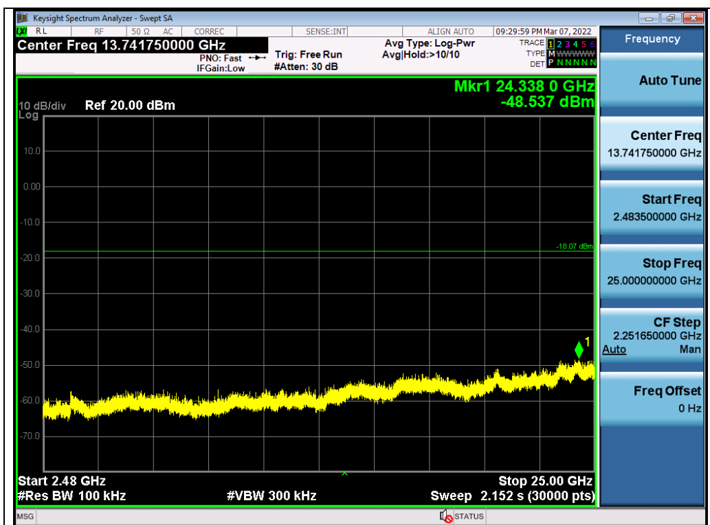
Test_Graph_LE1M_ANT1_2404_1Mbps_Higher Band Emissions
