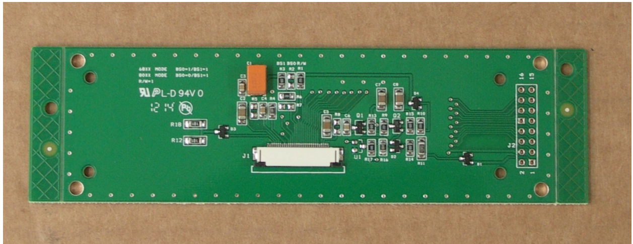
OLED INTERFACE TOP
