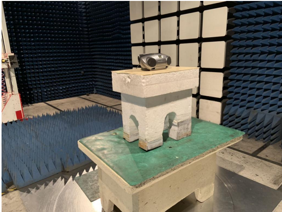
Photograph 5: Set-up for Radiated Spurious Emission, Ab ove 1GHz
