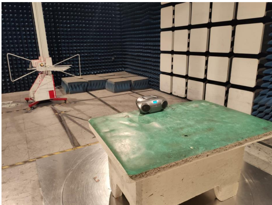
Photograph 4: Set-up for Radiated Spurious Emission, Up to 1GHz
