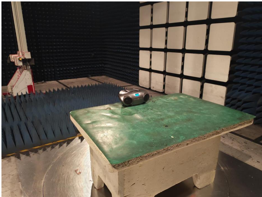
Photograph 3: Set-up for Radiated Emission, 1GHz - 6GHz
