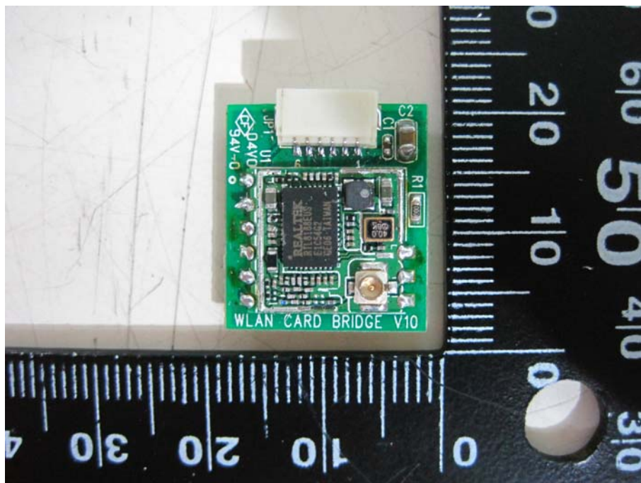
Front View of the WIFI Module-1
