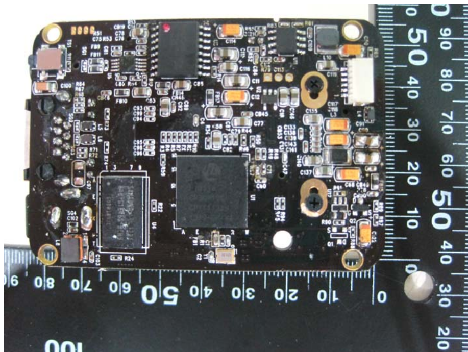
Rear View of the EUT's PCB-1-1
