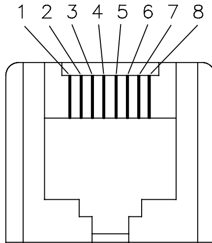
Figure A-1 Plug Pin Locations
