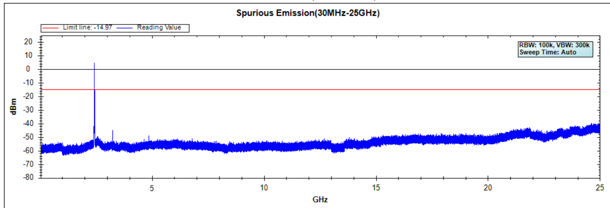
Channel 11 (2462MHz)
