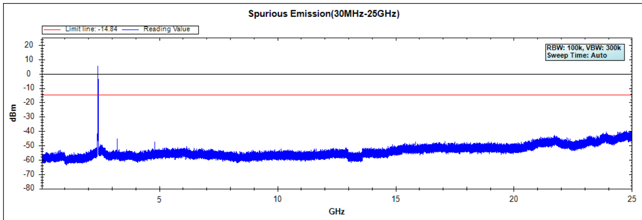
Channel 06 (2437MHz)
