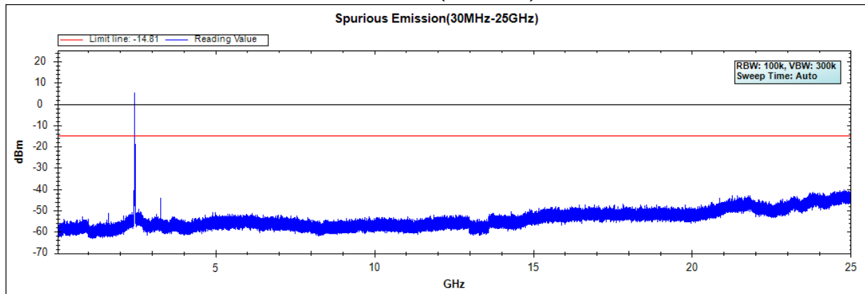
Channel 11 (2462MHz)
