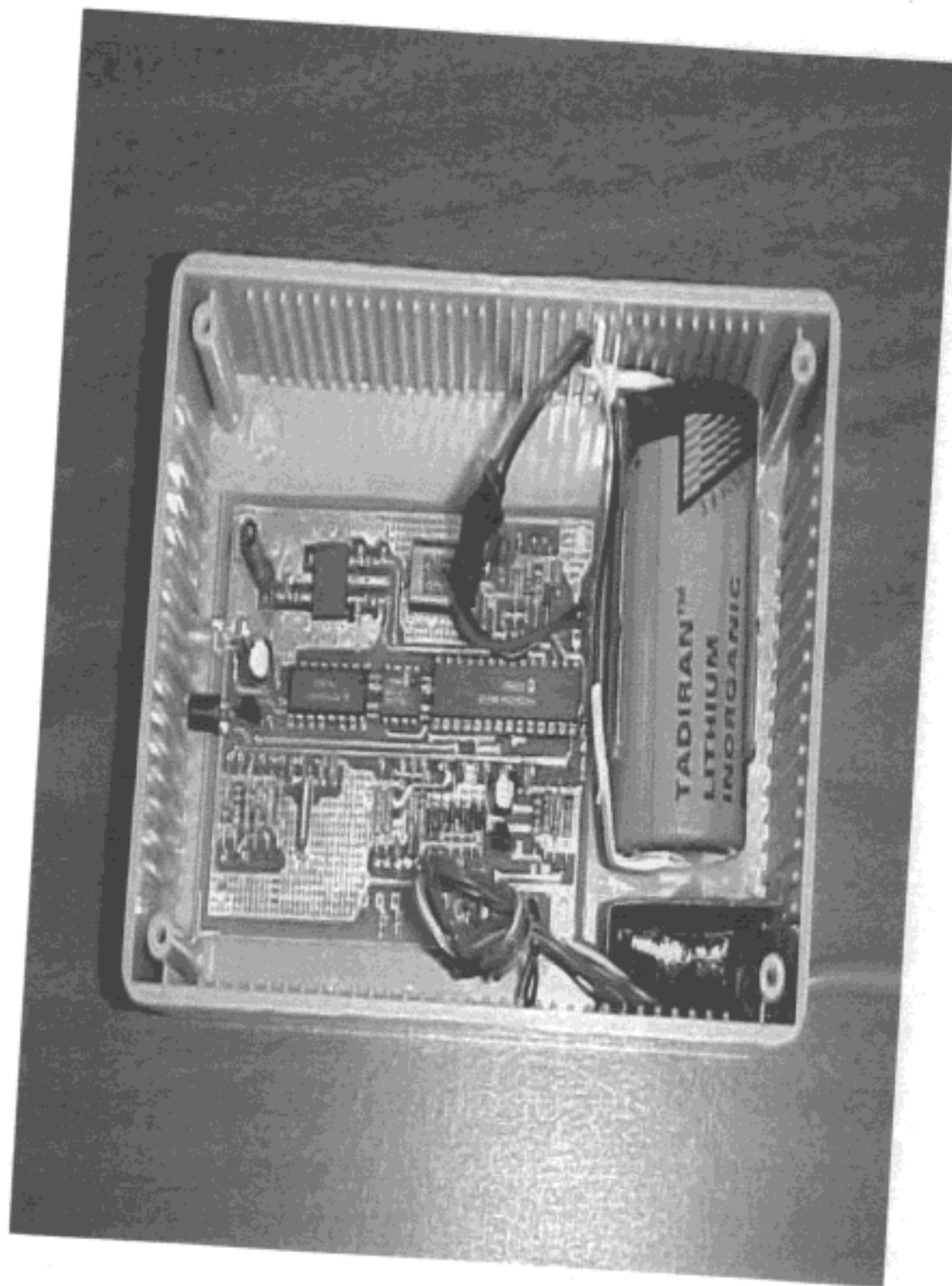
Figure 2 - Component Side of EUT
