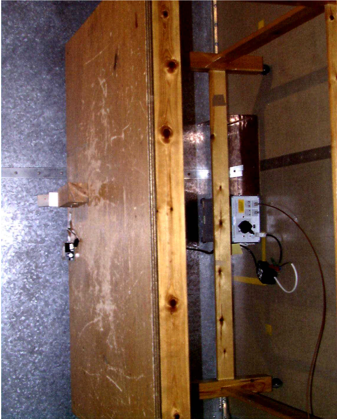
PHT/39126ETF03/001 Front view of conducted emissions.
