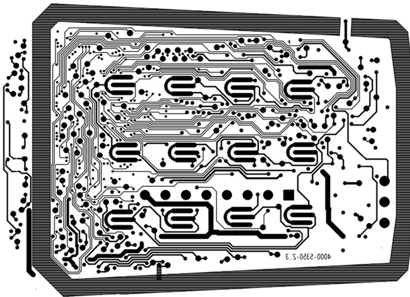
PCB layer 4, showing antenna bottom shield (figure 3):
