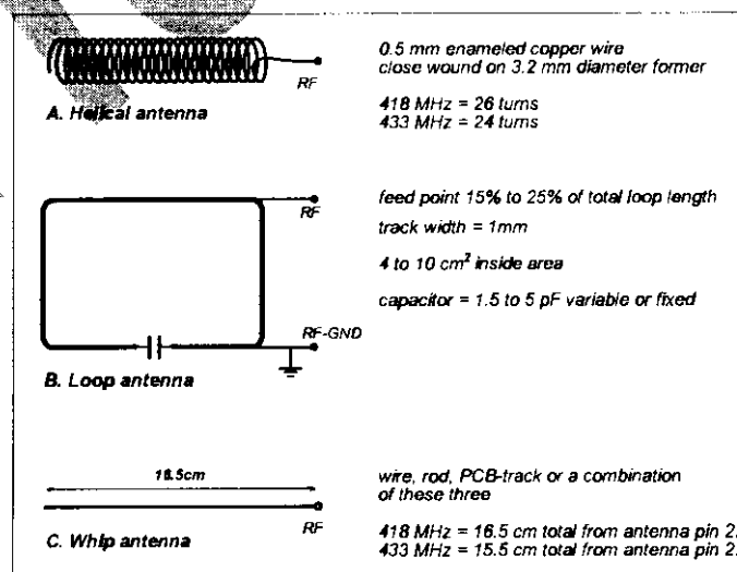
Fig.8: Antenna Configurations
