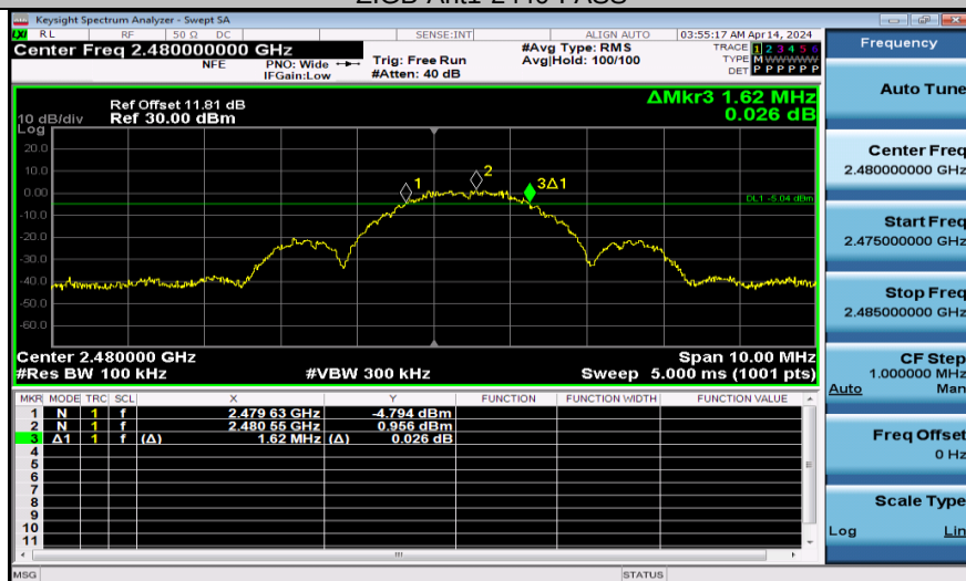
ZIGB-Ant1-2480-PASS
