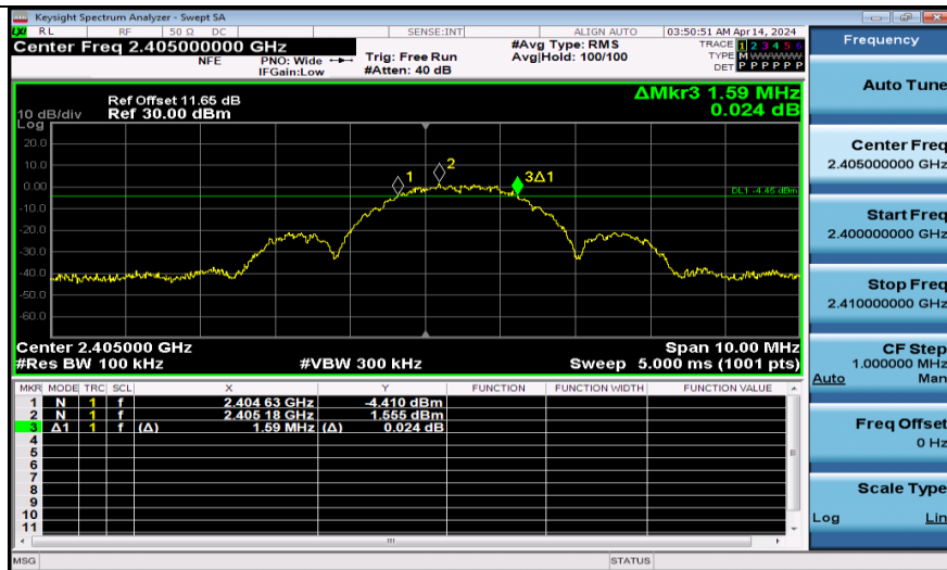
ZIGB-Ant1-2405-PASS
