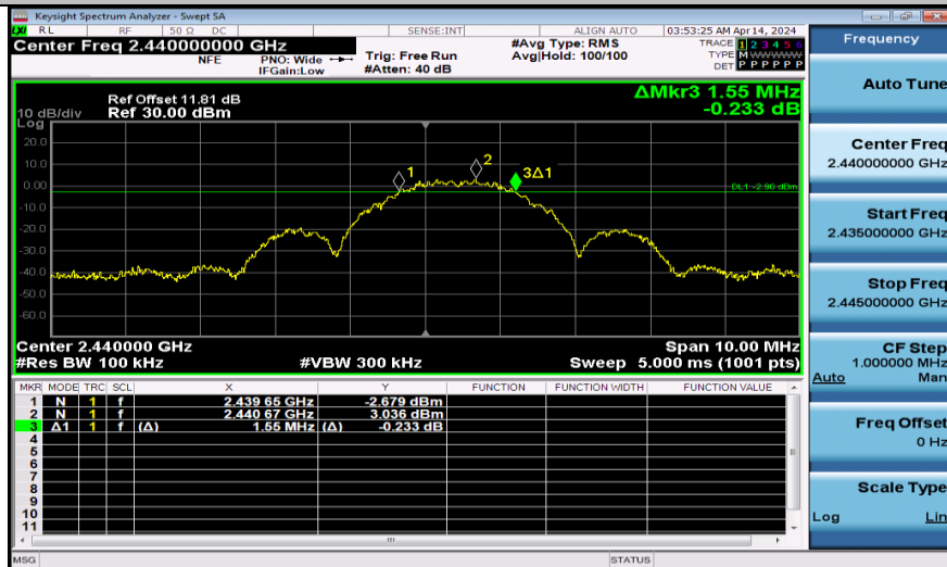
ZIGB-Ant1-2440-PASS
