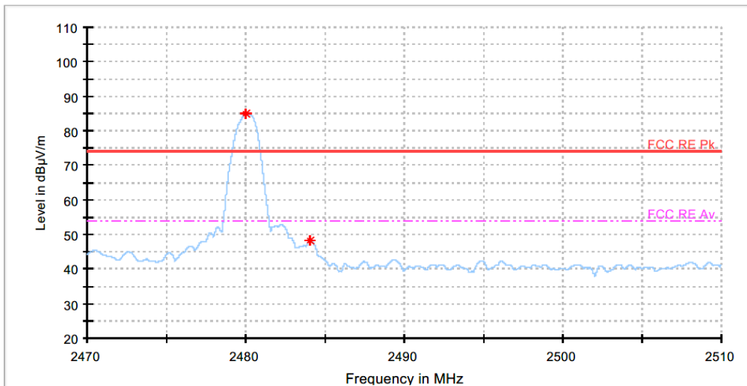
BLE 1Mbps, Highest Channel (2 480 MHz)_Peak
