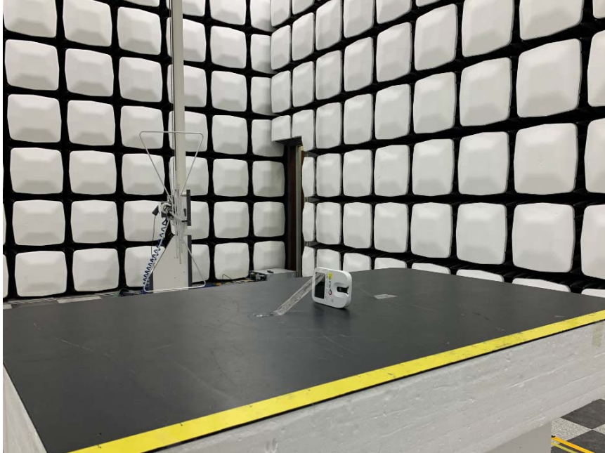
Radiated Test Picture(Front)_Below 1GHz
