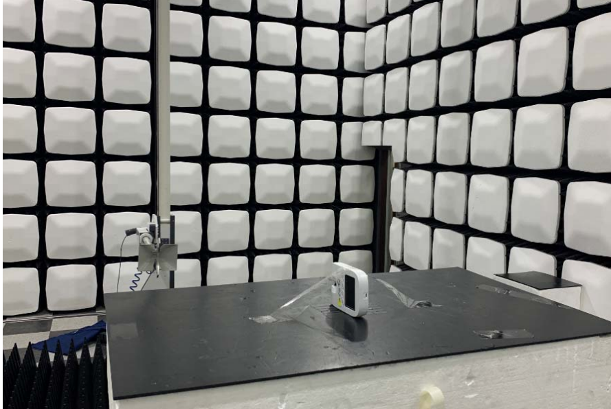
Radiated Test Picture(Front)_Above 1GHz
