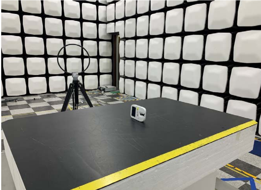
Radiated Test Picture(Front)_Below 30MHz
