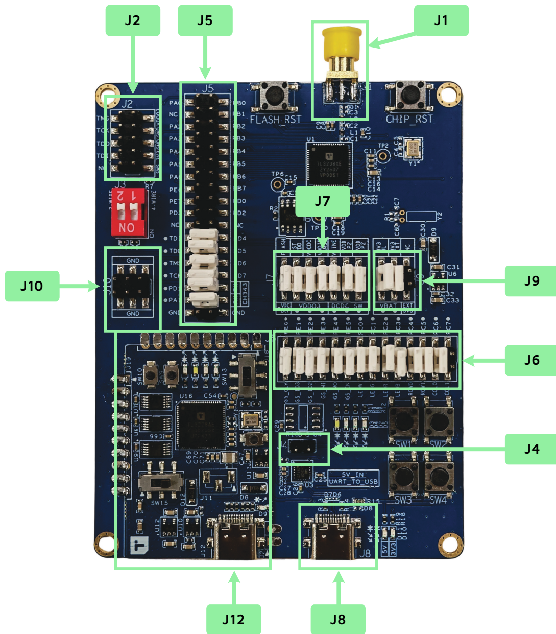
Figure 1-4 Connectors on Board Top
